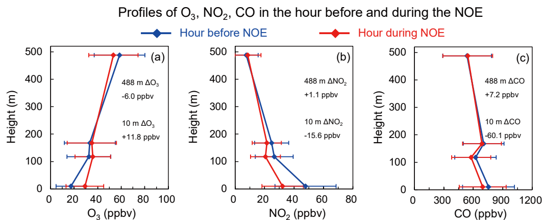
Figure 10. Characteristics of ozone, NO 2 , CO profiles before (blue colored lines) and during (red colored lines) the occurrence of the NOE event. ΔO 3 , ΔNO 2 , and ΔCO represent the change of concentrations during the occurrence of the NOE event compared to the hour before the NOE event.
