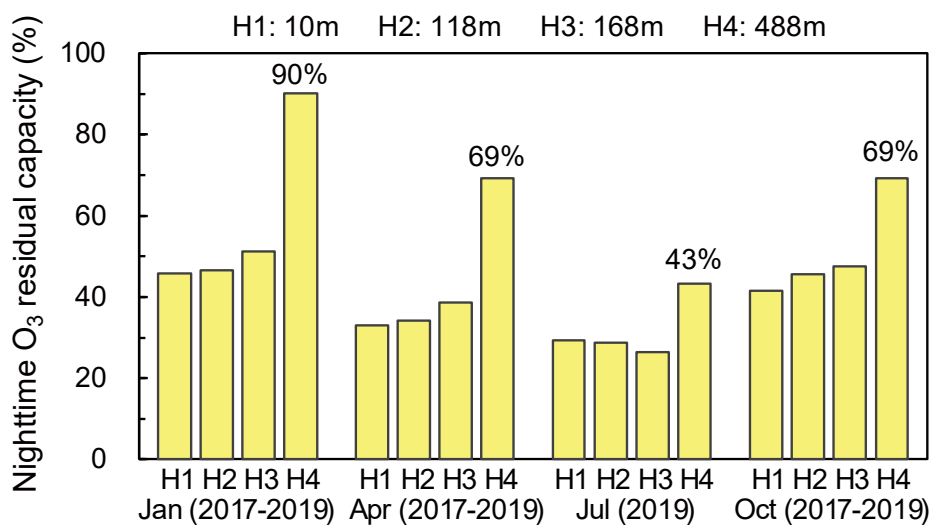
705 Figure 5. Nighttime ozone residual capacity at different height in the lower boundary layer in four seasons obtained from the Canton Tower measurements, 2017-2019. The nighttime ozone residual capacity is defined as the ratio of the ozone concentrations averaged over nighttime (20:00-07:00 LT) to that averaged over afternoon (14:00-17:00 LT).
