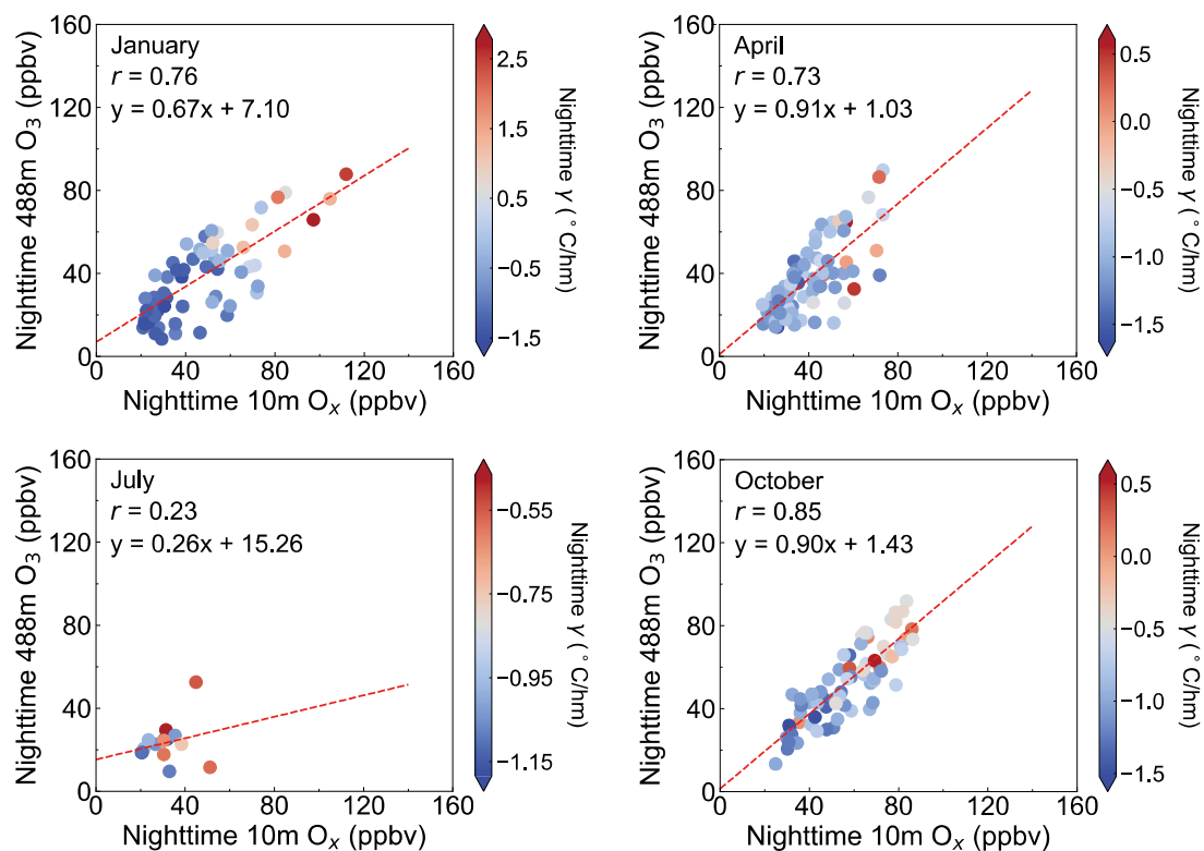
720 Figure 8. Relationship between nighttime (20:00-07:00 LT) 488 m ozone concentrations and nighttime surface O x (O x = O 3 + NO 2 ) concentrations. r represents correlation coefficient between the two variables. The red dash line and the fitting formula are fit from the two variables by a first-order polynomial. The fill color represents the temperature lapse rate averaged over nighttime.
