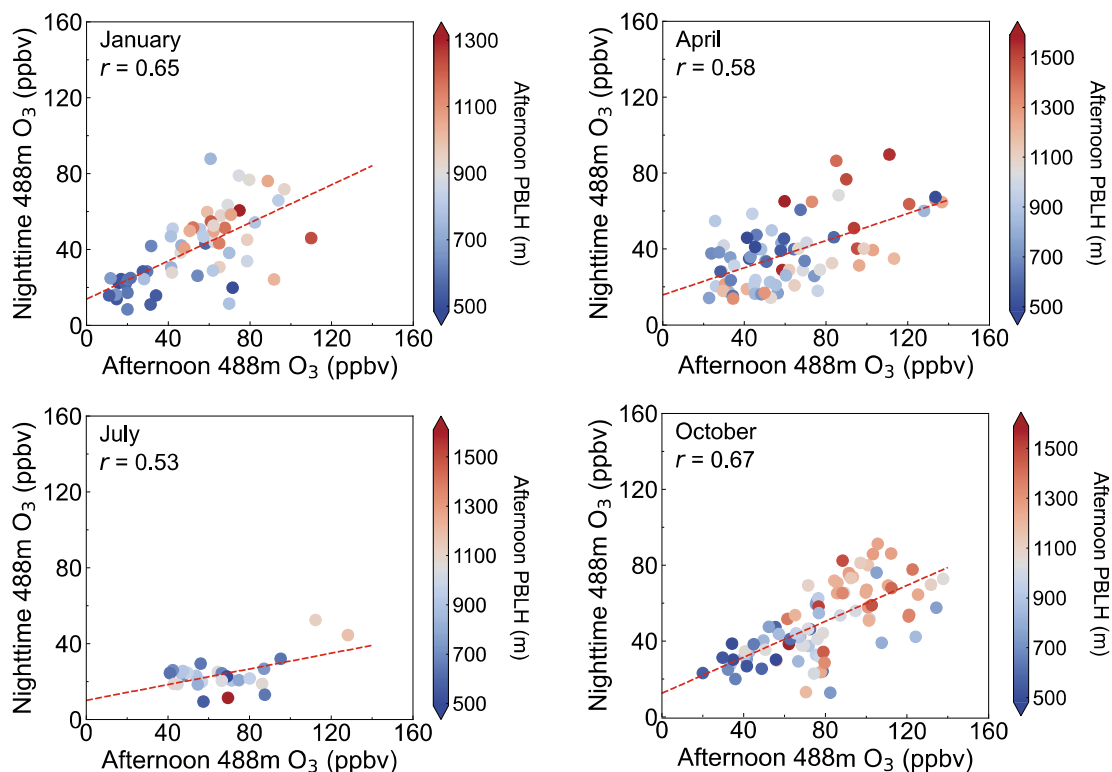
710 Figure 6. Dependence of nighttime (20:00-07:00 LT) 488 m ozone concentrations on afternoon (14:00-17:00 LT) 488 m ozone concentrations. r represents correlation coefficient between the two variables. The red dash line is fit from the two variables by a first-order polynomial. The color represents the planet boundary layer height (PBLH) obtained from the ERA5 reanalysis data averaged over afternoon.
