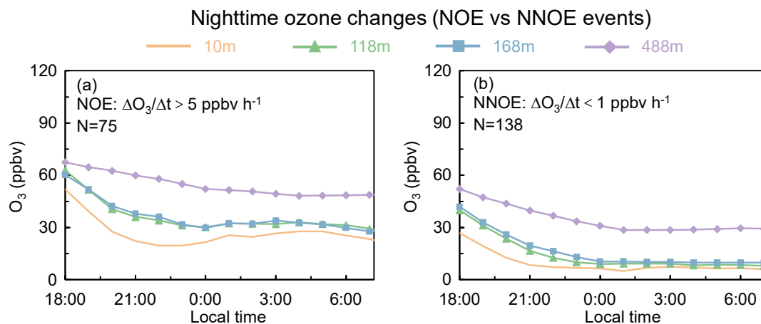
725 Figure 9. Comparison of ozone time series between the nighttime ozone enhancement (NOE, maximum of \Delta O_3/\Delta t > 5 \text{ ppbv h}^{-1} ) and the non-enhanced nocturnal ozone (NNOE, maximum of \Delta O_3/\Delta t < 1 \text{ ppbv h}^{-1} ) events. Panels (a) and (b) show the nighttime ozone changes averaged over 75 NOE and 138 NNOE events in 2017-2019 with available observations, respectively.
