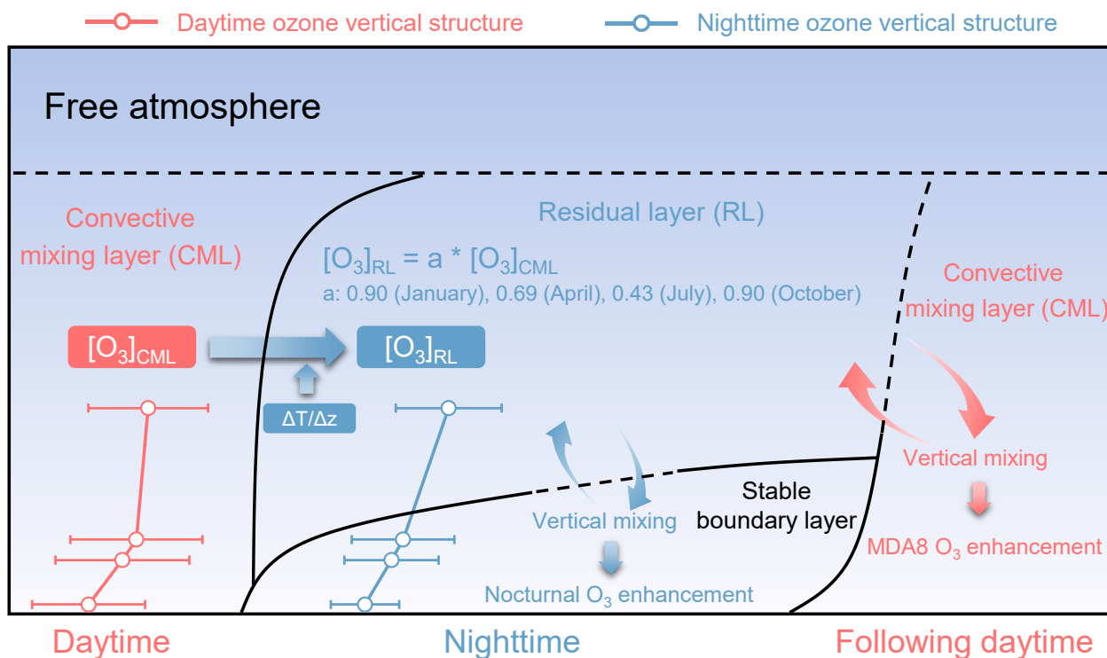
Figure 15. Conceptual model of the nighttime ozone in the lower boundary layer and its influences on surface ozone. The ozone profiles and the residual capacity (a) are obtained from the measurements in 2017-2019.
