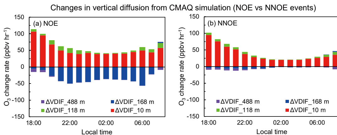
Figure 11. Characteristics of vertical diffusion ( \Delta VDF) during NOE and NNOE events at the four measurement heights at the Canton Tower. The budget terms of \Delta VDF are diagnosed from the CMAQ IPR module budget at the Canton Tower,
