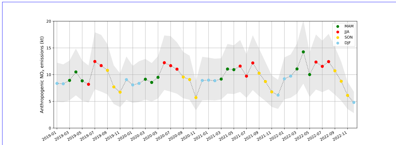
Figure 10: Total TROPOMI-derived anthropogenic \text{NO}_x emissions in Qatar from 2019 to 2022 2022 using the flux-divergence method. The colors are used to illustrate seasonal variations (green: MAM; red: JJA; yellow: SON; blue: DJF).
