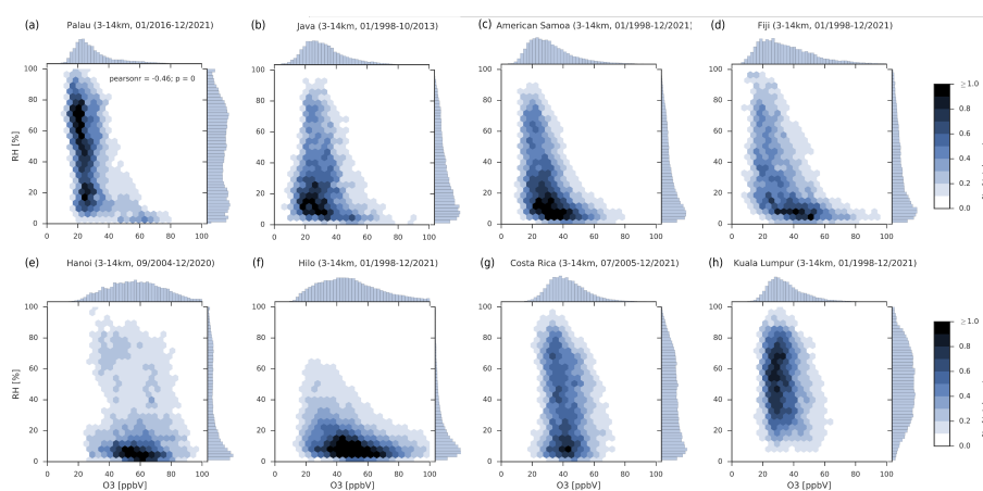
Figure 7. Free-tropospheric (3–14 km) relation between O_3 and RH in a 2D (hexagonally binned) histogram, normalized to the total count of data points per station, using all measured data pairs with \leq 100 ppb O_3 VMR for Palau (a) and selected SHADOZ stations (b–h); color shading indicates percentage of total count per gridpoint and marginal plots give individual 1D histograms, normalized to unity.
