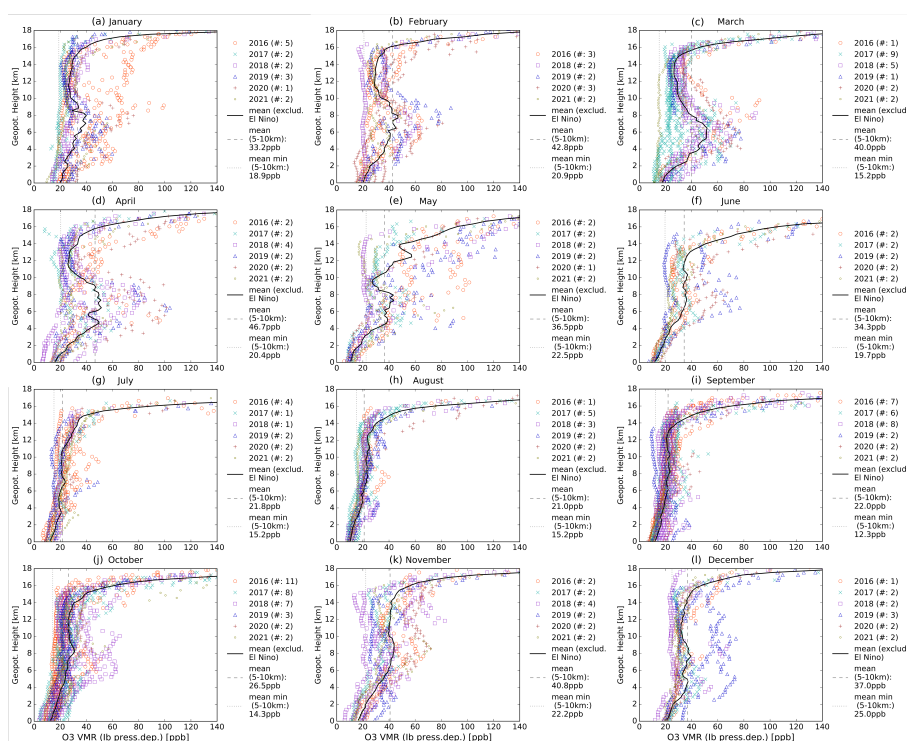
Figure A1. All measured individual O 3 VMR profiles sorted by month and year (colored markers), the monthly mean (solid black line) excluding El Niño 2016, i.e. starting 08/2016, and monthly statistics (dashed line for mean between 5 and 10 km, dotted line for mean of minimum values per sounding between 5 and 10 km); number (#) of profiles per year given in brackets.
