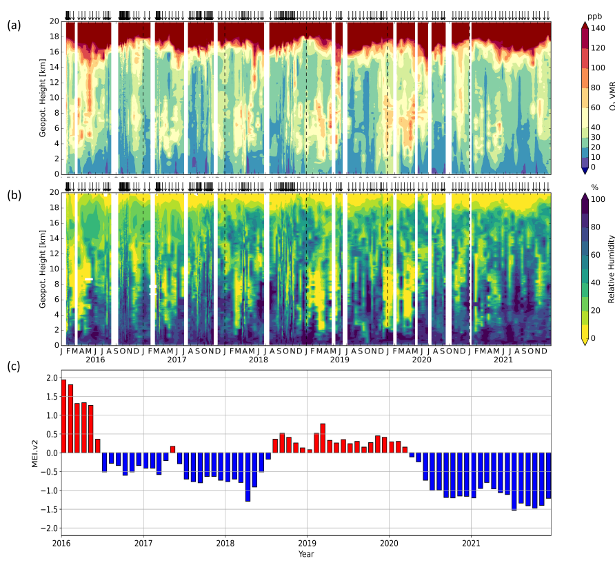
Figure 4. Time height cross sections of (a) ozone ( O_3 ) volume mixing ratio and (b) relative humidity (RH), (c) Multivariate ENSO index (MEI) from 2016 to 2021. The O_3 and RH measurements have been performed at the PAO. The ENSO Index data is provided by NOAA ( https://psl.noaa.gov/enso/mei/ ), (Wolter and Timlin, 2011).
