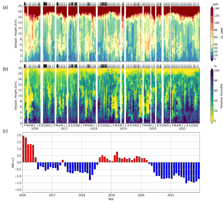
Figure 4. Time height cross sections of (a) ozone ( O_3 ) volume mixing ratio and (b) relative humidity (RH) ( with respect to liquid water ), (c) Multivariate ENSO index (MEI) from 2016 to 2021. The O_3 and RH measurements have been performed at the PAO. The ENSO Index data is provided by NOAA ( https://psl.noaa.gov/enso/mei ), (Wolter and Timlin, 2011).
