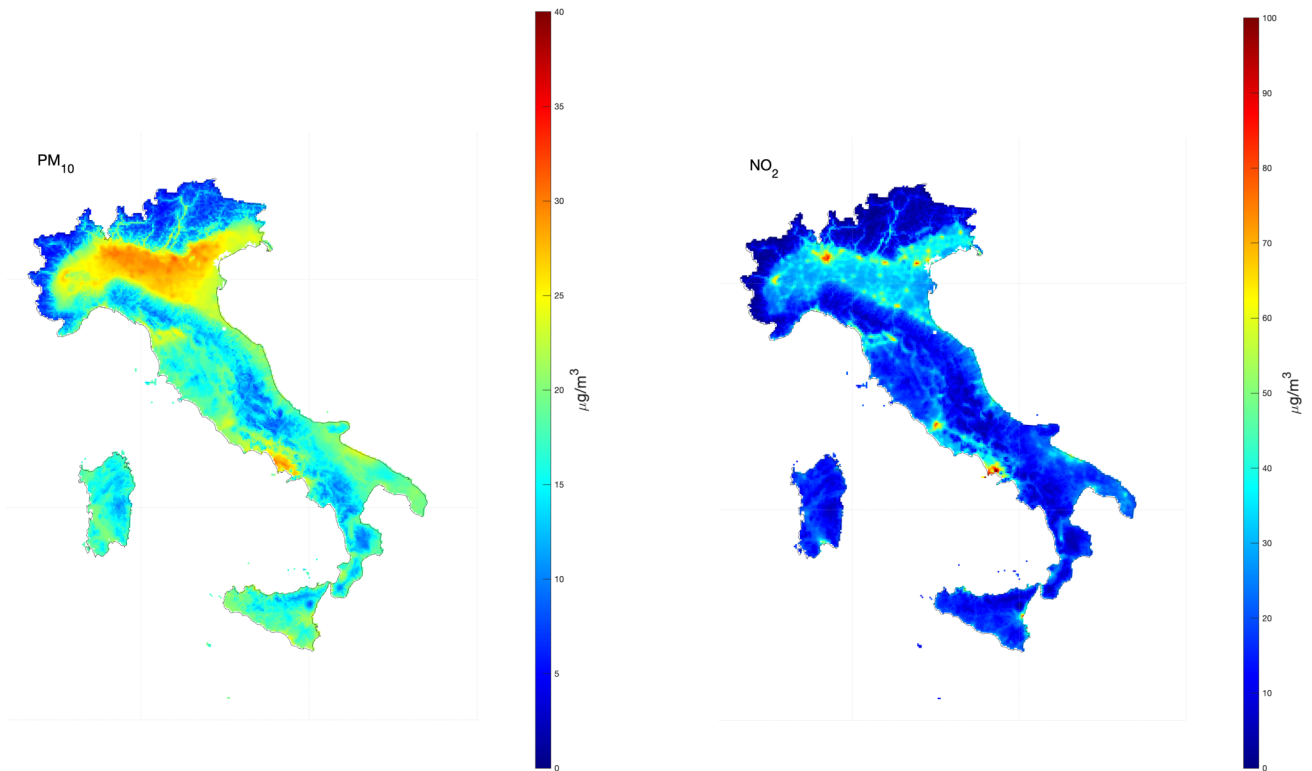
Figure 7. Median \text{PM}_{10} concentration map (left) of daily means, and median \text{NO}_2 concentration map (right) of 1-hour daily maximum in 2022, after the application of the second post-processing stage and estimated over a regular 4 \times 4 km grid resolution.
