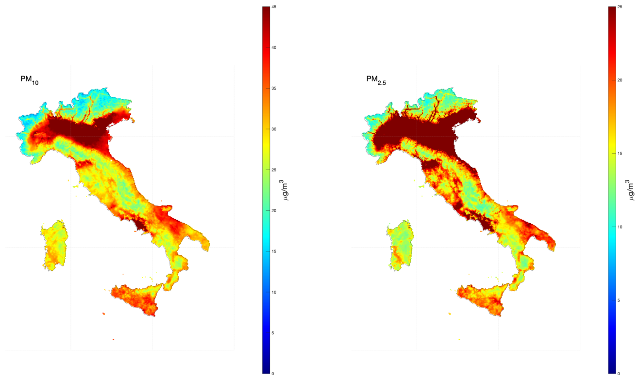
Figure 8. 95.1st percentile of PM_{10} (left) and PM_{2.5} (right) after the application of the second post-processing stage and estimated over a regular 4 \times 4 km grid resolution.
