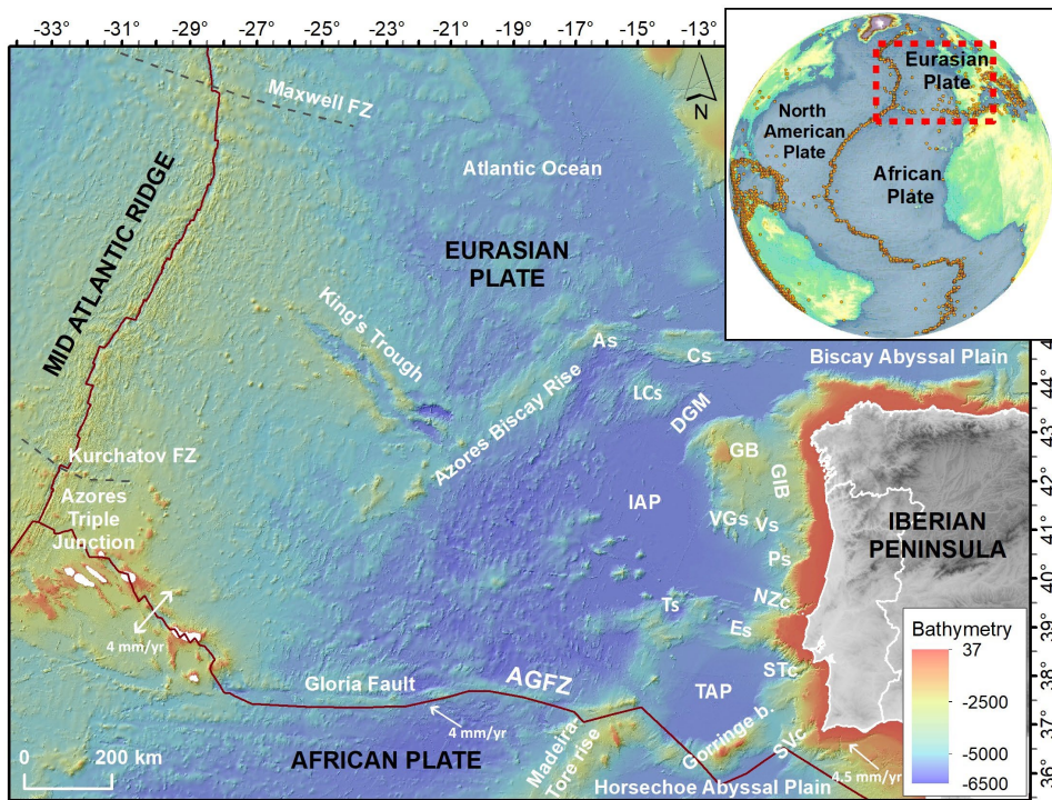
Figure 1: Study area. The WIM and its main physiographic features including their West (mid Atlantic ridge (MAR) , Eurasia- America) and South (Azores-Gibraltar fault zone AGFZ, Eurasia-Africa) plate boundaries. GB: Galicia Bank, IAP: Iberian Abyssal Plain, GIB: Galician interior Basin, VGs: Vasco de Gama seamount, Vs: Vigo seamount, Ps: Porto seamount, NZc: Nazare canyon, Es: Extremadura Spur, STc: Setubal canyon, TAP: Tagus abyssal plane, SVc: San Vicente canyon, FZ: fracture Zone (Kurtachov). Cs: Charcot seamount, As: Atlantic seamount.
