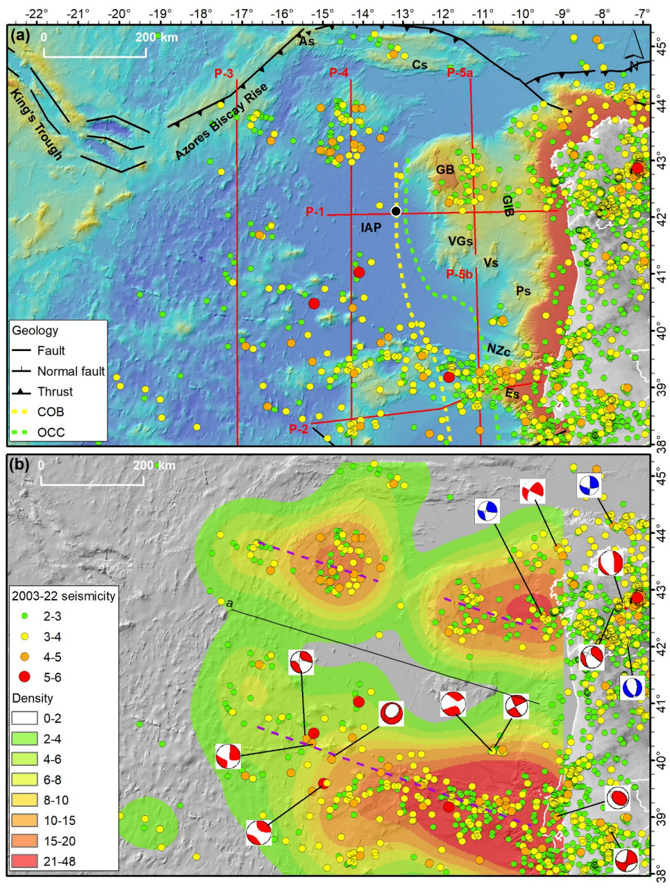
835 Figure 2. a) Seismicity studied in this work showing the events according to magnitude. b) Density map of events studied in this work highlighting the alignments in purple discontinuous lines 1) Galicia, north and 2), Lisbon, south (see text) some focal mechanisms are shown. Seismicity catalogue in the WIM in the period 2003-2022 (magnitude > 2.5, RMS < 1, Smaj < 25, Smin < 25 and Err < 75), according to the parameters described in the methodology section. Topographic base from EMODnet 840 Bathymetry Consortium (2020). Focal mechanism from CMT (blue) Catalog and IGN (red) Seismic Moment Tensor Database.
