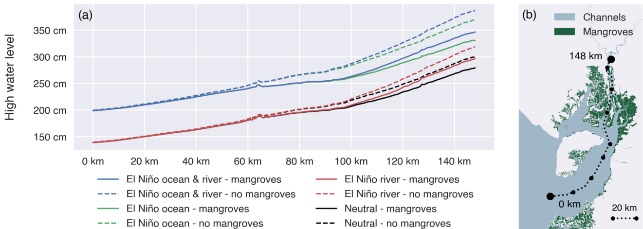
Figure 4. Maximum High water levels (a) during the simulated spring tides over a transect (b) running from the seaward boundary of the Gulf of Guayaquil through the eastern main branch of the Guayas river, receiving direct river discharge, for four scenarios, each one simulated with and without mangroves: a scenario with El Niño ocean and riverine forcing, with only El Niño oceanic forcing, with only El Niño riverine forcing and with neutral conditions (without El Niño forcing) at both sea- and landward boundaries.
