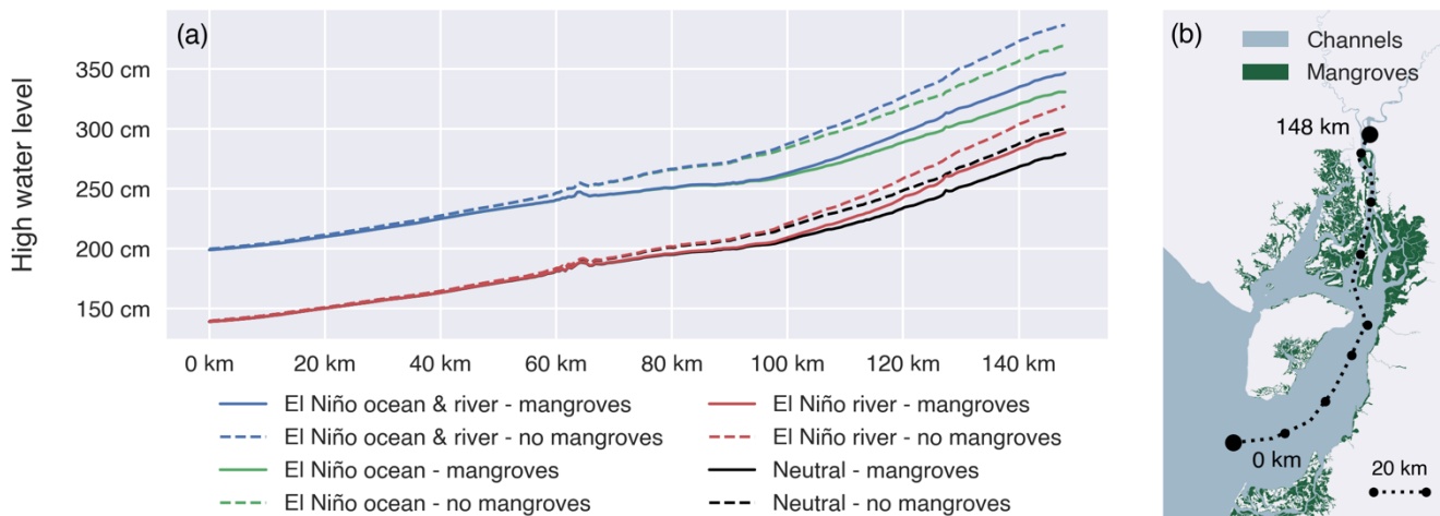
245 Figure 4. Maximum High water levels (a) during the simulated spring tides over a transect (b) running from the seaward boundary of the Gulf of Guayaquil through the eastern main branch of the Guayas river, receiving direct river discharge, for four scenarios, each one simulated with and without mangroves: a scenario with El Niño ocean and riverine forcing, with only El Niño oceanic forcing, with only El Niño riverine forcing and with neutral conditions (without El Niño forcing) at both sea- and landward boundaries.
