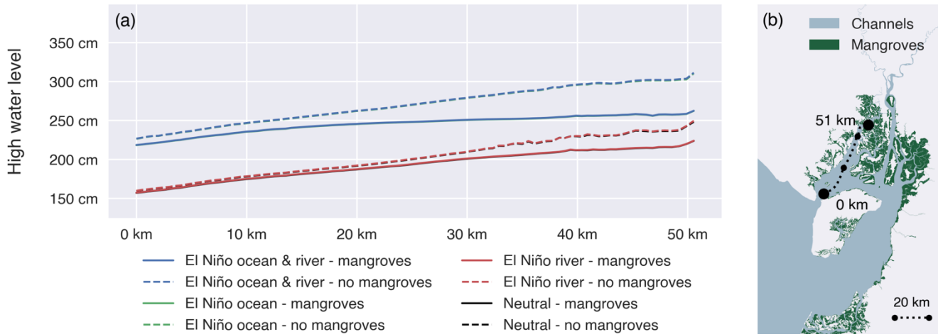
Figure A1. High water levels (a) during the simulated spring tide over a transect running from the northern entrance of the delta through the western main branch of the Guayas delta, receiving no river discharge (b), for four scenarios, each one simulated with and without mangroves: a scenario with increased ocean water levels and increased river discharge, with only increased ocean water levels, with only increased discharge and with neutral conditions at both sea- and landward boundaries. Note that differences between both El Niño ocean & river scenarios and El Niño ocean scenarios are negligible, and differences between both El Niño river scenarios and Neutral scenarios are negligible.
