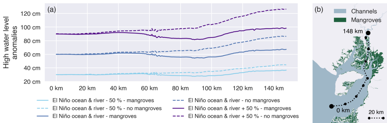
265 Figure 6. High water level anomalies (a) during the simulated spring tide over a transect (b) running from the seaward boundary of the Gulf of Guayaquil through the eastern main branch of the Guayas river, receiving direct river discharge, for three scenarios,
