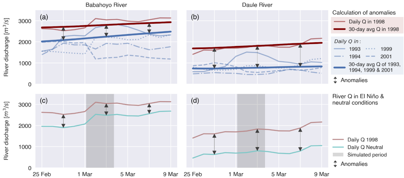
190 Figure 3. Calculation of river discharge (Q) anomalies from observed daily time series (a, b) and model input for daily river discharges for the El Niño & neutral scenarios (c, d) for the Babahoyo (a, c) and Daule rivers (b, d). The thick red line is a 30-day moving average of the daily river discharge time series observed during El Niño conditions in 1998 (thin red line). The thick blue line shows a 30-day moving average of the daily river discharge time series observed during neutral conditions in 1993, 1994, 1999 and 2001 (closest 4 years to 1998 without El Niño or La Niña events). River discharge anomalies are calculated as the difference between both 30-day moving means (a, b). Daily neutral river discharge values, as imposed at the upstream model boundaries, are calculated by subtracting the anomalies from the daily river discharges of 1998 (c, d).
