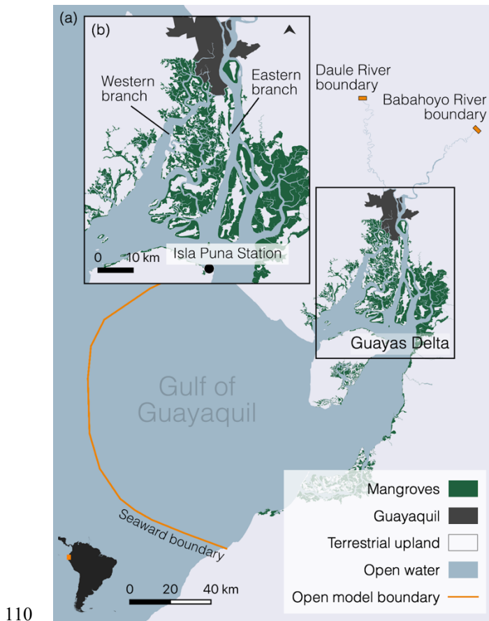
Figure 1. Map of the model domain (a), covering the Gulf of Guayaquil and the Guayas delta (b). The computational domain includes both the open water (in blue) and the mangrove areas (in green). The orange lines represent the open model boundaries: the seaward boundary downstream, and two freshwater boundaries upstream in the Daule and Babahoyo rivers.
