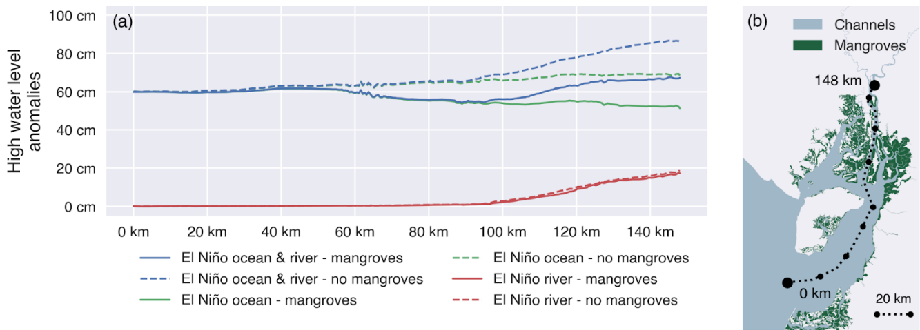
255 Figure 5. High water level anomalies (a) during the simulated spring tide over a transect (b) running from the seaward boundary of the Gulf of Guayaquil through the eastern main branch of the Guayas river, receiving direct river discharge, for three scenarios, each one simulated with and without mangroves: a scenario with El Niño ocean and riverine forcing, with only El Niño oceanic forcing and with only El Niño riverine forcing. High water level anomalies are defined as the difference between each model scenario and the corresponding Neutral model scenario (without El Niño forcing).
