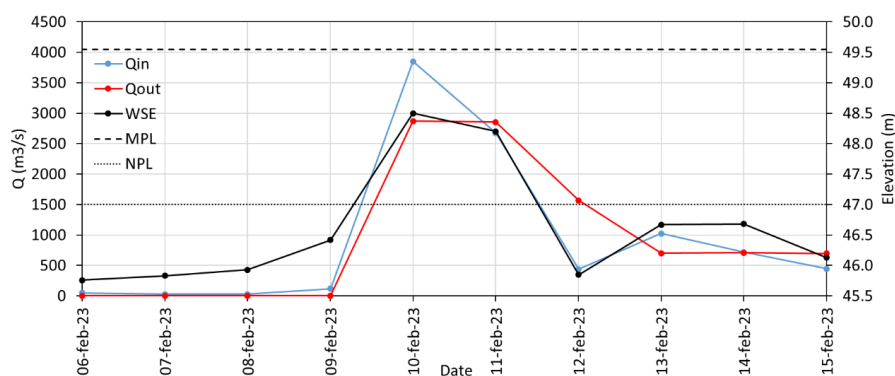
275 Figure 7. Daily inflow (Q in ), daily outflow (Q out ), and water surface elevation (WSE) in the PL reservoir during the flood event. The Normal and Maximum Pool Levels (NPL and MPL) are also provided for reference. Daily discharges correspond to the average over the previous 24 hours.
