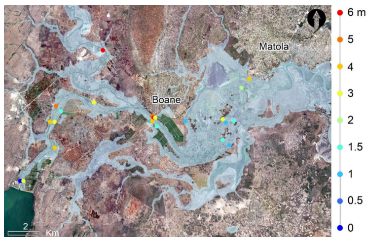
285 Figure 8: Location of the points at which the maximum water depth during the flood was estimated from field observations of the marks left by the water. Background image © Google Earth V 7.3.6.9345, http://www.earth.google.com [13 April 2023].
