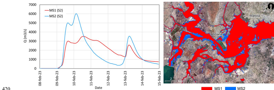
Figure 13: Hydrograph arriving at Boane (left) and flood extent in the AOI, under the scenarios MS1 (actual management of the reservoir during the flood event) and MS2 (absence of PL reservoir). Background image © Google Earth V 7.3.6.9345, http://www.earth.google.com [13 April 2023].
