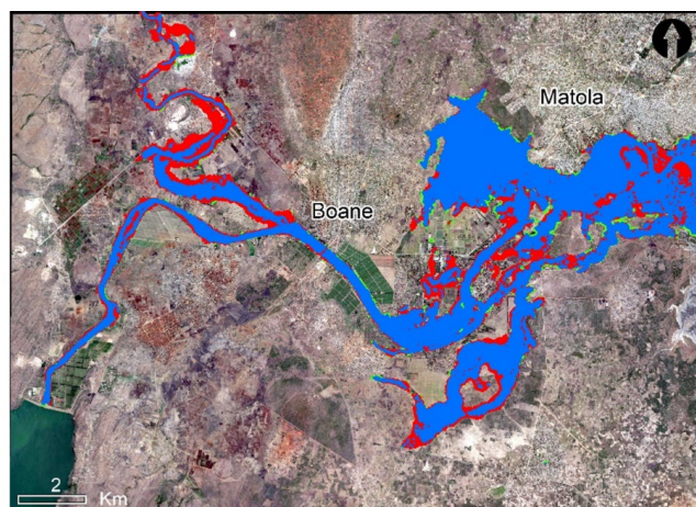
■ Overlap ■ MS1: Modelled with Iber ■ Observed SNAP processed
