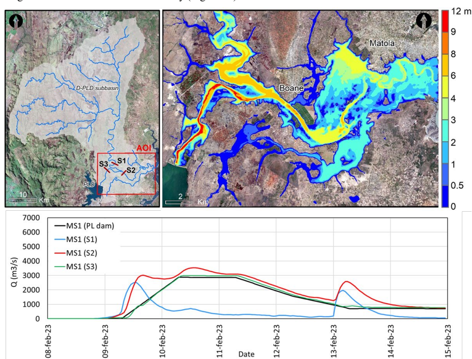
Figure 10: Map of maximum water depth in the area of interest (AOI) and hydrographs computed with Iber at several cross-sections located around the confluence of the rivers Umbeluzi and Moveve for the scenario MS1. Background images © Google Earth V 7.3.6.9345, http://www.earth.google.com [13 April 2023].
