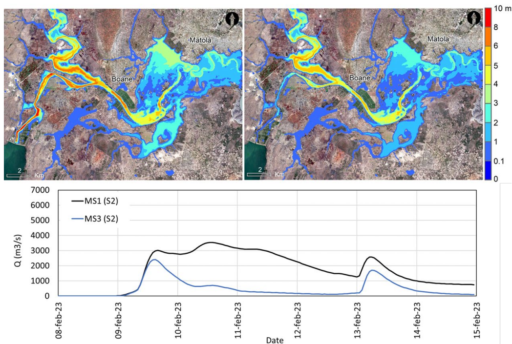
435 Figure 14: Water depth maps computed under the scenarios MS1 (left) and MS3 (right). The hydrographs computed in cross-section S2 for both scenarios are also shown. Background images © Google Earth V 7.3.6.9345, http://www.earth.google.com [13 April 2023].
