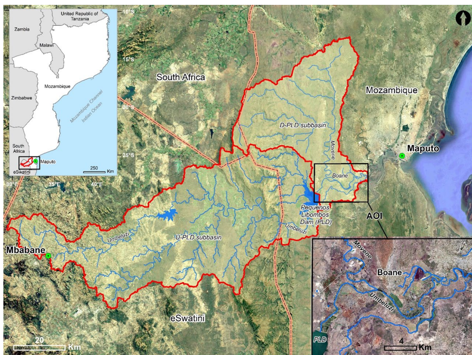
105 Figure 1: Location map of the Umbeluzi catchment, divided in two subbasins, U-PLD and D-PLD, located respectively upstream and downstream of the PL dam, and definition of the Area of Interest (AOI) for this study. Background image © Google Earth V 7.3.6.9345, http://www.earth.google.com [13 April 2023].
