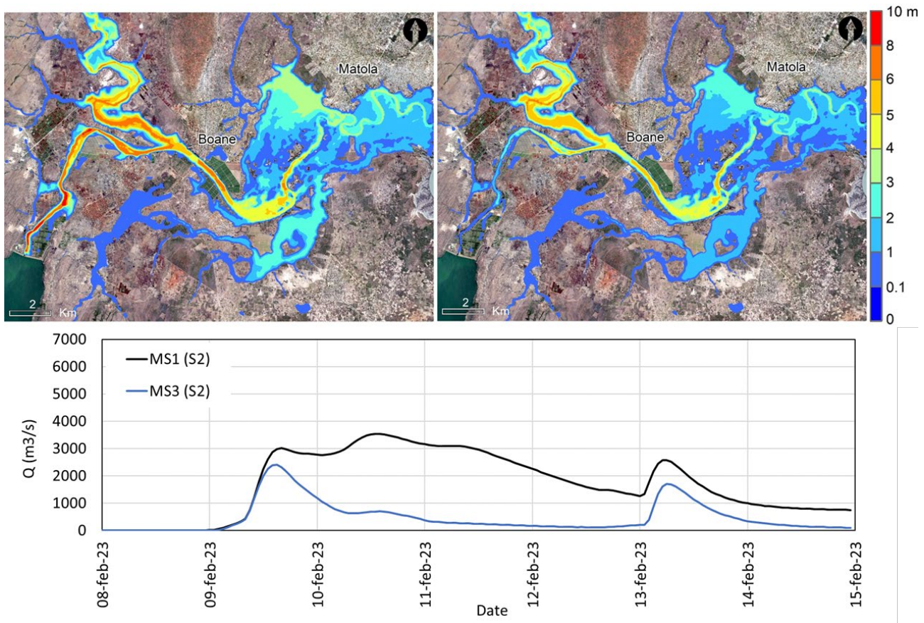
475 Figure 14: Water depth maps computed under the scenarios MS1 (left) and MS3 (right). The hydrographs computed in cross- section S2 for both scenarios are also shown. Background images © Google Earth V 7.3.6.9345, http://www.earth.google.com [13 April 2023].
