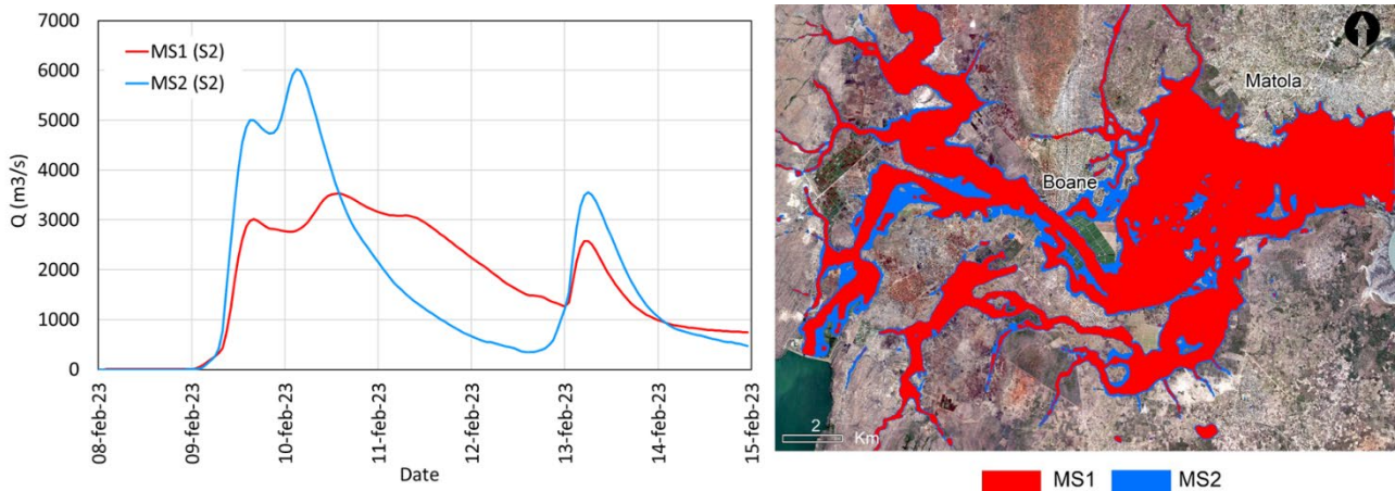
460 Figure 13: Hydrograph arriving at Boane (left) and flood extent in the AOI, under the scenarios MS1 (actual management of the reservoir during the flood event) and MS2 (absence of PL reservoir). Background image © Google Earth V 7.3.6.9345, http://www.earth.google.com [13 April 2023].
