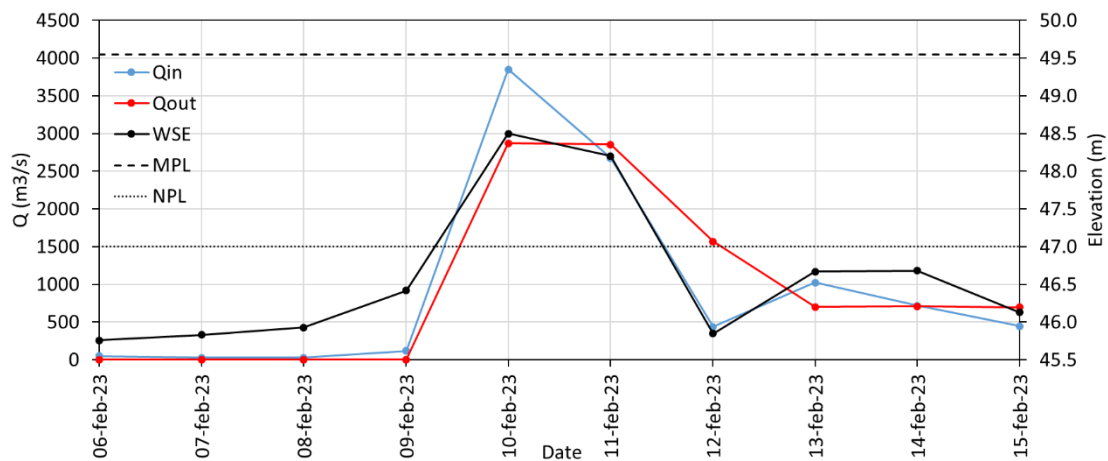
Figure 7. Daily inflow (Q in ), daily outflow (Q out ), and water surface elevation (WSE) in the PL reservoir during the flood event. The Normal and Maximum Pool Levels (NPL and MPL) are also provided for reference. Daily discharges correspond to the average over the previous 24 hours.
