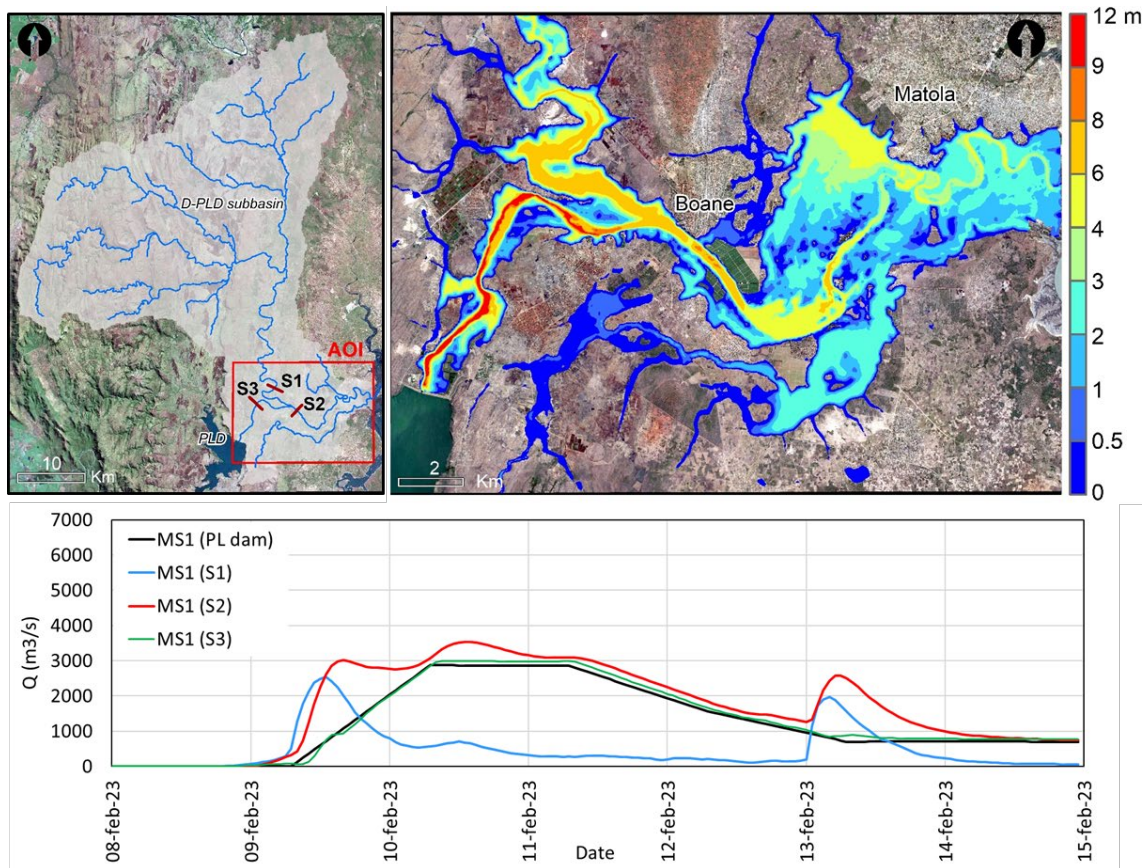
405 Figure 10: Extension of the D-PLD subbasin with its main river network and the location of cross section S1-S3 (top-left), map of maximum water depth in the AOI (top-right) and hydrographs computed with Iber at several cross-sections located around the confluence of the rivers Umbeluzi and Moveve for the scenario MS1. Background images © Google Earth V 7.3.6.9345, http://www.earth.google.com [13 April 2023].
