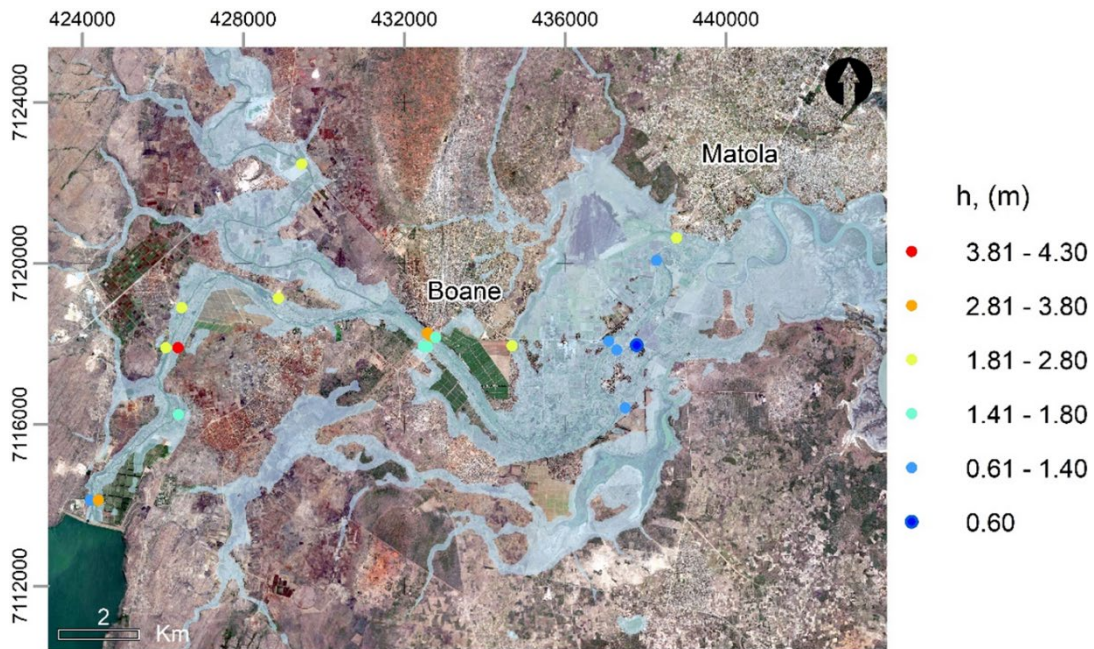
Figure 8: Location of the points at which the maximum water depth during the flood was estimated from field observations of the marks left by the water. The color of the dots indicates the maximum water depth estimated. The shaded area represents the maximum flood extent for the scenario MS1. Background image © Google Earth V 7.3.6.9345, http://www.earth.google.com [13 April 2023].
