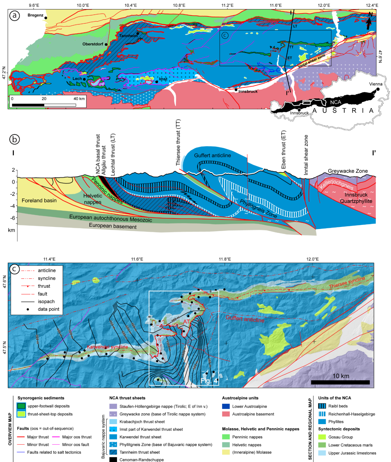
Figure 1: (a) Map showing the main tectonic units of W-Austria. Inset shows tectonic map showing the location of the Northern Calcareous Alps in western Austria. Rectangles show location of Figure Fig. 1c. Modified after Ortner and Kilian (2022). (b) N-S cross-section of the NCA at ~11.7°E, crossing the Achenal structure. (c) Geological map of the Achenal structure within the Karwendel thrust sheet. Black lines show isopachs of the Upper Jurassic Oberalm Fm, with data compiled from Nagel et al. (1976) and Schütz (1979). The hanging wall and footwall of the Achenal thrust (AT) were contoured separately, single outliers in the data were ignored. Major thickness changes occur from W to E and a maximum is observed in the southern hanging wall of the thrust. Rectangle shows the location of the study area (Fig. 4).
