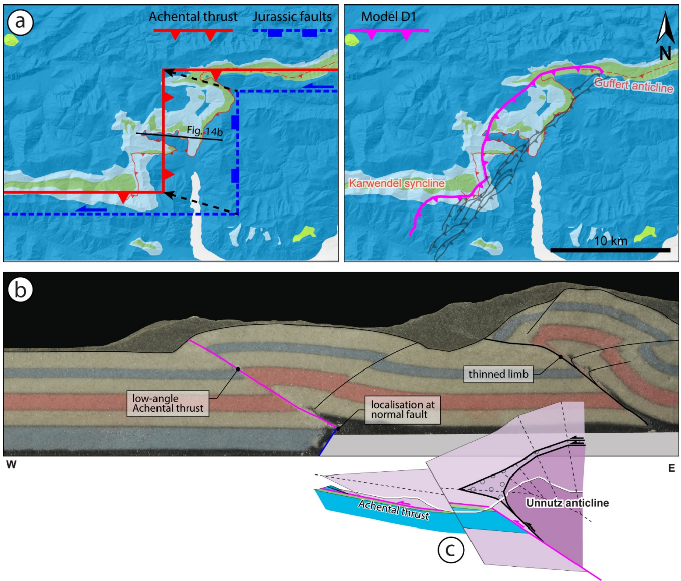
665 Figure 14: Summary figure showing (a) possible arrangement of Jurassic basin-bounding faults in relation to the Achenal thrust (left) and 670 overlay of inversion structures formed in analogue model D1, outlining the subsurface architecture (right). The traces of the thrusts in model D1 have not been intersected with the topography. Geological map modified after Ortner and Gruber (2011) and Ortner and Kilian (2016). For a legend of the geological map, see Fig. ure 1. (b) shows key structural elements in a cross-section of model D1 and (c) the corresponding 675 cross-section of the Unnutz anticline (see also Fig. ure 5a). The Achenal thrust is marked in pink. See Fig. ure 5 for legend of lithologies.
