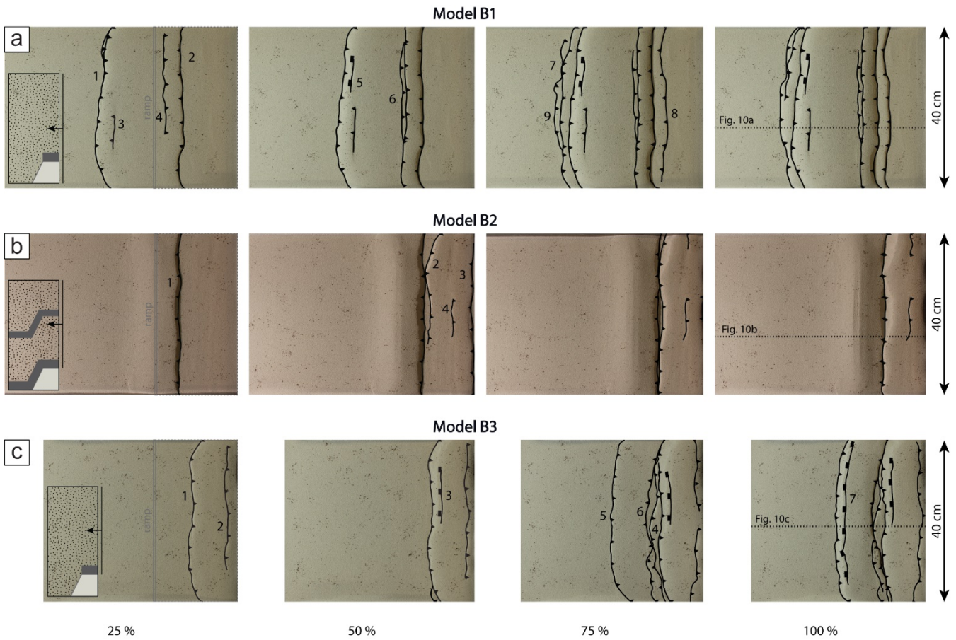
415 Figure 9: Top views of models (a) B1, (b) B2, and (c) B3 at 25, 50, 75 and 100 % of total shortening. Locations of sections are indicated (dotted lines). Numbers show sequence of fault formation. The insets in the first top view photographs show the modelling setups in cross- sectional view.
