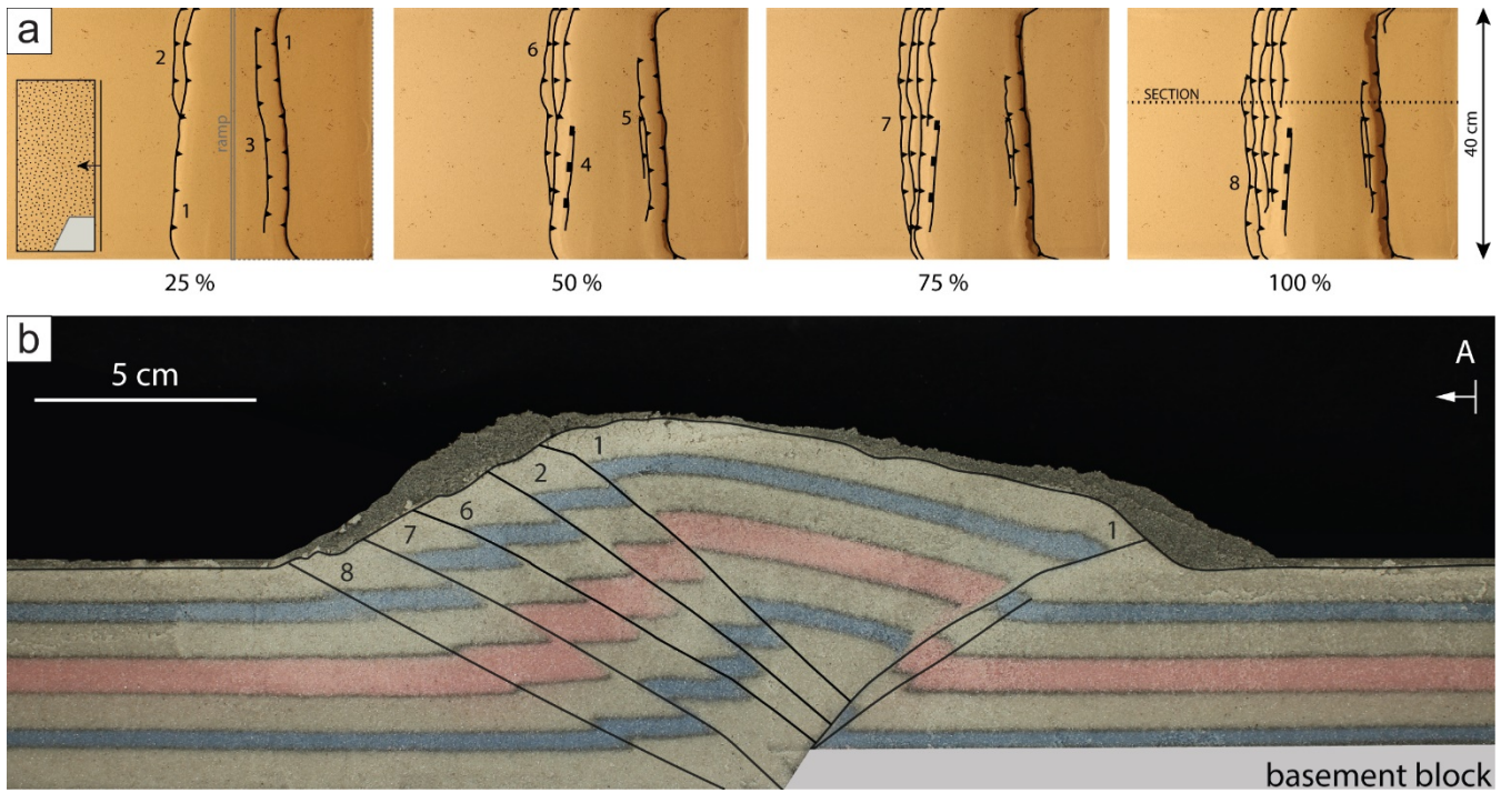
385 Figure 8: Modelling results of model A, showing (a) top views at 25, 50, 75 and 100 % of total shortening, and (b) side view at 100 % of total shortening. Location of section is marked in (a). Numbers show sequence of fault formation. The inset in the first top view photograph shows the modelling setup in cross-sectional view.
