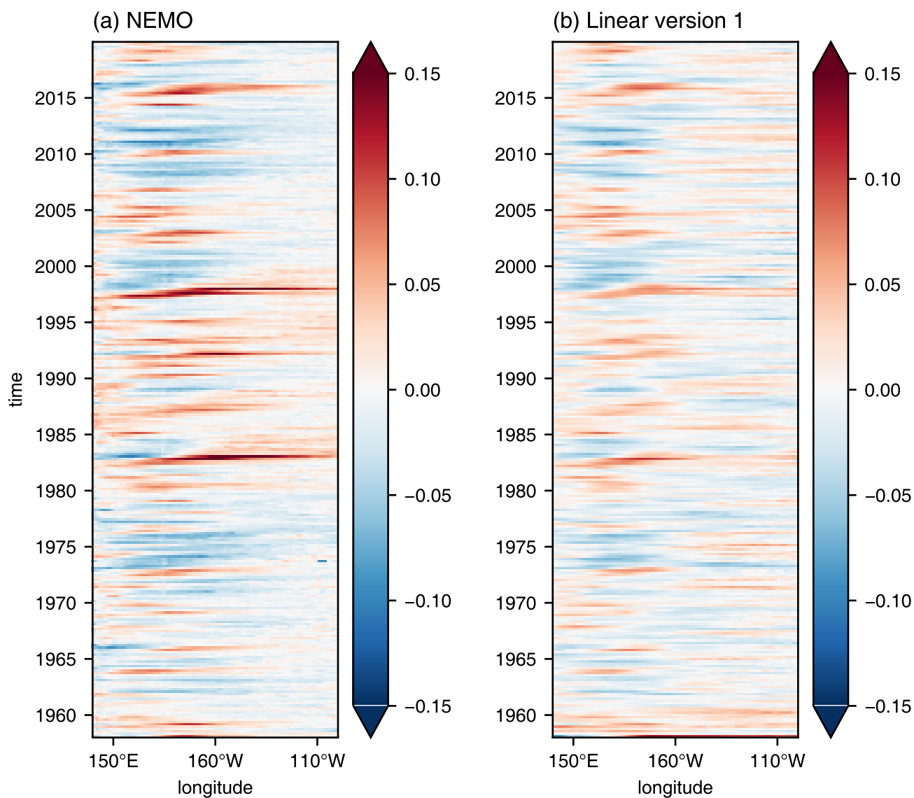
Figure 6. Hovmoeller diagrams as a function of longitude along the equator for (a) \eta_{mti} computed from the NEMO model simulation and (b) \eta_{mti} computed using version 1 of the linear multi-mode model. The units are metres.
