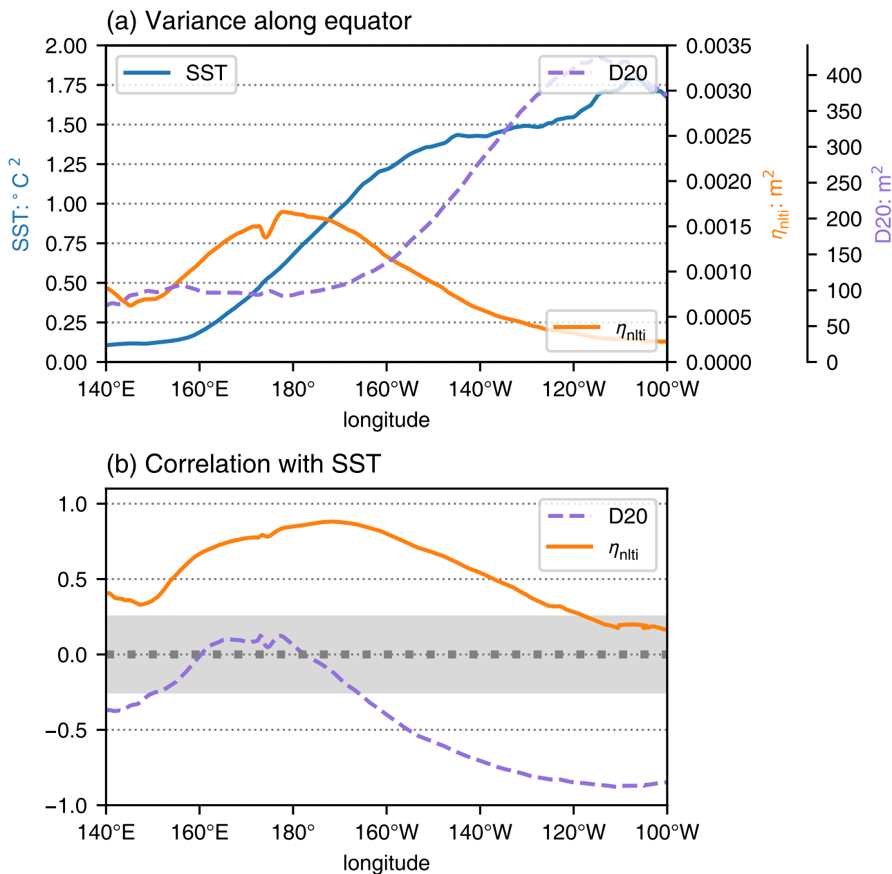
Figure 3. (a) The variance of detrended time series of monthly mean anomalies of SST (blue), \eta_{nlti} (orange), and D20 (dashed) as a function of longitude along the equator in the NEMO model simulation. (b) Same as (a) but for the correlation of the different indices with SST. The units in (a) are (^{\circ}\text{C})^2 (left hand scale) for SST; \text{m}^2 (right hand scale) for D20 and \eta_{nlti} . Correlations in (b) that are outside the grey, shaded region are significantly different from zero at the 95% level.
