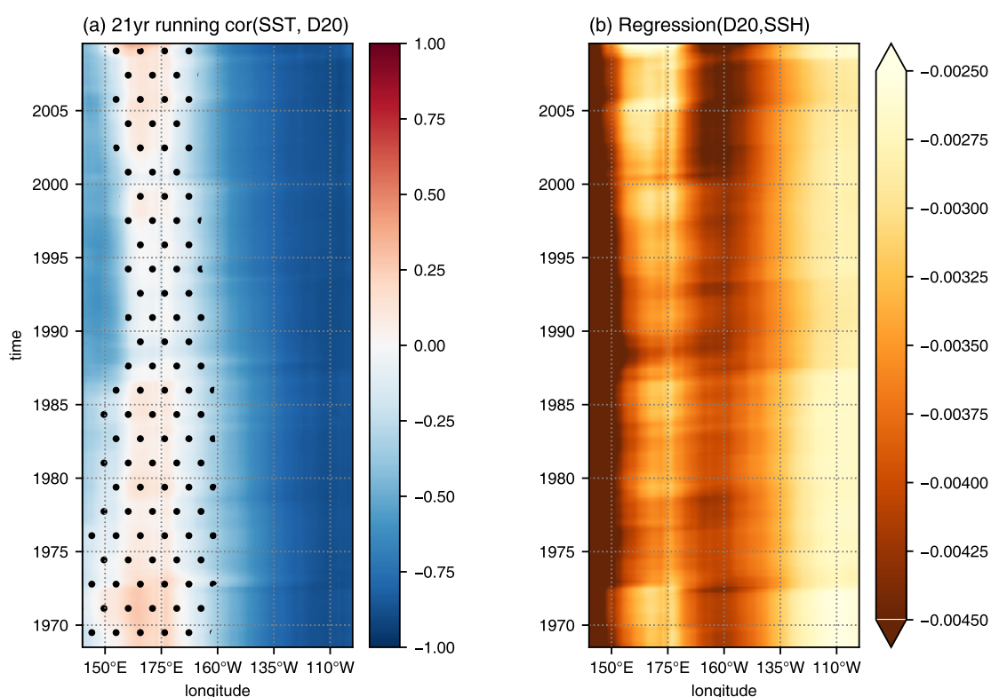
Figure 8. (a) The correlation in running 21 year windows between anomalies of SST and D20 from the NEMO model simulation. The time series have been detrended in each window separately. Dots indicate regions where the correlation is not significantly different from zero at the 95% level. (b) The coefficient, in running 21 year windows, obtained by regressing D20 on sea surface height from the NEMO model simulation. The time series have been detrended in each window separately. The regression slopes are everywhere significantly different from zero at the 95% level.
