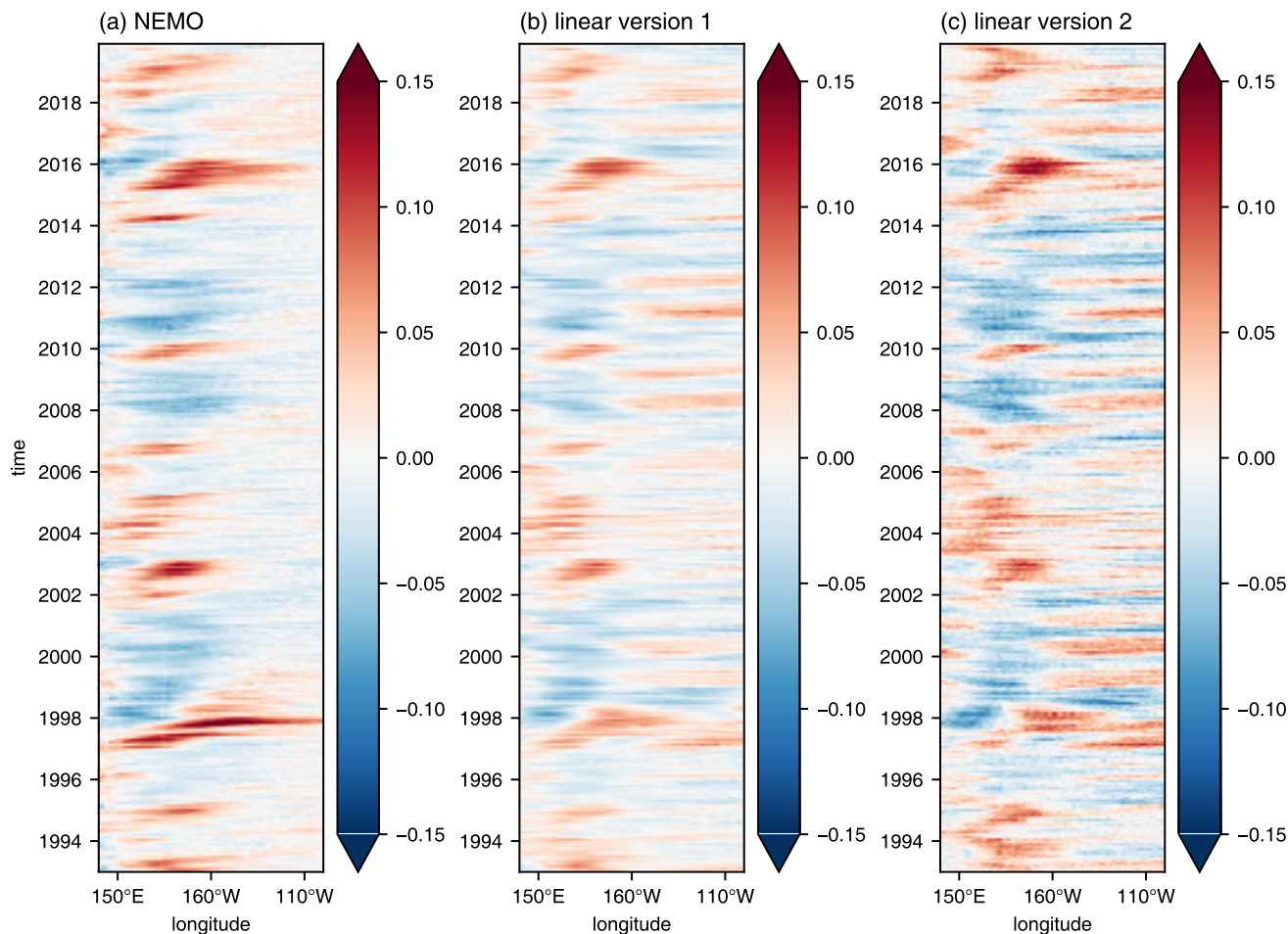
Figure 7. Hovmoeller diagrams (units of metres) along the equator of (a) \eta_{m\ell t i} computed from the NEMO model simulation, (b) \eta_{m\ell t i} computed using version 1 of the linear model using SSH from the NEMO model, and (c) \eta_{m\ell t i} computed using version 2 of the linear model using AVISO data.
