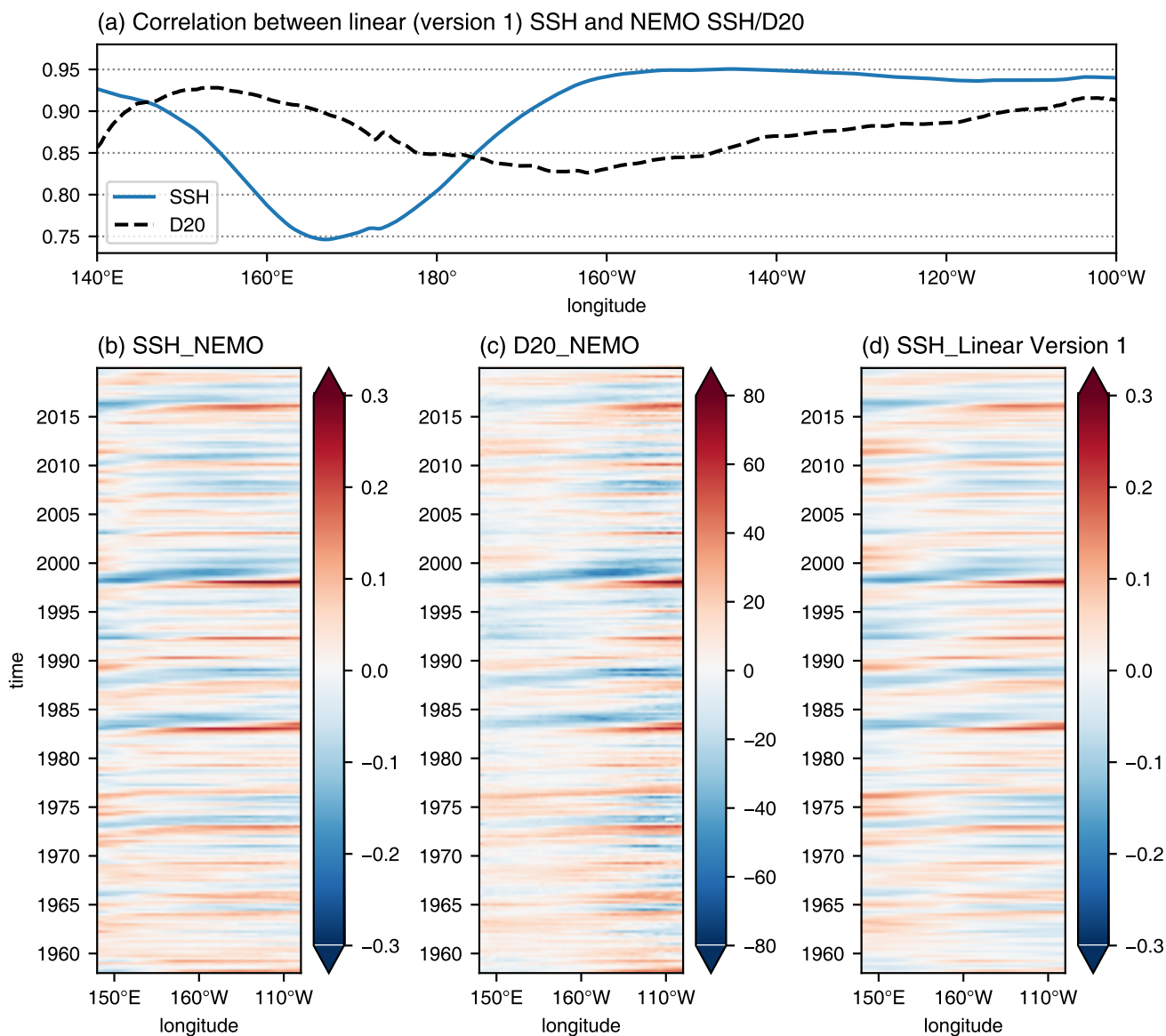
Figure 5. (a) The correlation between SSH from version 1 of the linear model and anomalies of SSH (blue) and D20 (sign reversed) from the NEMO model simulation (black dashed). All time series have been detrended and all the correlations shown are significantly different from zero at the 99% level. Also shown are Hovmoeller diagrams (units of metres) along the equator of anomalies of (b) SSH and (c) D20 from the NEMO model and (d) SSH from version 1 of the linear model. Note that the sign of the D20 anomalies have been reversed for ease of comparison in panel (c).
