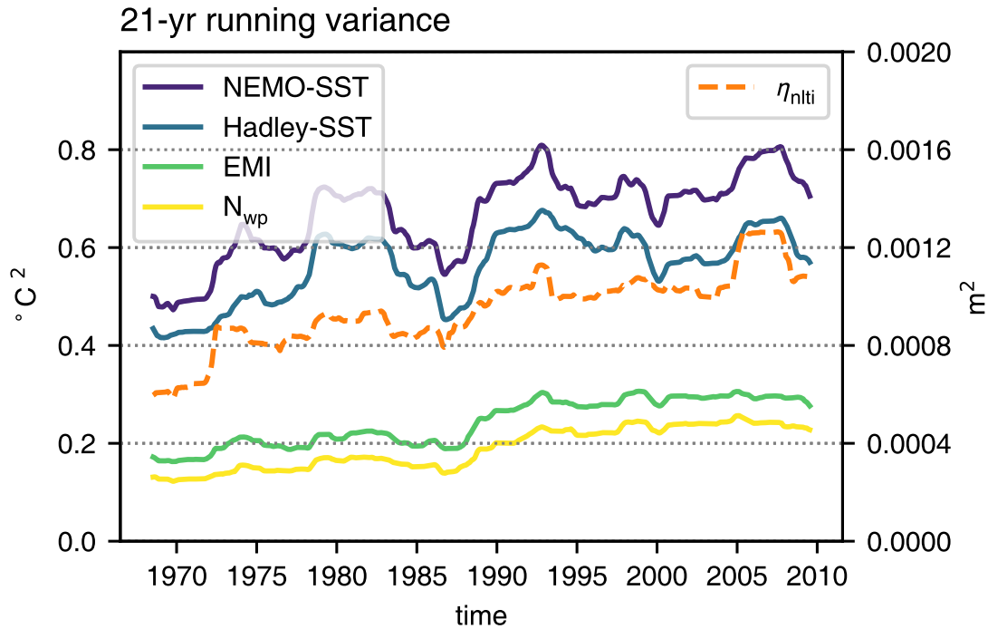
Figure 4. Variance in running 21 year windows of time series of different indices averaged along the equator between 160^{\circ}E and 150^{\circ}W , corresponding to the Niño4 region and computed using monthly mean anomalies. NEMO-SST refers to SST taken from the NEMO model simulation and Hadley-SST to SST taken from the HadISST data set. The units are (^{\circ}C)^2 (left axis) except for the index based on \eta_{nlti} which has units m^2 (right axis).
