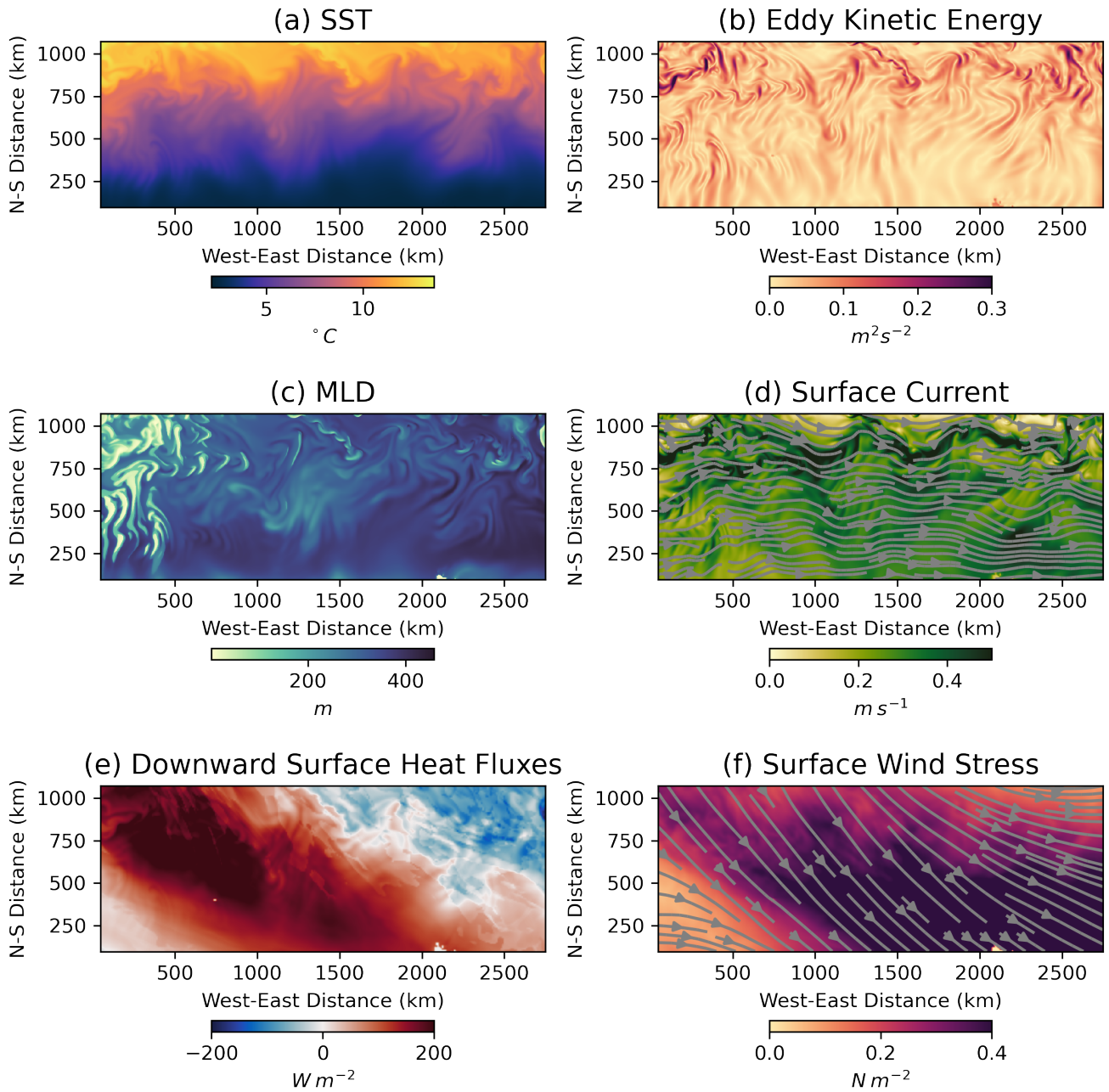
Figure 1. Examples of model simulated fields (values on September 1st, 2016): a) sea surface temperature, b) [.. 7 ] eddy kinetic energy, c) mixed layer depth (MLD), d) surface ocean current speed, e) downward sea surface heat fluxes, and f) surface wind stress.
