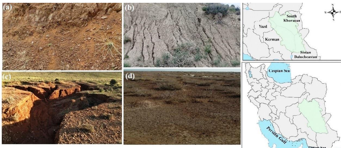
۱۱۷ Fig.1 Geographical location of the study watershed. Green shading marks the Lut watershed. The Lut ۱۱۸ Desert is located in the centre of the watershed. Settlements are primarily situated in the northern and ۱۱۹ south-western parts. Example of soil erosion in the watershed are sheet erosion (a), rill erosion (b), ۱۲۰ gully erosion (c), and wind erosion (d).
