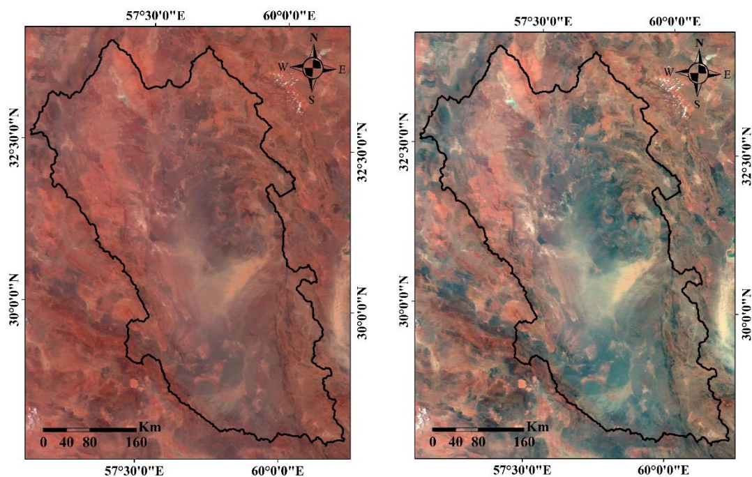
۳۴۴ Fig.4 The dust storm on 07 August 2019, as seen above is an example of the visual ۳۴۵ inspection of a dust storm (a) MODIS true colour (Red: Band 5, Green: Band 4, Blue: ۳۴۶ Band 3), and (b) enhanced MODIS satellite photos, (Red: BTD2931, Green: Band 4, ۳۴۷ Blue: Band 3).
