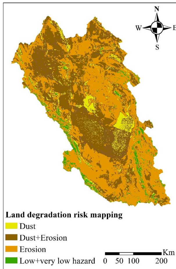
٤٩٣ ٤٩٤ Fig. 7 Land degradation susceptibility map in terms of soil erosion and dust sources areas ٤٩٥
