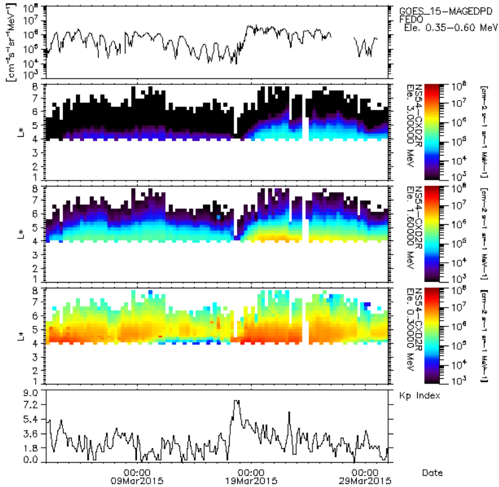
Figure 5. Overview of the assimilated data in Salammô-EnKF during the March 2015 simulations. From the top to the bottom, GOES-15 MAGED omnidirectional differential flux measurements for electrons from 350 keV to 600 keV, the GPS-NS54 CXD omnidirectional differential flux measurements for electrons at 3 MeV, 1.6 MeV, 300 keV, and the Kp index.
