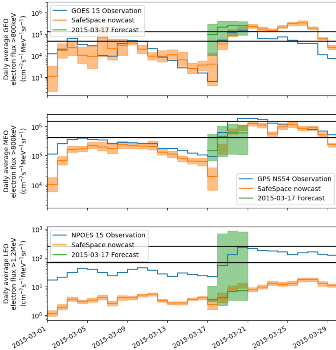
Figure 6. Comparison between the indices derived from the SafeSpace nowcast simulation (in orange for the median, and light orange for the 10th-90th decile percentile ensemble range), from the SafeSpace forecast simulation (in green for the median, and light green for the 10th-90th decile percentile ensemble range), with their associated reference observations (from the top to the bottom : GEO, MEO and LEO orbits). The solid black lines represent by increasing order, the moderate and active alarm thresholds.
