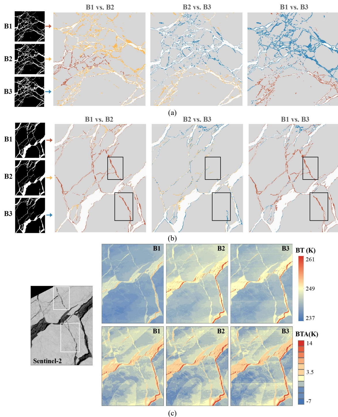
390 Figure 10: Cross-comparisons of lead detections among three TIS bands. The first column in (a) and (b) shows detections by the three bands. The following three columns are the pairwise comparisons, with dark red, orange, and dark blue representing the B1, B2, and B3 results, respectively. White pixels are consistency detections, and light gray indicates ice surface. Acquired from the
