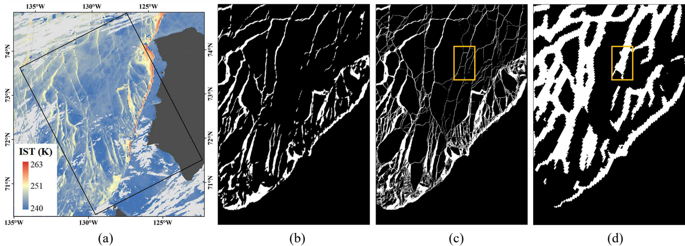
Figure 11: Comparisons of lead detections from MODIS data and SDGSAT-1 TIS data in the Beaufort Sea on April 3, 2022. (a) MODIS IST product with off-white clouds, dark gray land, and overlaid black border denoting coverage for (b), (c) and (d). (b) Lead detections at 1 km resolution from MODIS IST. (c) Lead detections at 30 m resolution from the combined result of TIS B1, B2 and B3 bands. IDs: KX10_TIS_20220403_W126.10_N71.30_202200033225, KX10_TIS_20220403_W128.84_N73.00_202200033226, KX10_TIS_20220403_W132.14_N74.67_202200033227. (d) Lead detections at 1 km resolution from Hoffman et al. (2022b).
