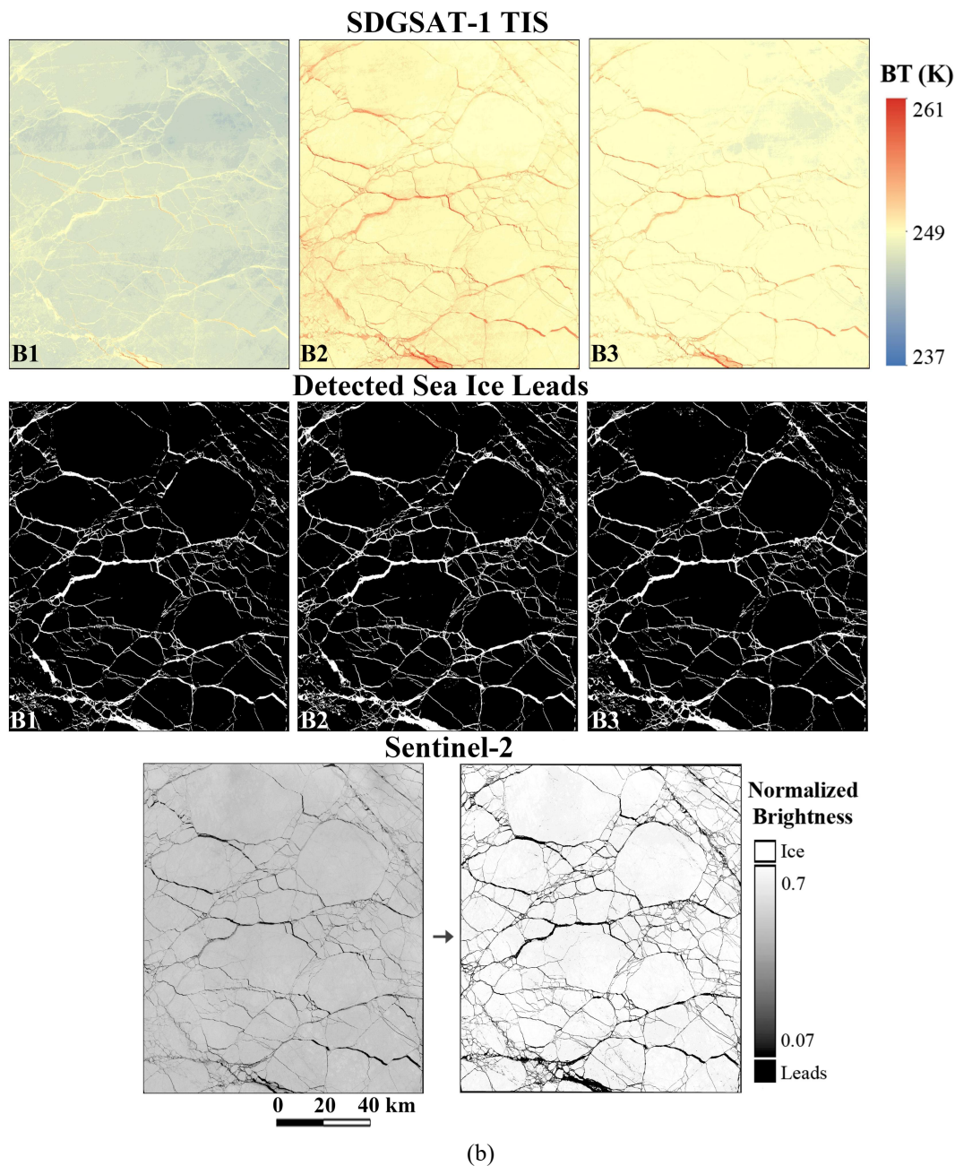
Figure 8: Validation of sea ice lead detection based on SDGSAT-1TIS data compared with S2 visible images in the Beaufort Sea, April 2022. Rows show the BT maps for the B1, B2 and B3 bands, the lead detection results, the S2 images and the normalized brightness (from 0.07 to 0.7). (a) TIS data acquired at 04:28 UTC and S2 data at 21:00 UTC on April 3, 2022. IDs: KX10_TIS_20220403_W128.84_N73.00_202200033226, KX10_TIS_20220403_W132.14_N74.67_202200033227. (b) TIS data acquired at 04:56 UTC and S2 data acquired at 22:42 UTC on April 28, 2022. ID: KX10_TIS_20220428_W147.26_N77.60_202200049406.
