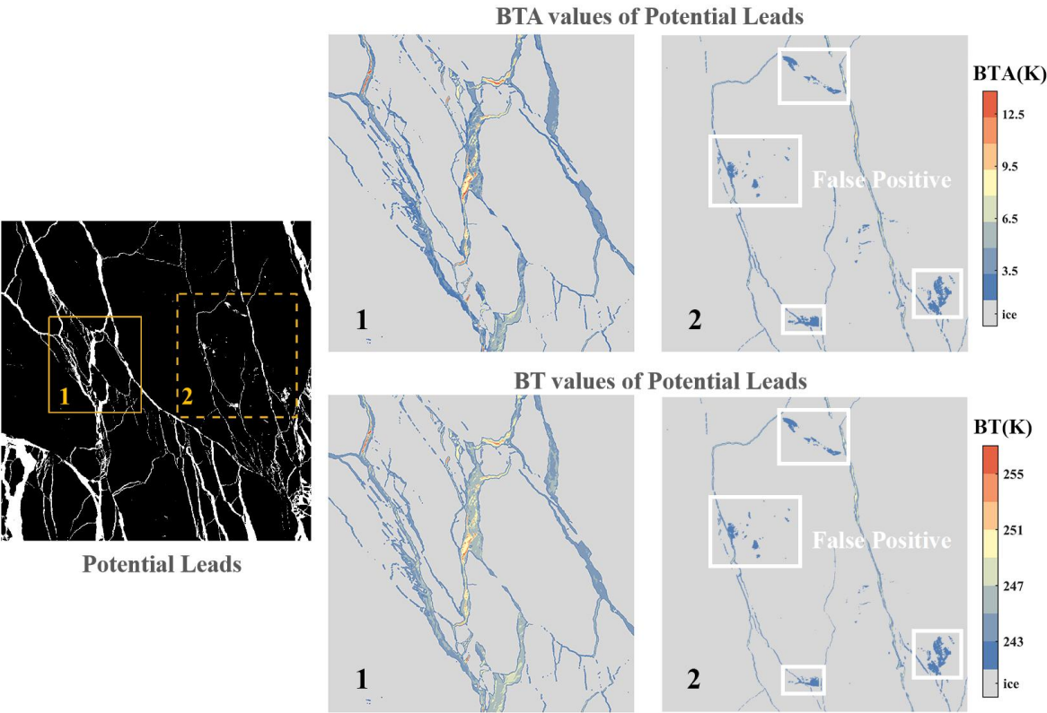
260 Figure 6: Characteristics of potential leads after segmentation. The left panel presents a binary image of potential leads detected by segmentation (the same as Fig. 5 (b)), with the two squares highlighted: view 1 represents highly reliable detection, while view 2 is part of a false-positive detection. Corresponding to the two views, the right panel displays the BTA images of these potential leads in the first row and the BT images in the last row, with the gray background representing the ice surface. SDGSAT-1 TIS data ID: KX10_TIS_20220403_W128.84_N73.00_202200033226.
