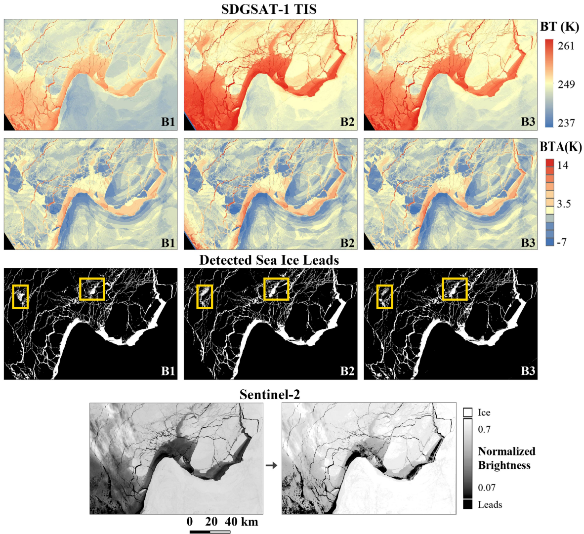
355 Figure 9: Application of the lead detection method to the SDGSAT-1 TIS data acquired over the Laptev Sea at 10:53 UTC on 360 March 23, 2022, and comparison with the S2 visible image at 03:55 UTC on the same day (similar illustration to the previous figure). IDs: KX10_TIS_20220323_E129.38_N75.60_202200028841 and KX10_TIS_20220323_E133.08_N73.96_202200028843
