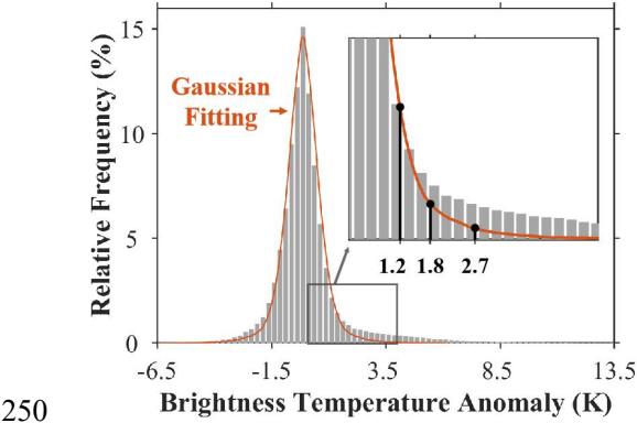
250 Figure 4: Statistical BTA histogram of seven TIS data acquired from April 3 to April 28, 2022, with a bin width of 0.25 K. The orange curve is the Gaussian fitting, with \mu = -0.25 K and \sigma^2 = 0.38 K.
