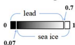
Figure R3 Diagram of a binary cases (sea ice and lead) for the normalized brightness.
