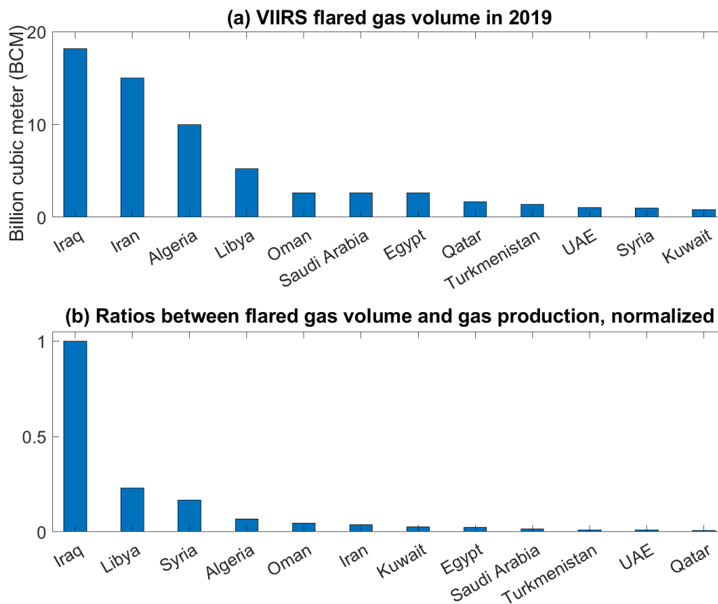
Figure 12. Flared gas volume in 2019 from major oil/gas producing countries. Top panel shows flared volume derived from flare radiances detected by the Visible Infrared Imaging Radiometer Suite (VIIRS) instrument. Bottom panel shows ratios of flared gas volume to gas production in 2019 normalized by a value of 264 m 3 flared gas per barrel of oil equivalent produced for Iraq.
