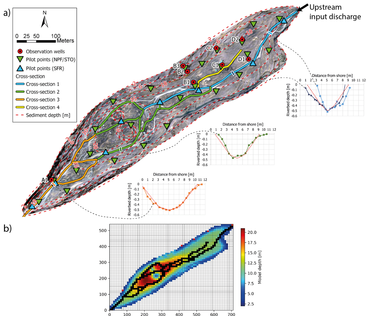
Figure 2. a) Overview of outwash plain model parameters. Six pilots points are used for streamflow (SFR) and 15 for hydraulic conductivity (NPF) and storage (STO). Observation wells are used for history-matching. Sediment depth was drawn manually based on ERT profiles and the two anomalies in the largest part of the floodplain are due to buried ice (see Sect.4.1). River cross-sections are separated in 4 classes, two bathymetrics profiles are shown for Cross-section 1 (light/dark blue), one for cross-section 2 (green) and cross-section 3 (orange). The dashed red line in the graphs represents the corresponding simplified cross-section used as model input. b) Corresponding MODFLOW grid. The colorscale represents the maximal model depth. The stream network is shown in black and the red squares represent the location of recharge and input discharge.
