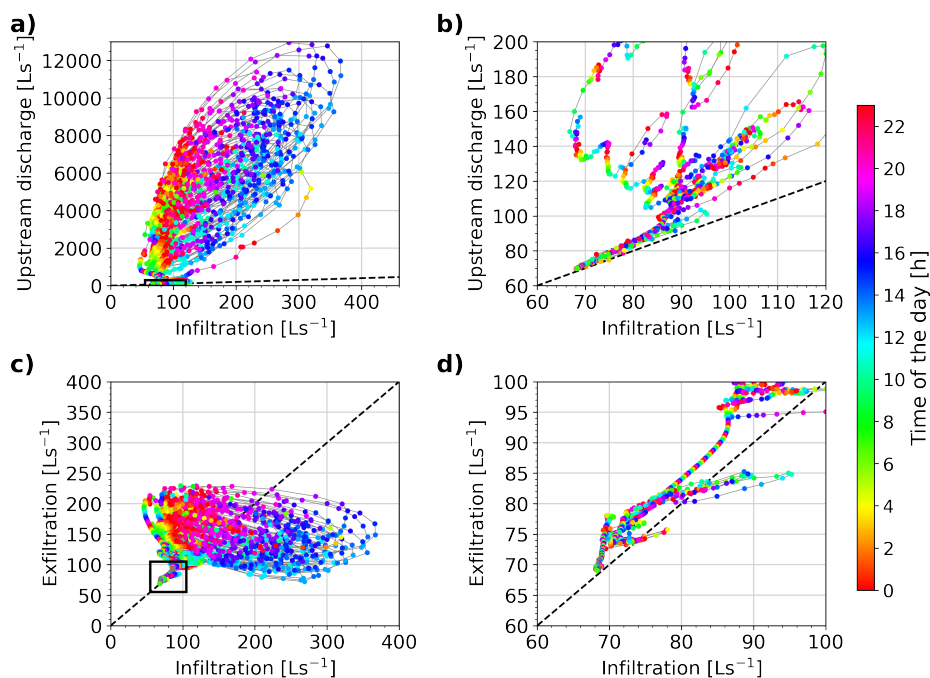
Figure 8. Surface water - groundwater exchanges. (a) Relationship between river reach infiltration and incoming upstream river discharge. (c) Relationship between river reach infiltration and groundwater exfiltration into the stream. The black rectangles indicate the zone of the zoom-in windows of the graph on the right (b) and (d). The colorscale corresponds to the hour of the day for each point. The straight dashed lines show the line of equal values.
