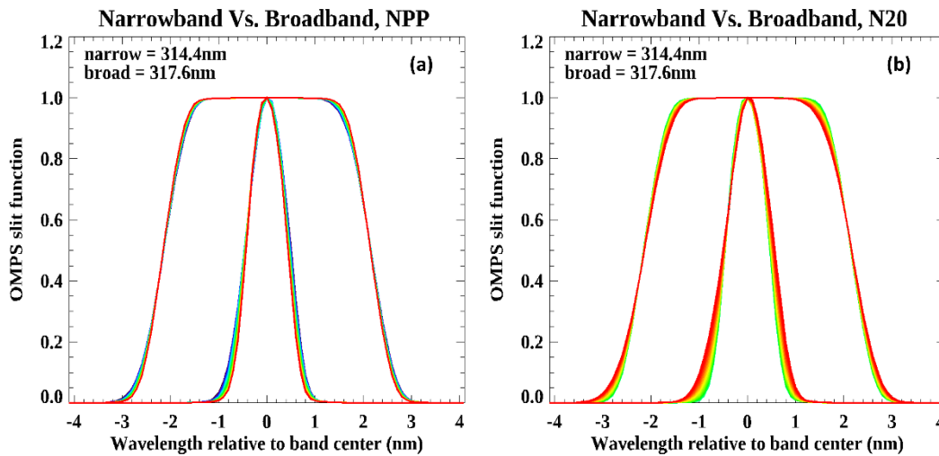
Figure 2. (a) OMPS NPP pre-flight slit function at 314.4 nm narrowband center and 317.6nm broadband center for 35 cross-track positions, with colors representing different cross-track positions from 1 (blue) to 35 (red). (b) Same as (a) but for OMPS N20.
