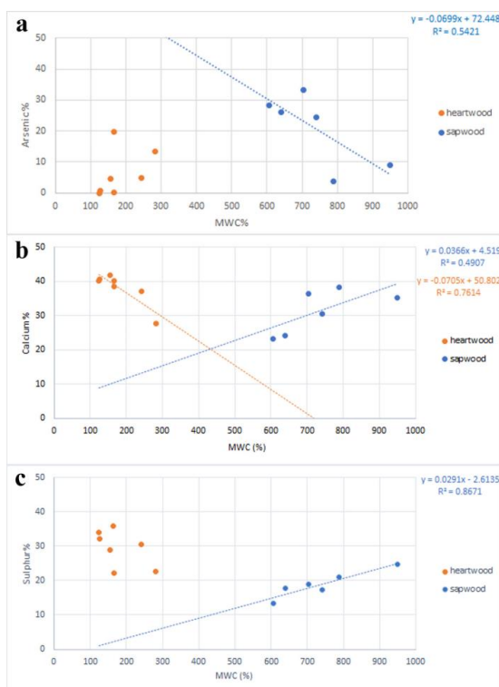
Figure 5 – Regression analyses performed between the percentages of the three most abundant metals and Maximum Water Content (MWC). (a) Arsenic; (b) Calcium; (c) Sulphur.
