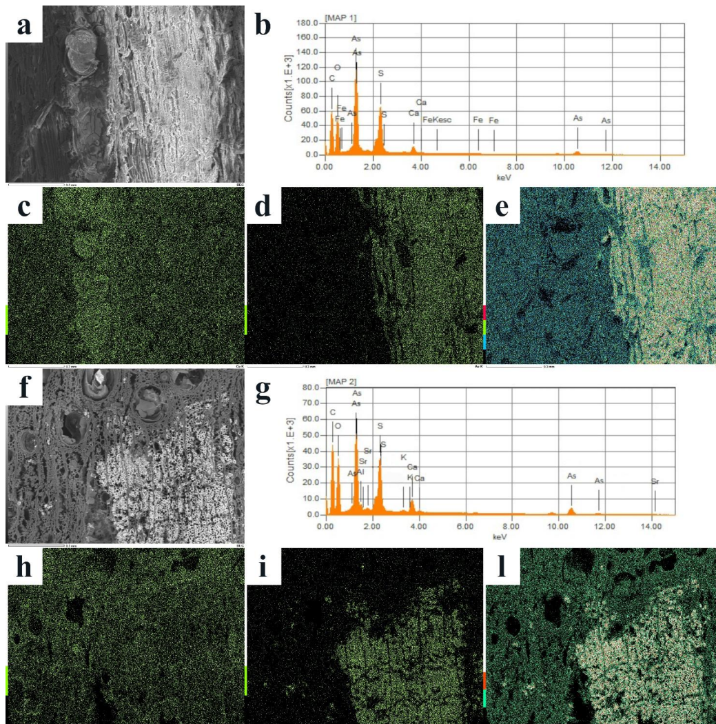
Figure 2 - BSE (a, f) and EDS maps and charts (b-e, g-l) of sapwood representative samples. (a-e) Radial section. (f-l) Tangential section. (a, f) the white areas correspond to the yellowish deposit in the sample. (b) EDS chart of the section in Figure 2a. (c) Ca; (d) As; (e) S; (g) EDS chart of the section in Figure 2f. (h) Ca; (i) As; (l) S.
