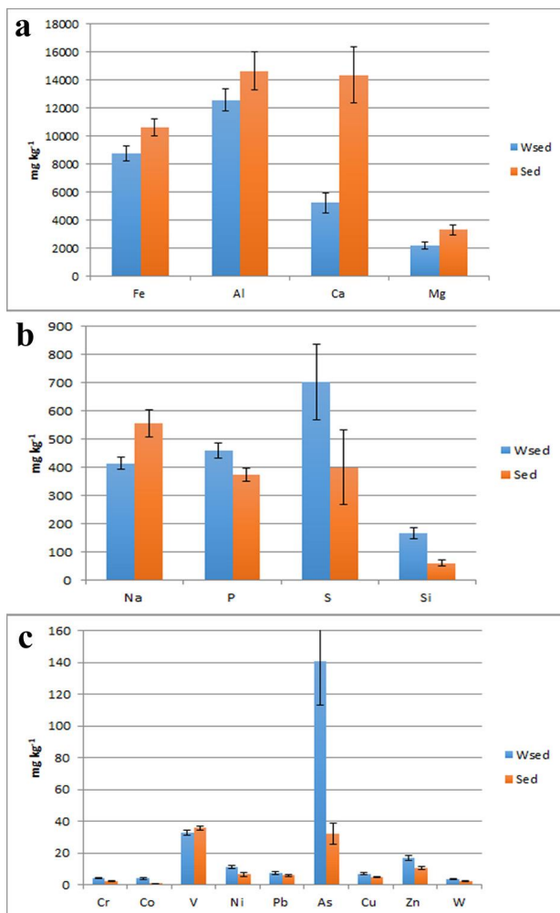
Figure 6 – Concentration of minerals and heavy metals in the sediments of Bolsena lake. (a) Elements originated from the lithological substrate; (b) elements of mixed origin; (c) Heavy metals (natural and/or anthropogenic sources).
