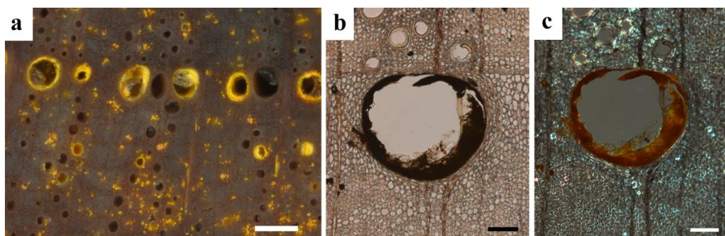
Figure 1 - Pole 125, microscope view in cross section and elemental analysis of inorganic deposits in wood cells. (a) stereomicroscope; (b) bright field optical microscope; (c) polarized light optical microscope. Scale bar: (a) 0.5 mm; (b, c) 100 \mu m.
