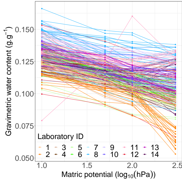
Figure 3. SWRCs Observed series of the entire data set expressed with four successive retention points (10 hPa, 50 hPa, 100hPa and 300 hPa) connected by straight lines. Water content is gravimetric ( \text{g.g}^{-1} ) water contents. One colour represents one laboratory. This colour code is kept constant throughout the paper.
