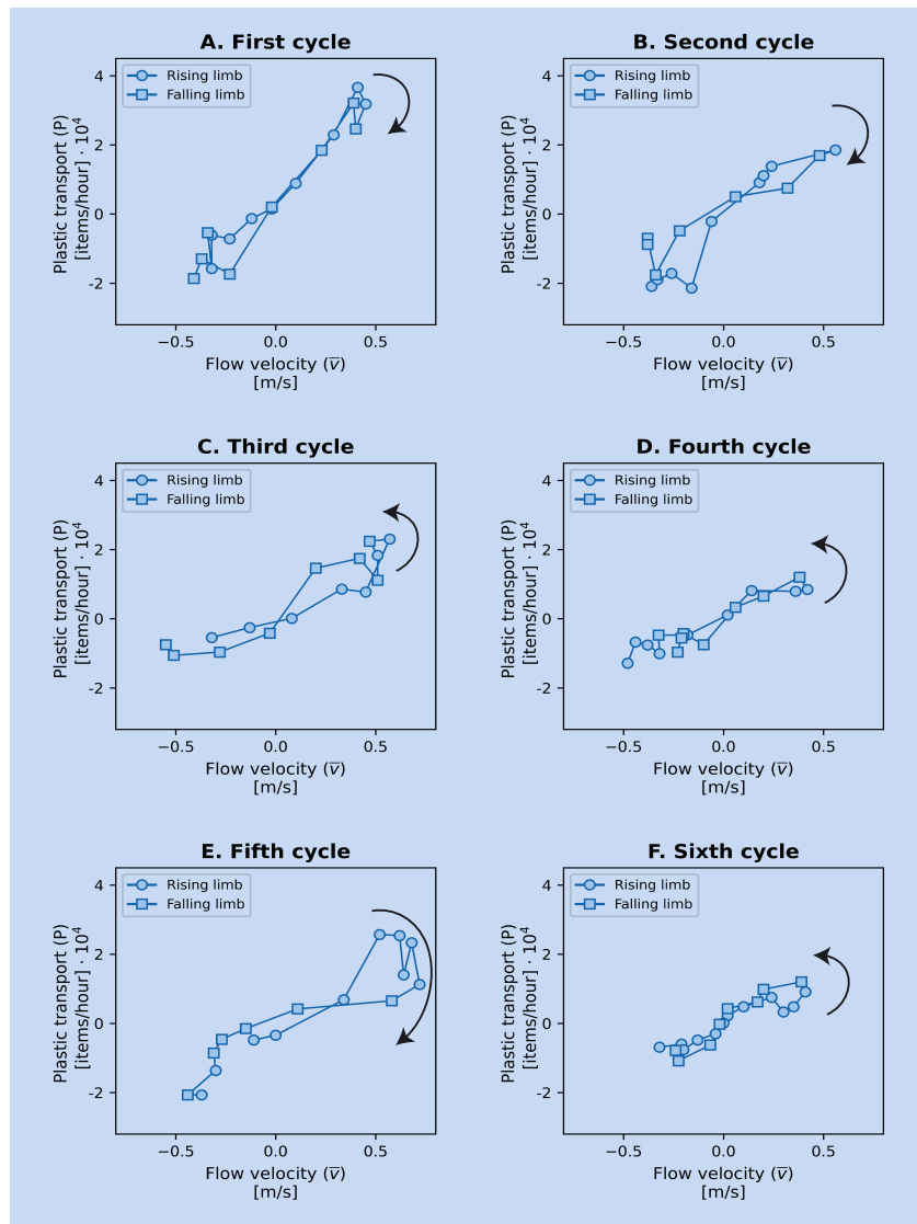
Figure C3. Relationship between plastic transport and flow velocity per tidal cycle (A-F). The arrows indicate the direction of the hysteresis (clockwise or anticlockwise) between rising and falling limbs of the tidal cycle.
