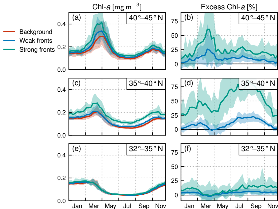
Figure 7. Seasonal subtropical biome: local impact of fronts on Chl-a excess over fronts by range of latitudes in the biome . (a-c-e) Chl-a median values over weak fronts (blue), strong fronts (green) and background (red), (b-d-f) corresponding local excess of Chl-a in weak and strong fronts computed as the relative difference of Chl-a in fronts and in the background. The plain lines represent the climatological mean, and the envelopes mark the standard deviation over the period 2000–2020. The excess is maximum at mid-latitudes.
