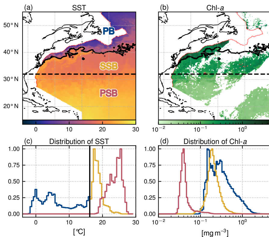
Figure 1. Delimitation of the three biomes in the open ocean Gulf stream-Stream extension region: the Permanent Subtropical Biome (PSB, south of the dashed line at 32°N), the Seasonal Subtropical Biome (SSB, between 32°N and the meandering Gulf stream-Stream northern wall on that day marked with the black contour), and the Subpolar-sub-Polar Biome (PB, north of the Gulf stream-Stream northern wall). (a) SST and (b) Chl- a snapshots on the 22 April 2007 (with data masked by clouds in white); The red line follows the 1500m isobath. Data on the continental shelf (< 1500m) is not considered here and have been masked. (c) SST and (d) Chl- a distribution within each biome for the same day (PB: blue , SSB: yellow , PSB: red ). The black line in (c) shows the SST threshold value detected to delimit the Gulf Stream northern wall (see methods section). The x-axis of the distributions correspond to the x-axis scale of the corresponding color bars. The red line follows the 1500m isobath. Data on the continental shelf (< 1500m) is not considered here and have been masked.
