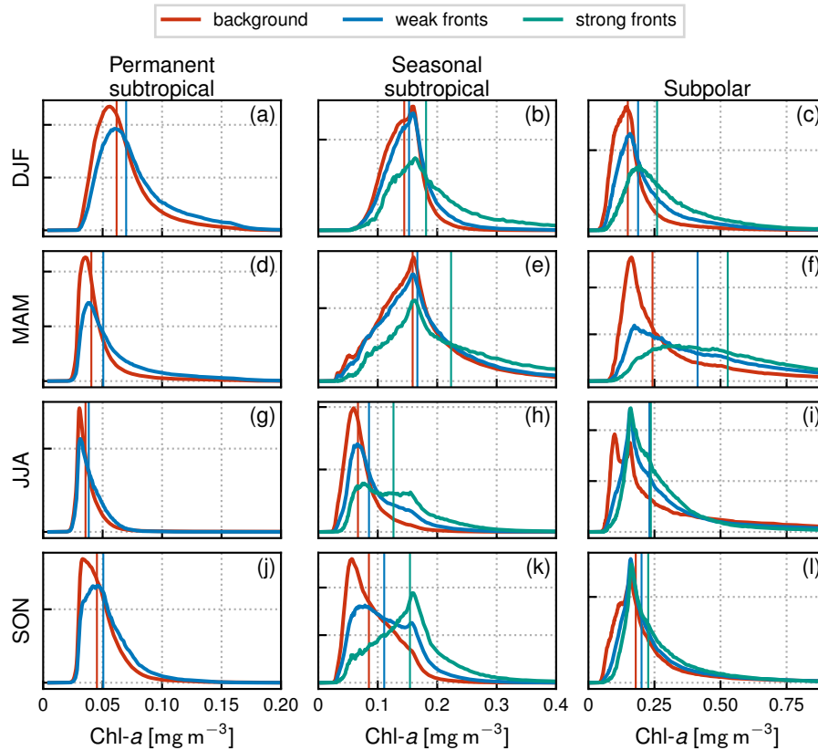
Figure A2. Distribution of Chl-a of the year 2007 by seasons (rows), for the three biomes (columns), and for the background (red), weak fronts (blue) and strong fronts (green). The median value of each distribution is indicated by a vertical line.
