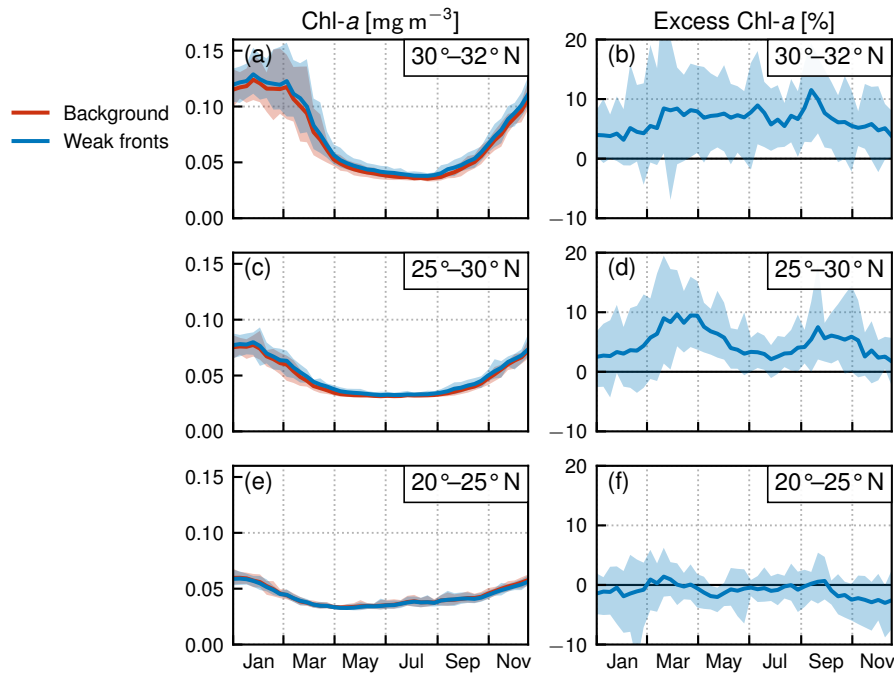
Figure 6. Permanent subtropical biome: local impact of fronts on Chl-a excess over fronts by range of latitudes in the biome . (a-c-e) Chl- a median values over weak fronts (blue) and background (red), (b-d-f) corresponding local excess of Chl- a in weak fronts computed as the relative difference of Chl- a in fronts and in the background. The plain lines represent the climatological mean, and the envelopes mark the standard deviation over the period 2000–2020. The excess increases from south to north.
