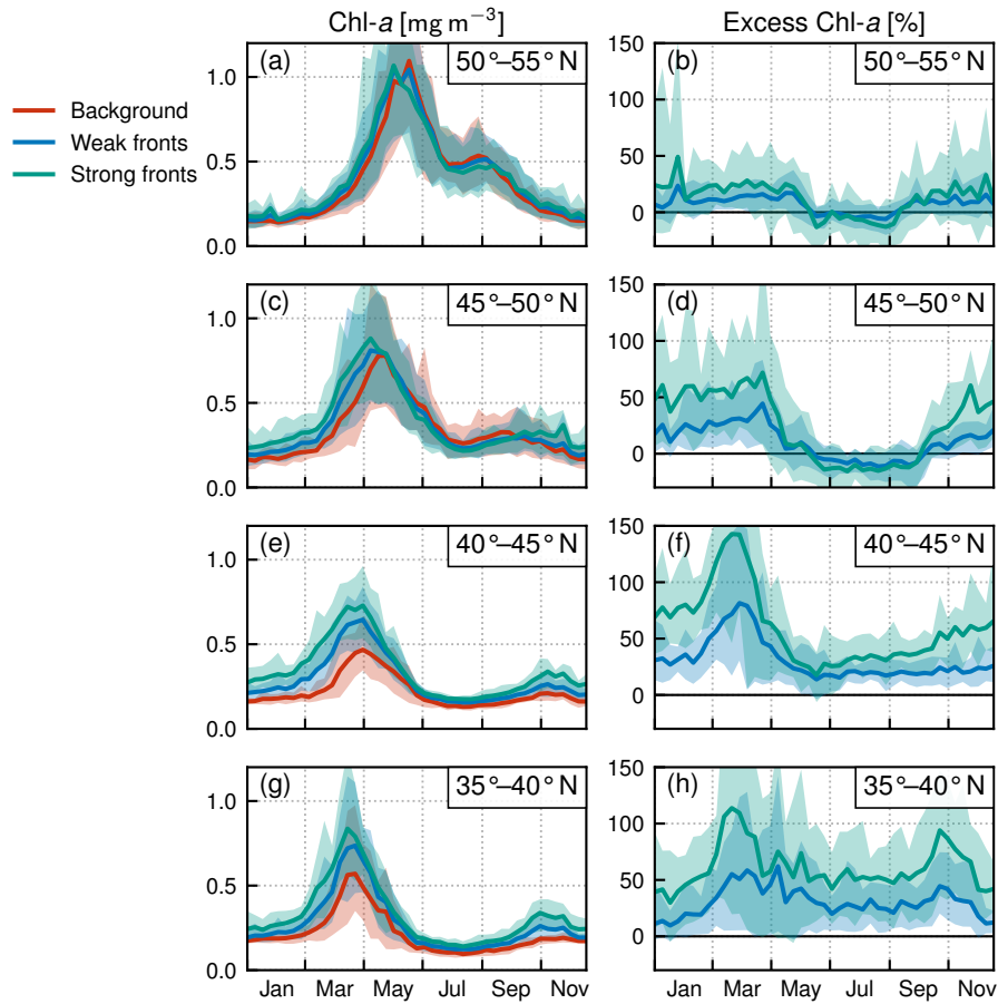
Figure 8. Subpolar biome: local impact of fronts on Chl-a excess over fronts by range of latitudes in the biome. (a-c-e) Chl- a median values over weak fronts (blue), strong fronts (green) and background (red), (b-d-f) corresponding local excess of Chl- a in weak and strong fronts computed as the relative difference of Chl- a in fronts and in the background. The plain lines represent the climatological mean, and the envelopes mark the standard deviation over the period 2000–2020. The excess decreases from south to north.
