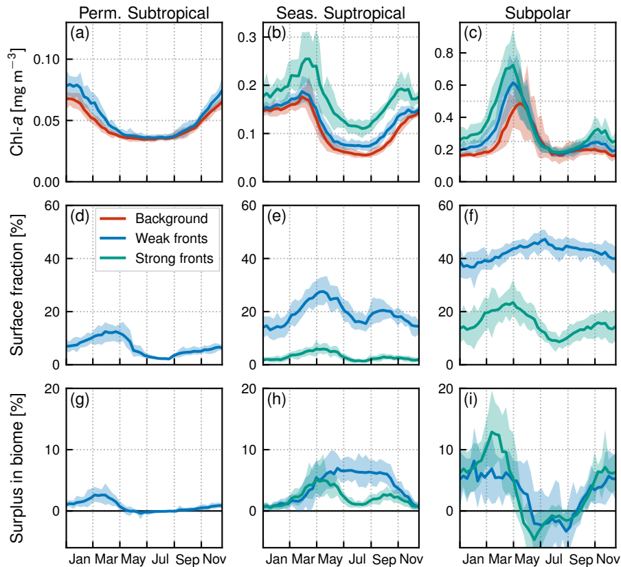
Figure 5. Seasonal impact of fronts on Chl-a climatologies in the permanent subtropical biome (1st column), in the seasonal subtropical biome (2nd column) and in the subpolar biome (3rd column). (a-b-c) Chl-a median values (top row) over weak fronts (blue), strong fronts (green) and background (red). The differences Gaps between the curves show represent the local impact at the scale of excess over fronts. (d-e-f) Surface fraction occupied by weak fronts and strong fronts. (g-h-i) Global-Regional Chl-a surplus due to weak fronts and strong fronts at the scale of the biome. The surplus accounts for the local excess and for the number of fronts (see method). The plain lines represent the climatological mean, and the envelopes mark the standard deviation over the period 2000–2020. The excess in Chl-a is more strongly enhanced larger over strong fronts than over weak fronts, but weak fronts are more numerous than strong fronts, resulting in a Chl-a surplus that can be reversed comparable or even larger for weak fronts .
