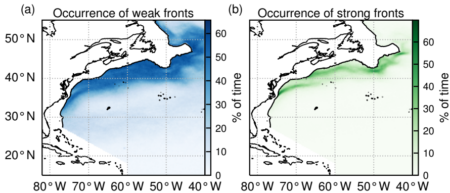
Figure 4. occurrence Occurrence of (a) weak fronts and (b) strong fronts expressed as the percentage of time steps over the entire time series (2000–2020) that for which a given pixel is occupied by a front.
