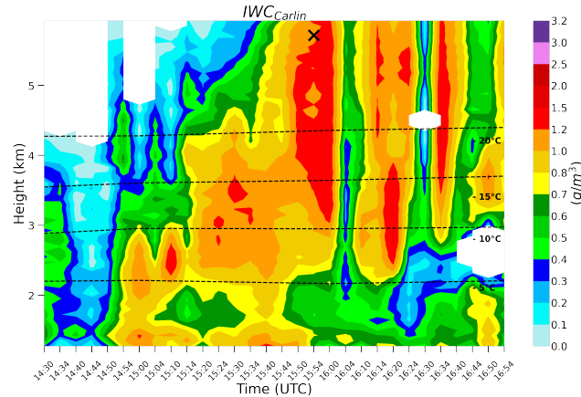
Figure 8. RSVPs of \text{IWC}_{\text{Carlin}} at ranges between 15.5 km–20 km from the DOW on 10 December 2015 between 14:30 and 16:54 UTC. Overlaid dashed lines display the -5^{\circ}\text{C} , -10^{\circ}\text{C} , -15^{\circ}\text{C} and -20^{\circ}\text{C} isotherms from ERA5 at the DOW location. The collocated data point is indicated by the black cross.
