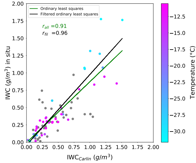
Figure 4. Scatter plots and linear regressions of IWC_{Carlin} vs. IWC from OLYMPEX in situ data. Temperature-dependent colouring of each data point indicates temperatures colder than or equal to -10^{\circ}\text{C} , while the gray dots, represent data masked via filter criteria for temperature ( T \geq -10^{\circ}\text{C} ) and intersection time ( t \leq 30 s). The r statistics are reported in green for all data points and in black for filtered ones.
