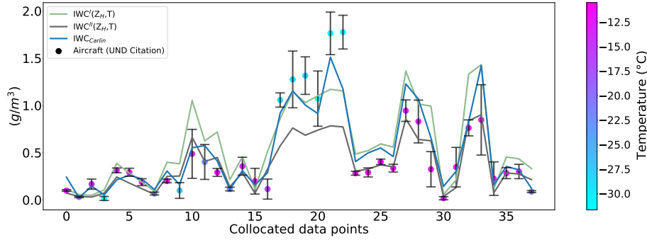
Figure 6. Collocated aircraft in situ data in chronological order (colored dots), the IWC^I(Z_H, T) (green), IWC^{II}(Z_H, T) (gray), and IWC_{Carlin} (blue) of RSVP data (solid lines) for 10 flight missions. Vertical bars have the same meaning as in Fig. 5.
