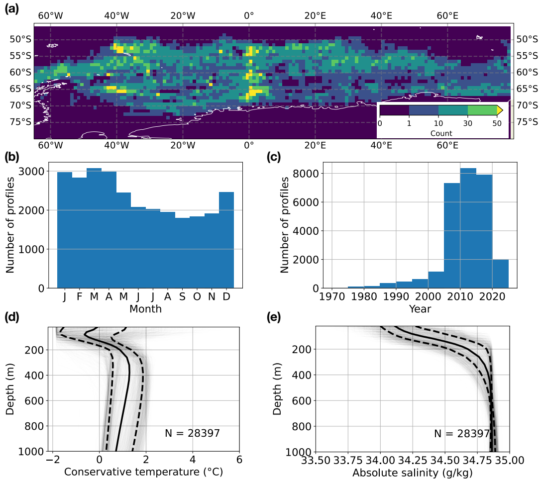
Figure 2. The distribution of profiles used in this study. (a) Number of profiles in the dataset shown in 1° latitude-longitude bins. Note that profiles with a maximum depth of less than 1000 m have been excluded. (b) Distribution of the profiles by month. (c) Distribution of the profiles in five-year intervals. (d) Random selection of 10% of the conservative temperature profiles by depth (thin grey lines), shown with the 25th percentile (thin dashed line, left), the median (solid black line), and the 75th percentile (thin dashed line, right). (e) Same as (d), for absolute salinity. The total number of profiles is N = 28,397 .
