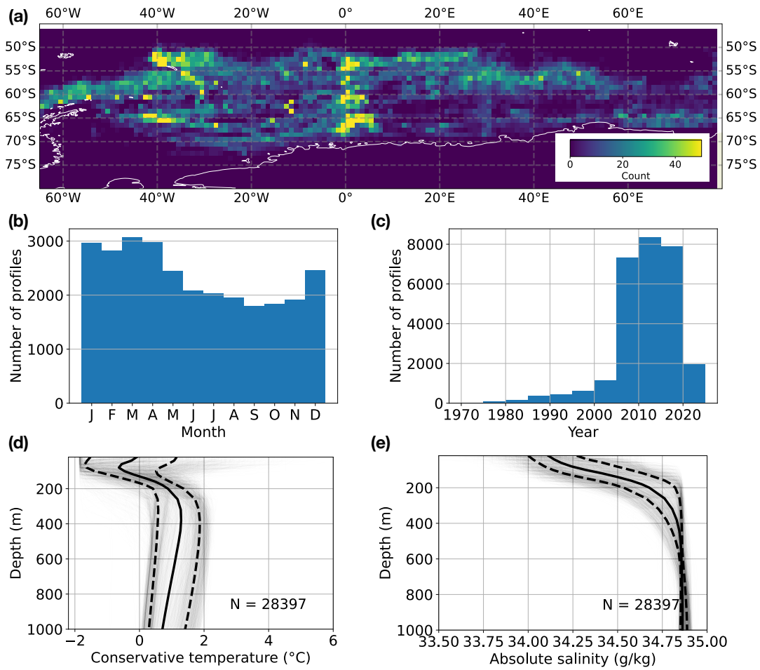
Figure 2. The distribution of profiles used in this study. (a) Number of profiles in the dataset shown in 1° latitude-longitude bins. (b) Distribution of the profiles by month. (c) Distribution of the profiles in five-year intervals. (d) Random selection of 10% of the conservative temperature profiles by depth (thin grey lines), shown with the 25th percentile (thin dashed line, left), the median (solid black line), and the 75th percentile (thin dashed line, right). (e) Same as (d), for absolute salinity. The total number of profiles is N = 28,397 .
