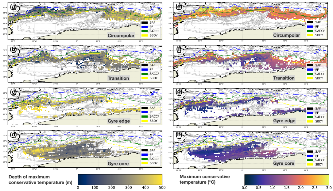
Figure 8. The depth of the conservative temperature maximum (left column) and the value of the conservative temperature maximum (right column), binned and averaged over 1^\circ latitude-longitude bins. The fronts and f/h contours are the same as in Figure 4.
