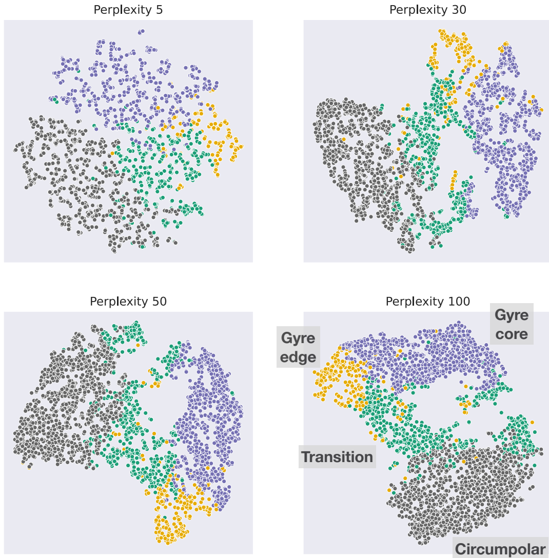
Figure 15. Visualisation of six-dimensional principal component space, transformed into a 2D space using t-SNE (Maaten and Hinton, 2008). The colours indicate the four classes into which the profiles have been sorted. Roughly speaking, the perplexity indicates the level of mutual “attraction” between nearby points during the fitting process. The axes are arbitrary dimensions and should not be interpreted quantitatively; they are for visualisation purposes only.
