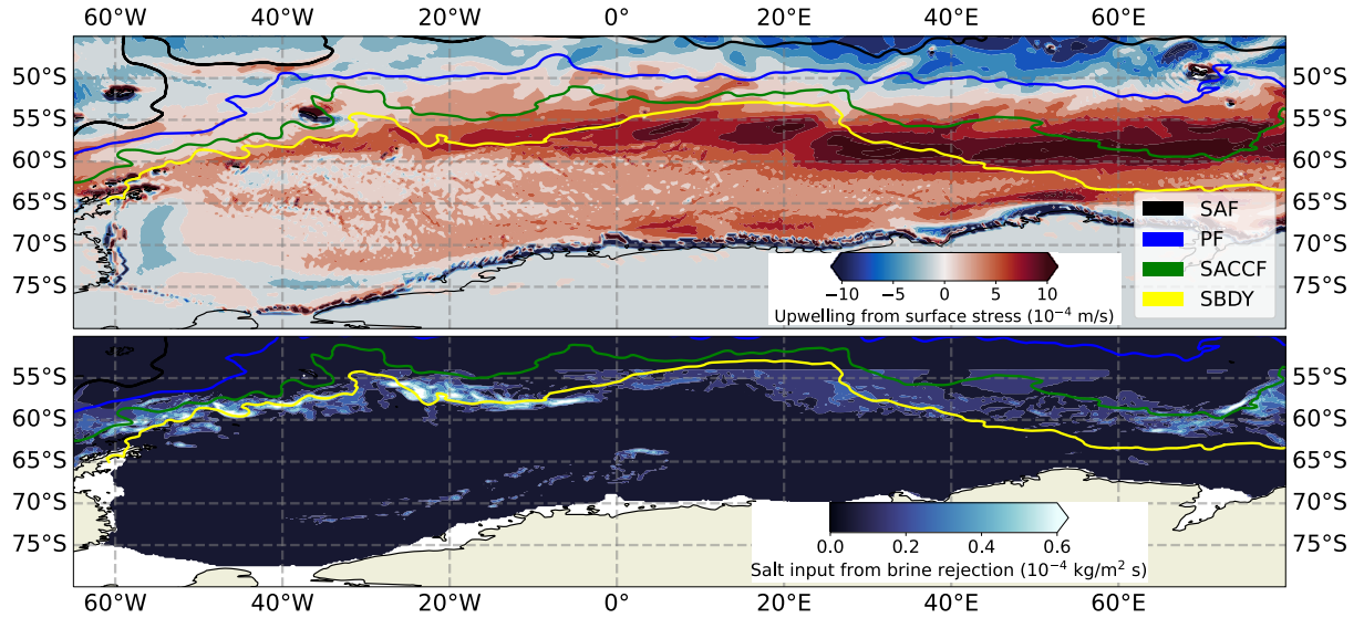
Figure 13. (a) Estimated upwelling ( 10^{-4} \text{ m s}^{-1} ) from surface stress, including the effects of wind stress, sea ice coverage, and sea ice drift, following Dotto et al. (2018). Sea ice concentration is from Climate Data Record v4 and sea ice drift is from Polar Pathfinder. (b) Approximate position of the wintertime sea ice freezing line, as indicated by the salt input from brine rejection during sea ice formation (negative freshwater input, shown in units of 10^{-4} \text{ kg m}^{-2} \text{ s}^{-1} ). Values below 10^{-5} \text{ kg m}^{-2} \text{ s}^{-1} have been masked out (i.e. set to zero). Data from SOSE averaged over JAS during the period 2005-2010 (Mazloff et al., 2010). The fronts are the same as in Figure 4 from Kim and Orsi (2014).
