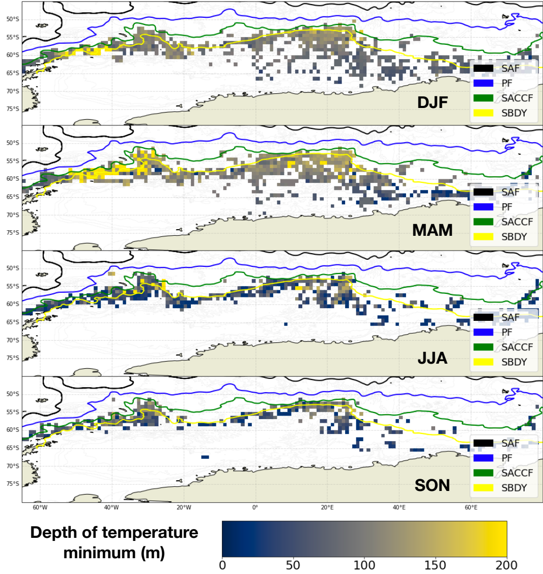
Figure 12. Depth of the conservative temperature minimum averaged over 1^\circ latitude-longitude bins, separated by season.
