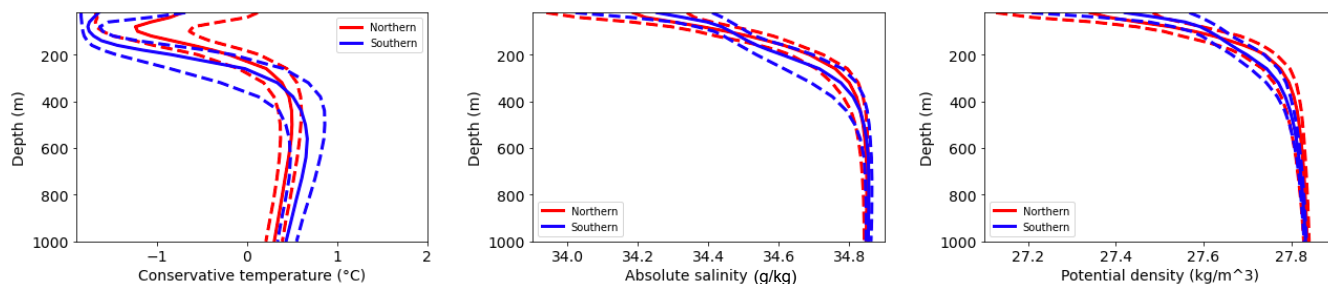
Figure 14. Compare northern and southern extents of the gyre edge class
