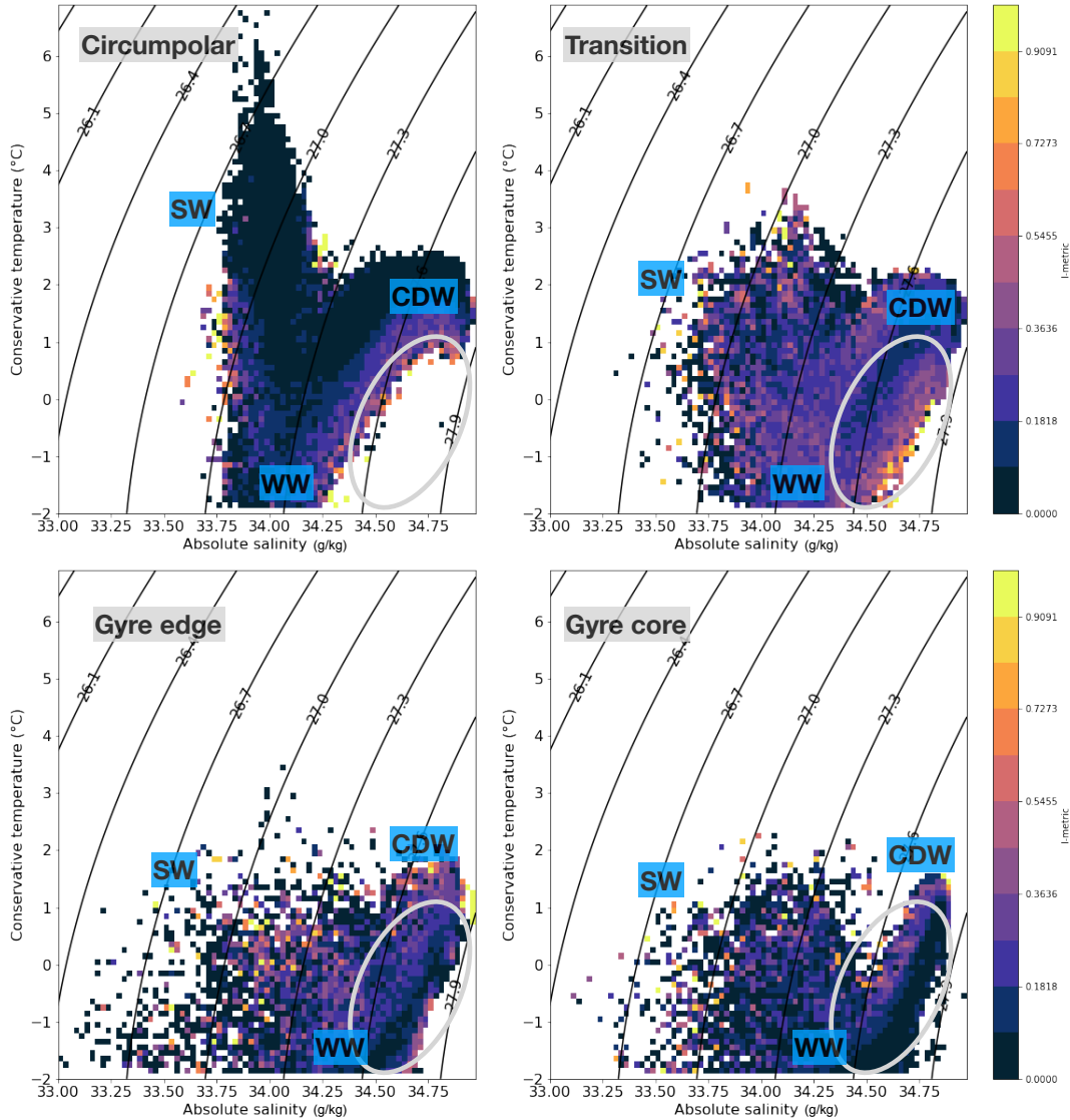
Figure 9. Temperature-salinity diagrams for the four classes. The shading indicates the mean I-metric value for each bin ( 0.1^{\circ}\text{C} , 0.025\text{ g/kg} ). Since each profile has a single I-metric value, the approach used here averages all profiles that pass through any given bin. The result is a relative indication of the core class properties versus the more peripheral ones. The solid lines are potential density contours ( \sigma_0 ). The grey oval indicates a potential signature of mixing between the winter water and deeper water. Also shown are the approximate locations of the surface water (SW), circumpolar deep water (CDW), and winter water (WW).
