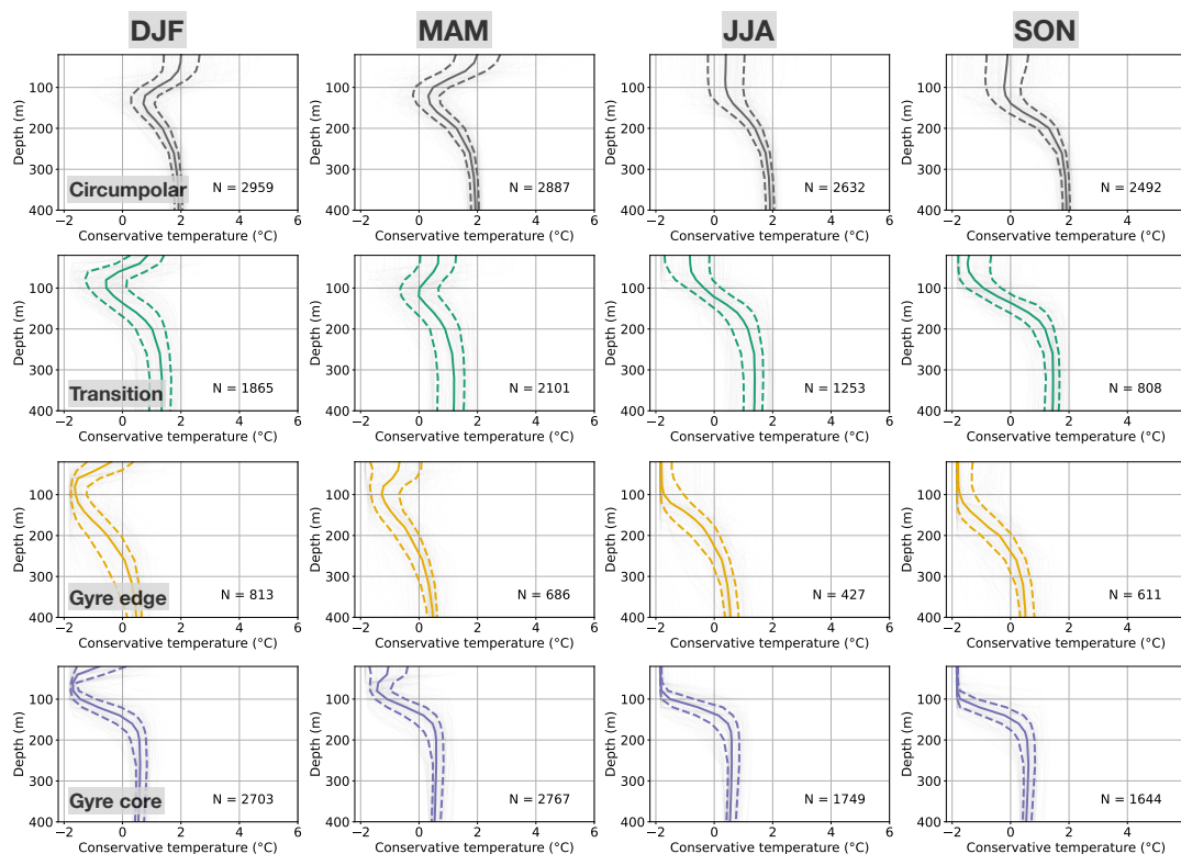
Figure 10. Distribution of the conservative temperature of the four classes, split by season. Each panel features a random selection of 400 profiles (thin grey lines), the 25th percentile (dashed line, left), the median (solid line), the 75th percentile (dashed line, right), and the number of profiles N in each class and season.
