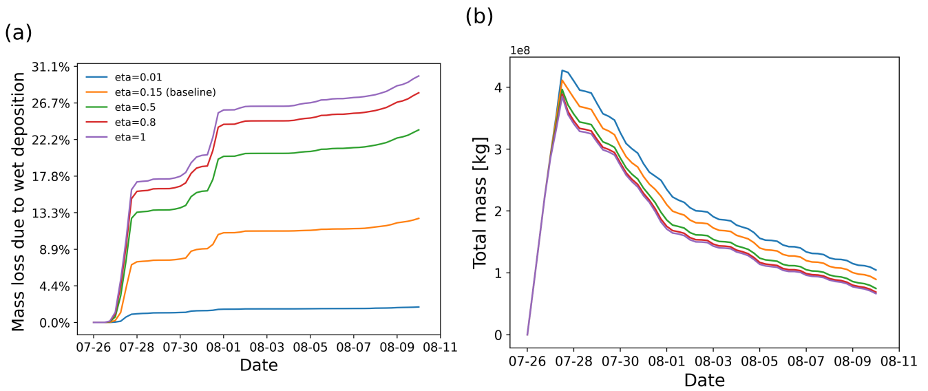
Figure 10. SO 2 mass loss relative to the total mass (in percent) due the wet deposition module(a) and total mass burden evolution (b), derived from different simulations with different retention ratios settings in the wet deposition module.
