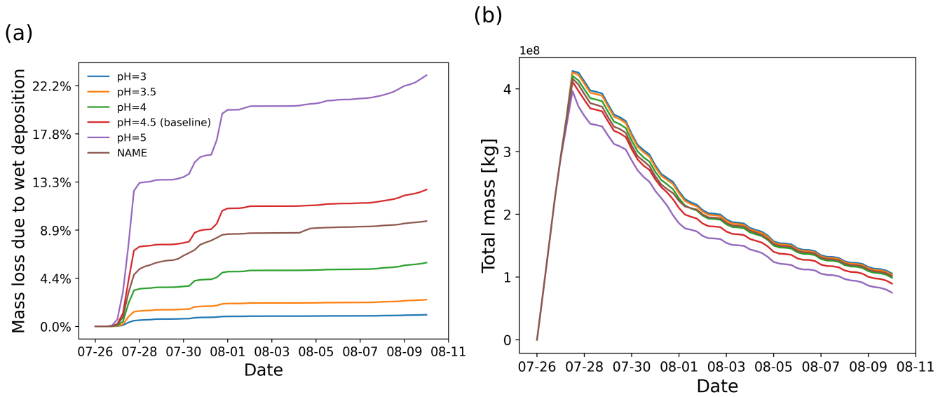
Figure 9. SO 2 mass loss relative to total mass (in percent) due to the wet deposition module (a) and total mass curves (b), derived from simulations with different pH values in the wet deposition module and comparing with the wet deposition scheme of the NAME model.
