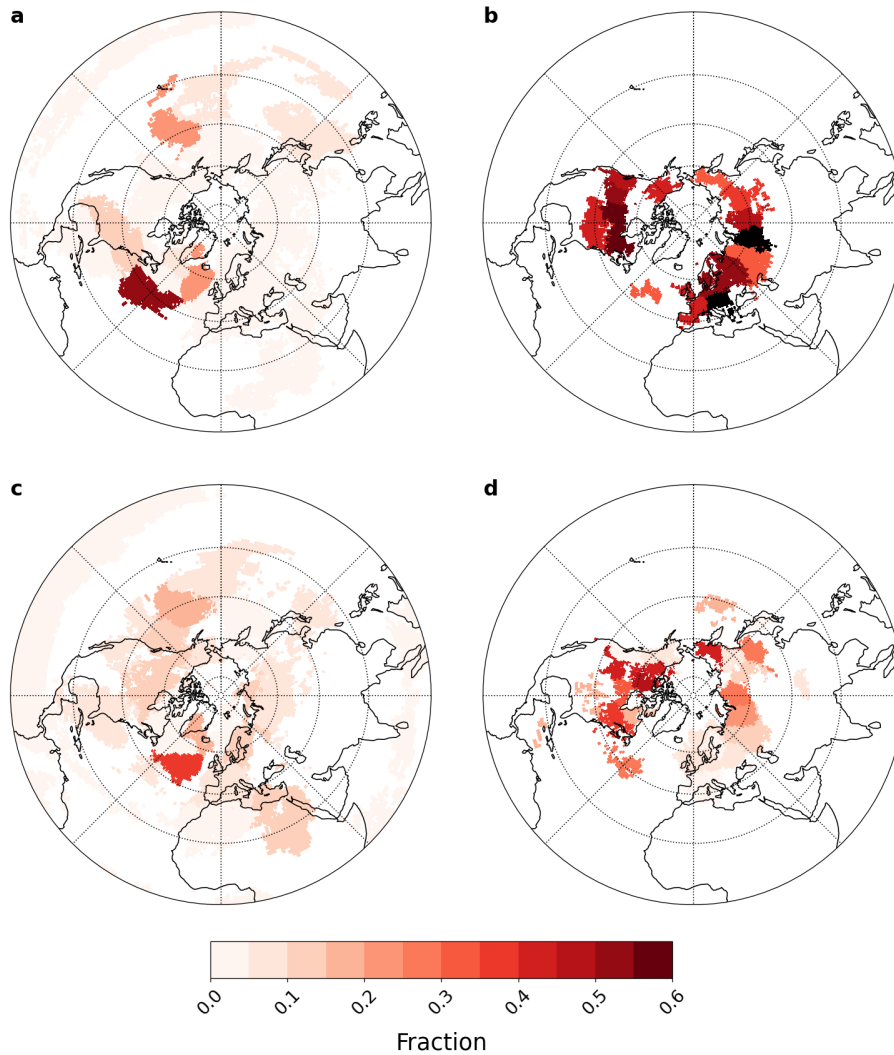
Figure A1. Fraction of 5-day 21-day persistent warm and/cold spells occurring within 21-day which do not include a 3-day extreme warm or/cold spells period, for (a) DJF cold spells, (b) JJA cold spells, (c) DJF warm spells and (d) JJA warm spells, averaged by region. In each case spells 3-day extreme periods are defined relative to the 95th or 5th percentiles of the corresponding 5- or 21-day based on daily 5 th /95 th temperature distribution percentiles.
