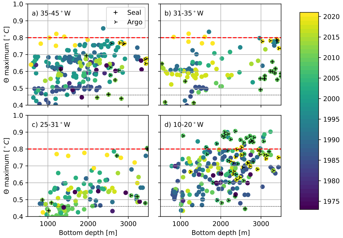
Figure 3. Maximum conservative temperature within the WDW-core from CTD-profiles obtained above the continental slope a) northwest of FT (35-45°W) b) north of the FT (31-35°W) c) northeast of the FT (25-31°W) and d) upstream of the FT region (10-20°W) as a function of bottom depth. The data points are color-coded with respect to time, and profiles obtained by seals or profiling floats are marked according to the legend. Note that seal profiles rarely cover the temperature maximum; the temperature shown is the highest temperature observed during a dive. The red dashed line marks 0.8°C and is included in all panels (and in subsequent figures when relevant) to facilitate comparison. The black line is the average two-week maximum temperature from the mooring records (see Fig. 6a-d and the text for an explanation).
