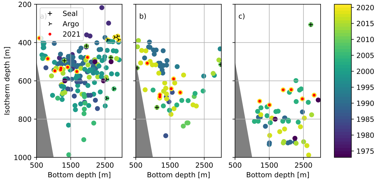
Figure 5. Scatter plot of the depth of the 0.5^{\circ}\text{C} isotherm versus bottom depth, where the color code indicates the year a) northwest of the FT ( 35-45^{\circ}\text{W} , 35-45^{\circ}\text{W} ) b) north of the FT ( 31-35^{\circ}\text{W} , 31-35^{\circ}\text{W} ) and c) northeast of FT ( 25-31^{\circ}\text{W} , 25-31^{\circ}\text{W} ). Profiles obtained by instrumented seals, Argo floats, or in 2021 are marked according to the legend.
