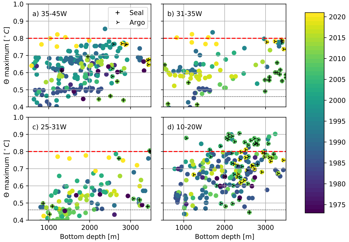
Figure 3. Maximum conservative temperature within the WDW-core from CTD-profiles obtained above the continental slope a) northwest of FT ( 35-45°W 35-45W ) b) north of the FT ( 31-35°W 31-35W ) c) northeast of the FT ( 25-31°W 25-31W ) and d) upstream of the FT region ( 10-20°W 10-20W ) as a function of bottom depth. The data points are color-coded with respect to time, and profiles obtained by seals or profiling floats are marked according to the legend. Note that seal profiles rarely cover the temperature maximum; the temperature shown is the highest temperature observed during a dive. The red -dashed line marks 0.8^{\circ}\text{C} and is included in all panels (and in subsequent figures when relevant) to facilitate comparison. The black line is the average two-week maximum temperature from the mooring records (see Fig. 6a-d and the text for an explanation).
