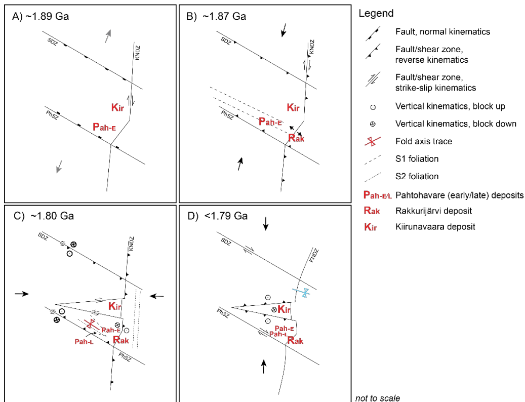
Figure 8: A proposal for the structural framework for the Kiruna mining district. A) The onset of the Svecokarelian orogeny and back arc extension forms and/or reutilizes preexisting normal faults, additional transtensional faults form. The earliest ca. 2.1 Ga Pahtohavare syngenetic deposit (Eastern, Pah-E) has already formed and the Kiirunavaara IOA deposit forms, B) NE-SW crustal shortening from the early Svecokarelian orogeny reactivates preexisting faults structures, forming transpressional shear zones and dilatational jogs. The Rakkurijärvi IOCG forms (Rak). Early S 1 fabric develops in the southern Kiruna mining district, C) Late orogenic E-W crustal shortening and basin inversion occurs. Stratigraphy in the Pahtohavare-Rakkurijärvi area is folded and S 2 foliation develops. Strong strain partitioning occurs with S 2 fabric forming along shear zones in the central Kiruna area. Both brittle and ductile structures form. The late epigenetic Pahtohavare deposits form (Pah-L), D) N-S crustal shortening causes gentle refolding in the district and minor reactivation of preexisting structures occurs. SDZ = Svappavaara deformation zone, KNDZ = Kiruna-Naimakka deformation zone, PhSZ = Pahtohavare shear zone.
