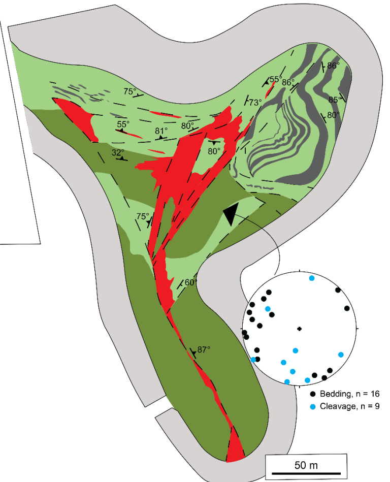
855 Figure 6: A) A mine level map at 300 m of the Southern Pahtohavare deposit showing albite felsite hosted Cu in a structurally-controlled position. The construction of the mine level map was done for resource estimates during the 1990s by utilizing vertical cross sections from profiles every ten meters along the strike of the ore body with 3 to 5 inclined drillholes in each profile intersecting the ore body at various depths. Geological contacts and structures have been interpolated from the vertical cross sections. Dipping of contacts and structures are estimated from the cross sections and are not based on actual structural measurements. B) The Southeastern Pahtohavare open pit showing both the stratabound and discordant ore zones. Structural measurements were acquired during mapping in the 1990s. 860
