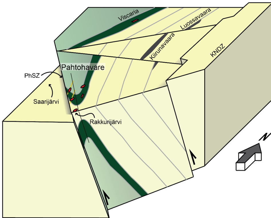
885 Figure 9: 3D conceptual model of the Pahtohavare area in the southern Kiruna mining district showing the oblique reverse NW-SE trending Pahtohavare shear zone and the resultant Pahtohavare F_2 fold. The axial surface is steeply dipping and the Pahtohavare epigenetic deposits are controlled by D_2 structures. Green colors denote older greenstone stratigraphy (ca. >2.1 Ga) and yellow colors denote ca. 1.92 Ga and younger stratigraphy. KNDZ = Kiruna-Naimakka deformation zone, PhSZ = Pahtohavare shear zone.
