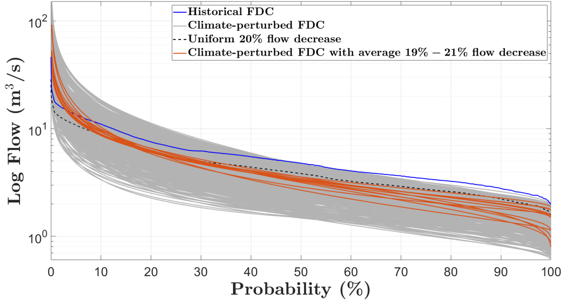
Figure 3. Plot of the flow duration curves (FDCs) of the historical record (blue line) and sampled flow duration curves (grey lines) constructed by deriving the FDC parameters for the Kosugi Model shown in Table 1. The figure also compares 20 % mean flow reductions, obtained either with the delta change method (uniform multiplier, dashed black line) and the 12 future scenarios we generated with mean flow reductions between 19 and 21 % (orange lines).
