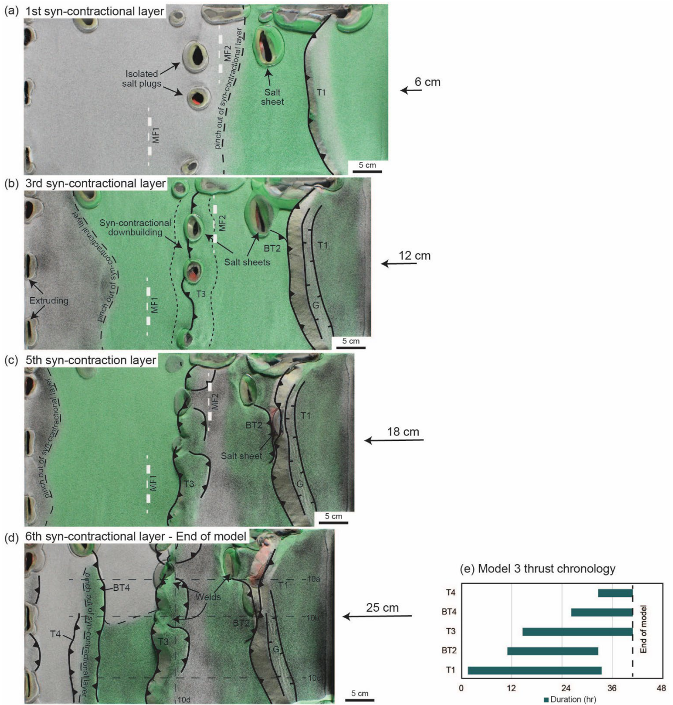
520 Figure 11. (a-d) Top-view images illustrating the contractional kinematic evolution of Model 3 (shortening with sedimentation), including the timing of thrust initiation, model salt extrusion from salt sheets, contractional welding of salt sheets, and the
