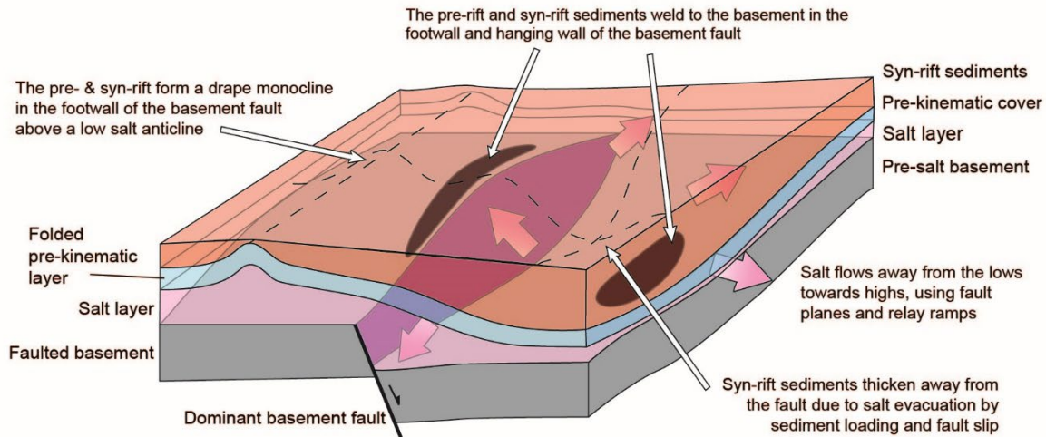
615 Figure 13. Block diagram illustrating the structural style of decoupled extensional rift half-graben with thick early syn-rift salt and a thin pre-kinematic layer bed showing the migration and inflation of salt away from the half-graben and the development of a synclinal minibasin within the basement half-graben. Modified and updated from Richardson et al (2005).
