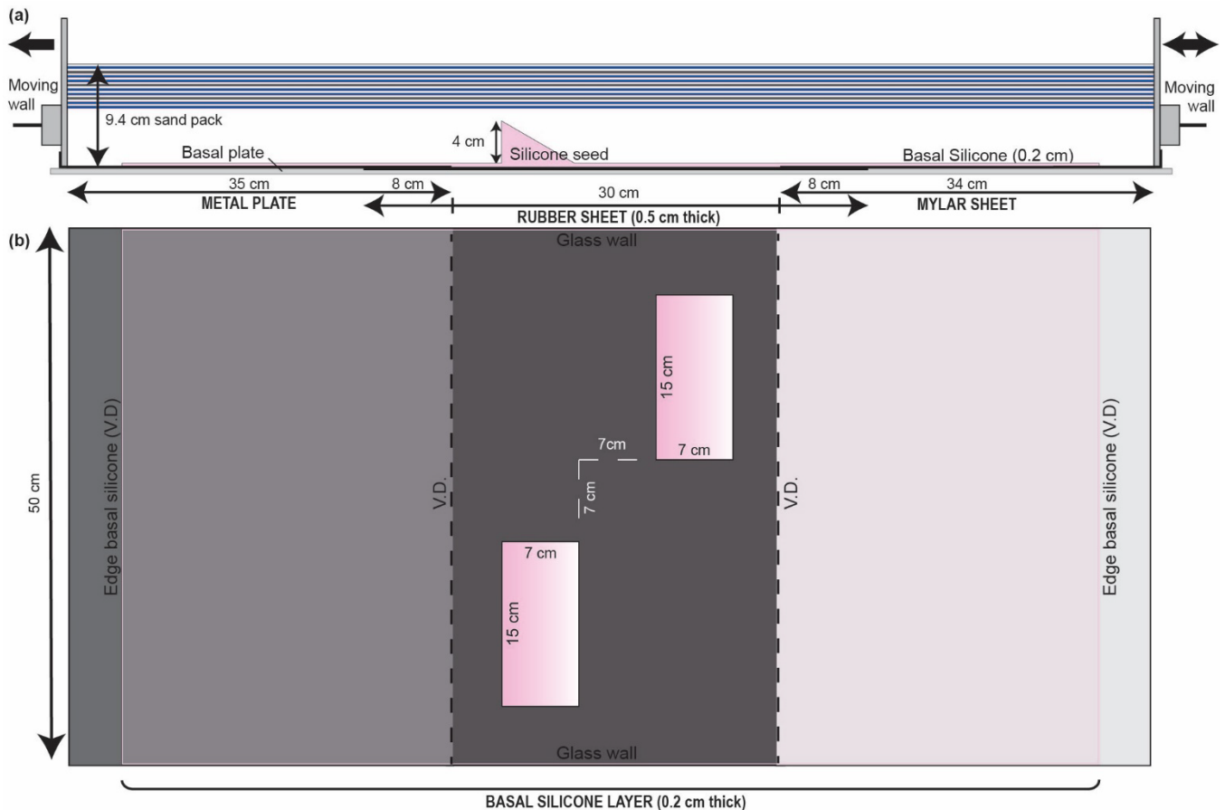
190 Figure 2. Experimental set-up. (a) Section view of model set-up through one of the silicone seeds illustrating the placement of the triangular prism within the basement sand pack on top of the basal set-up. (b) The plan view figure illustrates the organization of the basal set-up materials. V.D. stands for velocity discontinuity; these discontinuities are present at the edges of the rubber sheet where it connects to the metal plate and mylar sheet. The basal silicone layer that covers the basal set-up is 0.2 cm thick and extends
