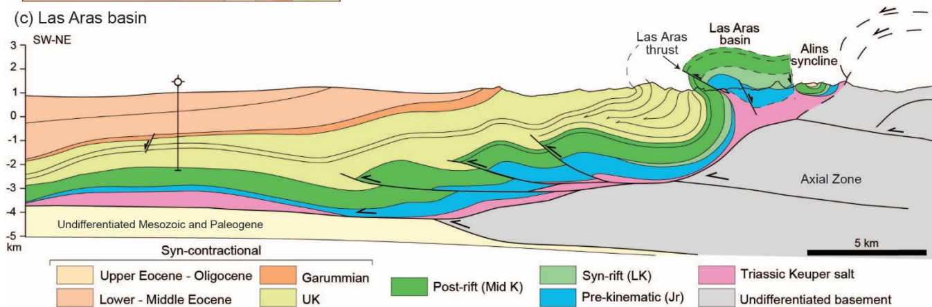
815 Figure 16. (a) Map showing the location of cross-sections through the San Juan and Las Aras basins, South-Central Pyrenees (compiled from Robador and Zamorano, 1999; García-Senz and Ramírez, 1997). (b) Cross-section through the San Juan basin. (c) Transect across the Las Aras basin (modified from Muñoz et al., 2018). Abbreviations: Jr: Jurassic; K: Cretaceous; L: Lower; U: Upper.
