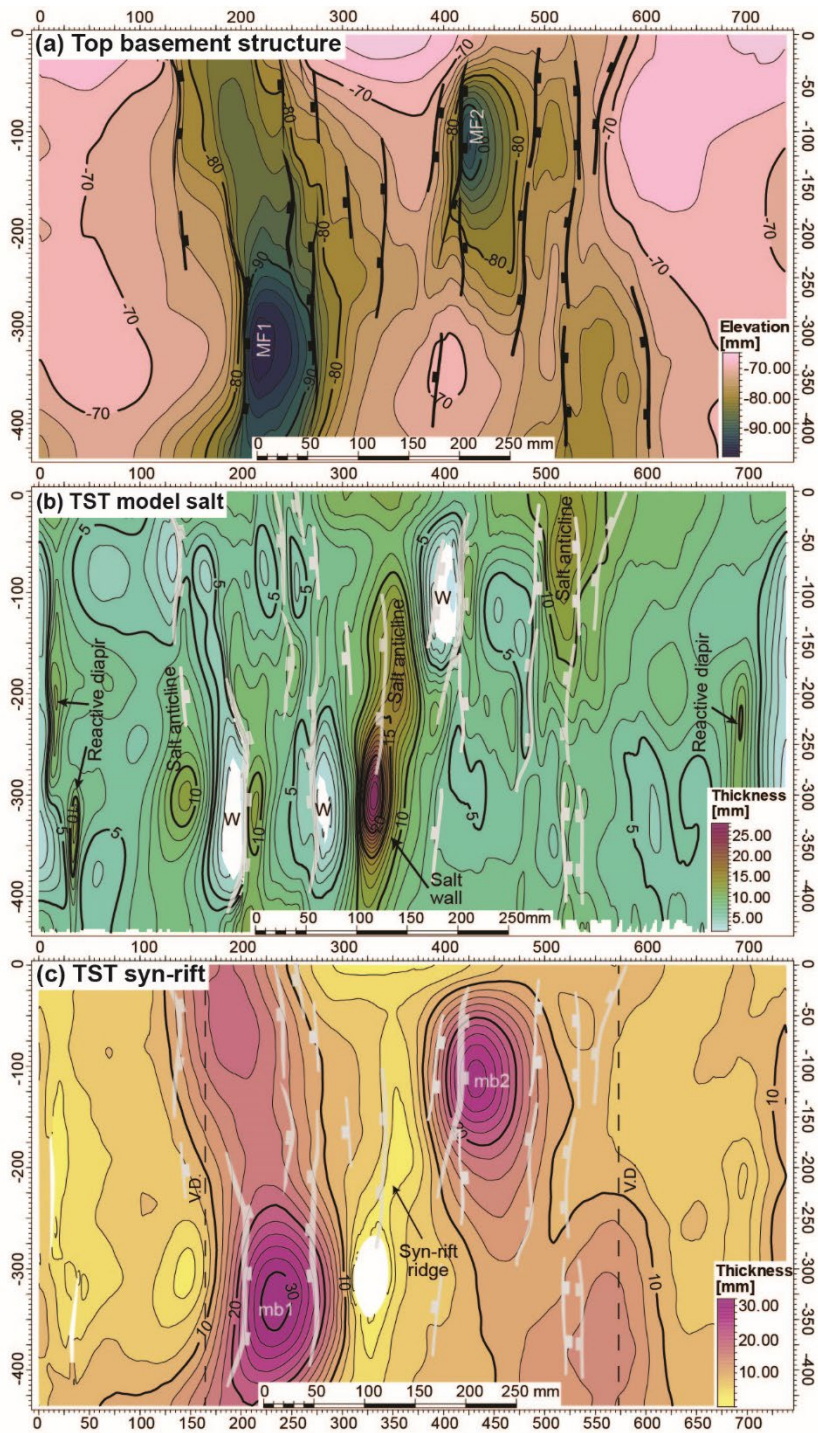
325 Figure 6. Structure and true stratigraphic thickness (TST) maps of key horizons from the voxel results of Model 1 (multistage rifting): (a) Top basement structure map, (b) TST autochthonous salt map, and (c) TST syn-rift map. Light gray lines in figures b
