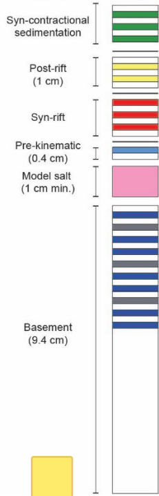
Figure 3. Experimental tectonostratigraphic units and final distribution through each model. (a) Schematic stratigraphic column of the tectonostratigraphic sand packages and their representative colors. (b) Representative cross section through Model 1 showing the distribution of the individual sand packages after the deposition of the post-rift succession. (c) Representative cross section through Model 2 showing the distribution of layers at the end of shortening. (d) Representative cross section through Model 3 at the end of shortening with the addition of syn-contractional sedimentation.
