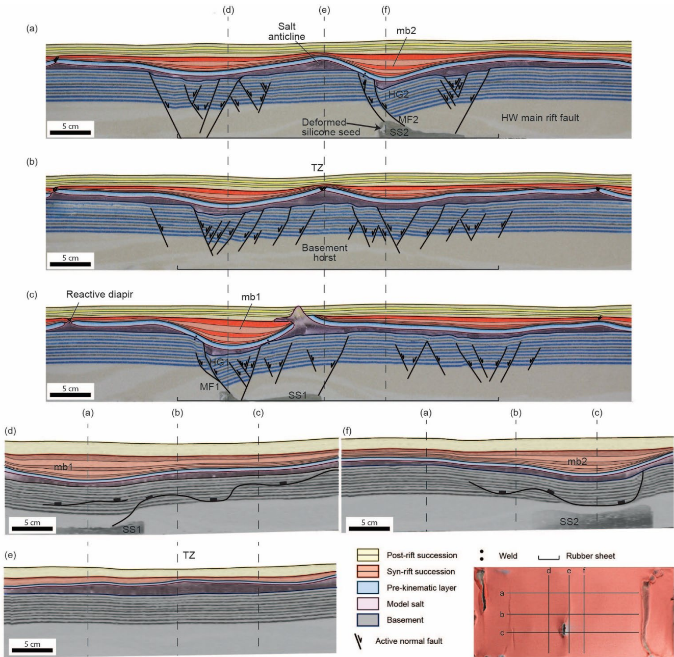
Figure 4. Interpreted representative cross-sections (a-c), and virtual inlines (d-f) through the central minibasins (mb1 and mb2) and the basement transfer zone of Model 1. The top view image shows section locations. Abbreviations: HG – half graben; HW – hanging wall; mb – minibasin; MF – Master Fault; SS – silicone seed; TZ – transfer zone.
