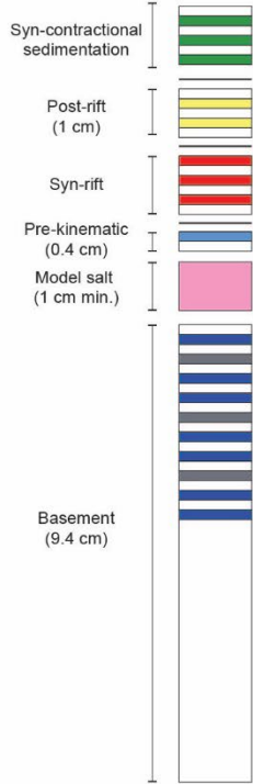
180 Figure 3. Experimental tectonostratigraphic units and final distribution through each model. (a) Schematic stratigraphic column of the tectonostratigraphic sand packages and their representative colors. (b) Representative cross section through Model 1 showing the distribution of the individual sand packages after the deposition of the post-rift succession. (c) Representative cross section through Model 2 showing the distribution of layers at the end of shortening. (d) Representative cross section through Model 3 at the end of shortening with the addition of syn-contractual sedimentation.
