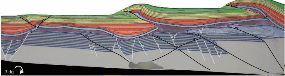
180 Figure 3. Experimental tectonostratigraphic units and final distribution through each model. (a) Schematic stratigraphic column of the tectonostratigraphic sand packages and their representative colors. (b) Representative cross section through Model 1 showing the distribution of the individual sand packages after the deposition of the post-rift succession. (c) Representative cross section through Model 2 showing the distribution of layers at the end of shortening. (d) Representative cross section through Model 3 at the end of shortening with the addition of syn-contractual sedimentation.
