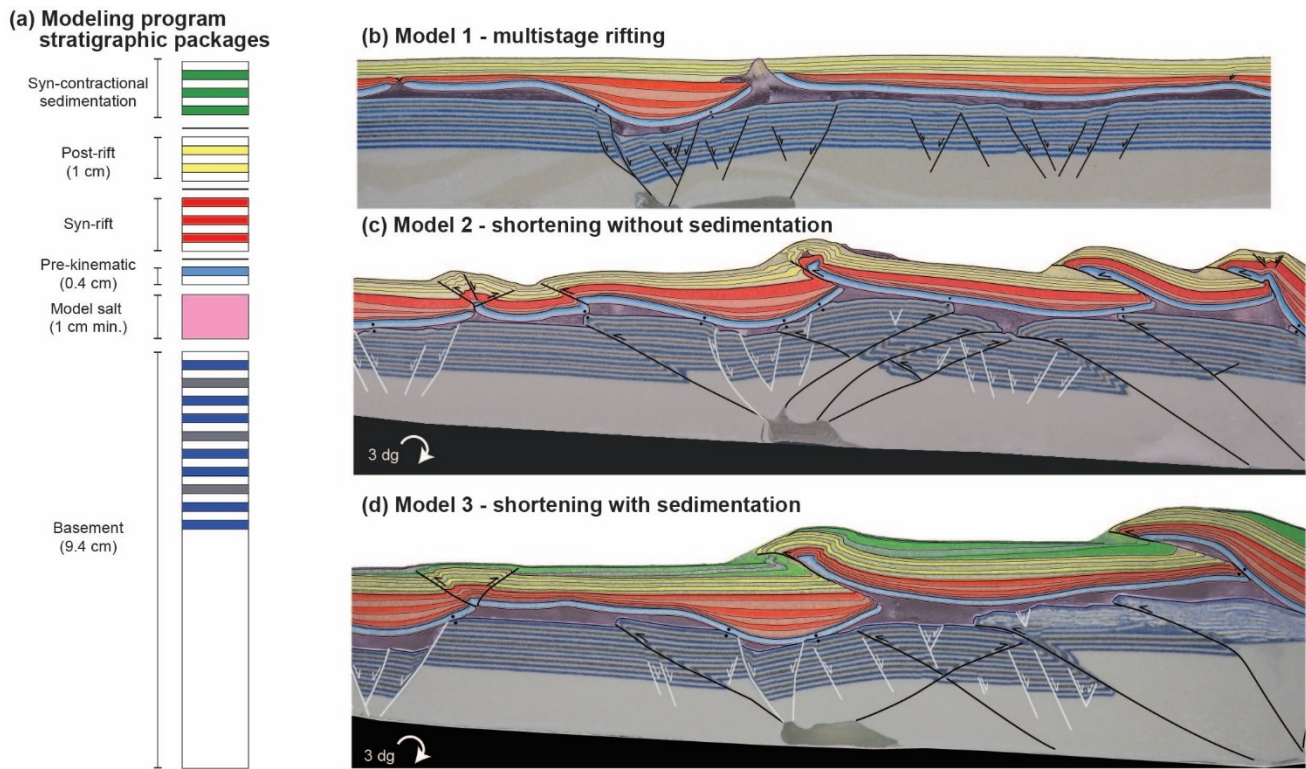
185 Figure 3. Experimental tectonostratigraphic units and final distributions through each model. (a) Schematic stratigraphic column of the tectonostratigraphic sand packages and their representative colors. (b) Representative cross section through Model 1 showing the distribution of the individual sand packages of the syn-rift and post-rift succession (see Fig. 4c). (c) Representative cross section through Model 2 showing the distribution of layers at the end of shortening (see Fig. 7c). (d) Representative cross section through Model 3 at the end of shortening with the addition of syn-contractual sedimentation (see Fig. 10c).
