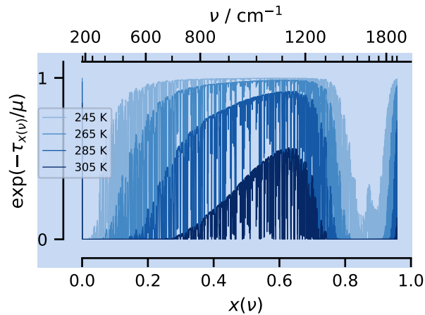
Figure 3. Spectral transmissivity plotted versus the cumulative black-body emission sensitivity, x = (4\sigma T^3)^{-1} \int_0^\nu \left( \frac{dB_\nu}{dT} \right) d\nu . The corresponding wavenumbers are indicated along the upper scale. Line colors darken with T_{\text{sfc}} with W = W_{\mathcal{R}}(T_{\text{sfc}}) .
