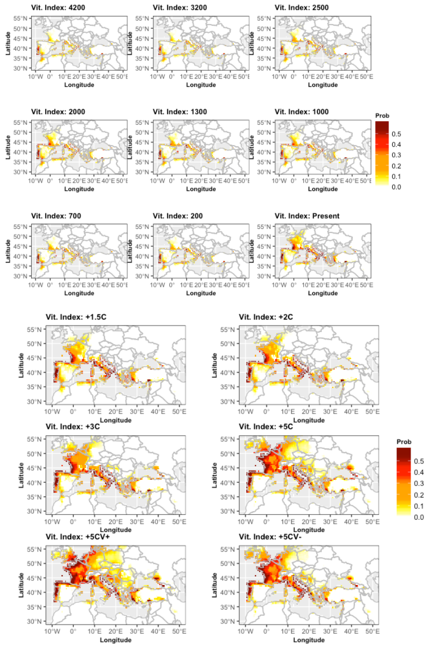
560 Figure 12. Distribution of the viticulture index (Vit. Index) for several time slices of the past (in yr BP) and future scenarios (expressed as anomalies of global temperature vs pre-industrial reference). The index is labelled VI and is explained in eq.4. White areas indicate where it is impossible to cultivate vine.
