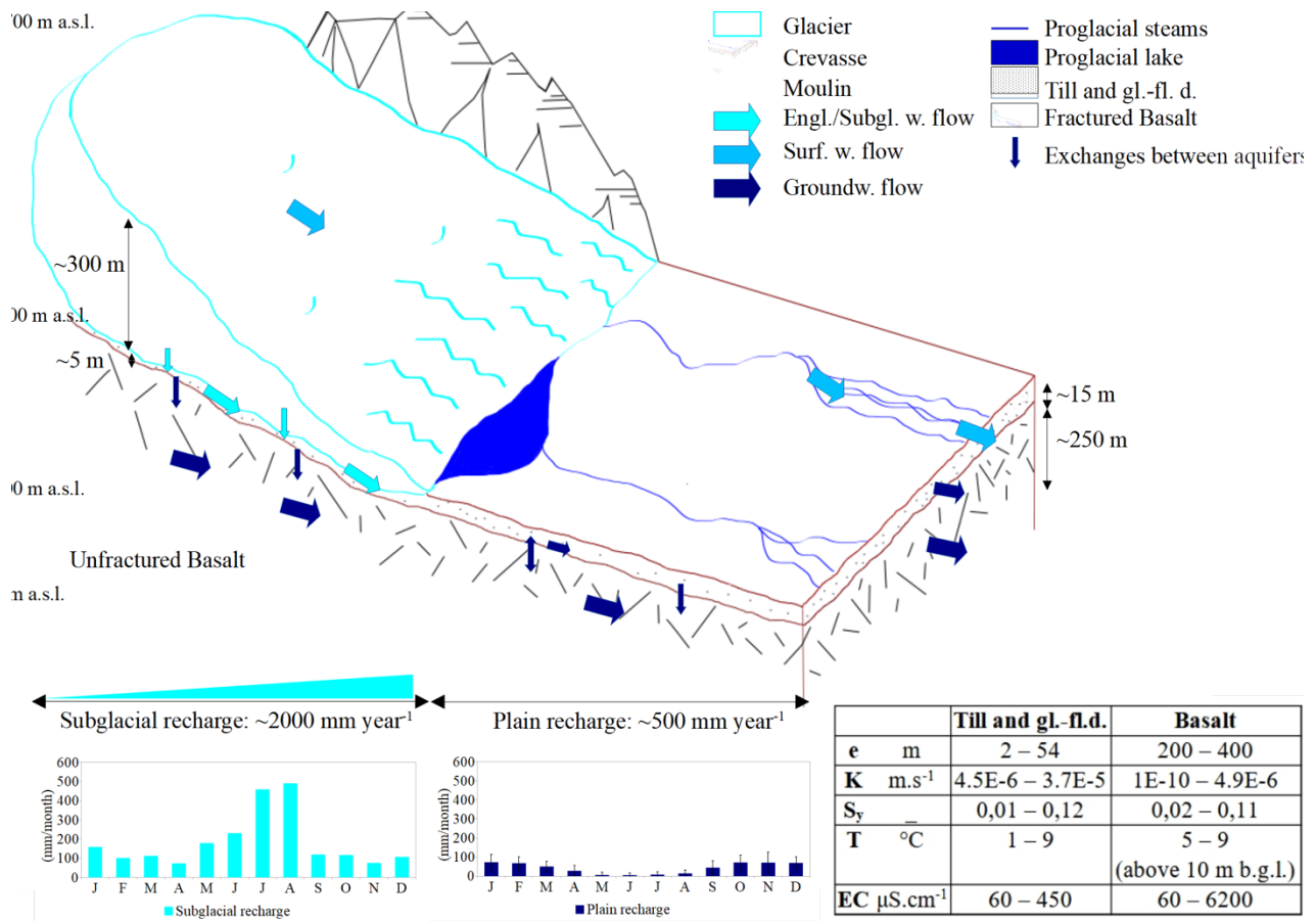
535 Figure 13: Conceptual model of the groundwater dynamic in glacierized catchments such as those observed at Fláajökull, Heinabergsjökull and Skálafellsjökull. The model is based on all the data presented in this paper. A glacier is at the head of the catchment along with the two geological formations underlying it and in its front: The till and glacio-fluvial deposits and the basalt formation. Average characteristics of the hydrogeological formations are described along with their spatial (e, K, S y ) and seasonal (T, EC) variability as well as recharge rates (subglacial and on the proglacial area) along with their monthly variability. The groundwater dynamic is expressed by arrows. Subgl.: subglacial; w.: water; surf.: surface; groundw.: groundwater; gl.fl. d.: glacio-fluvial deposits. 540
