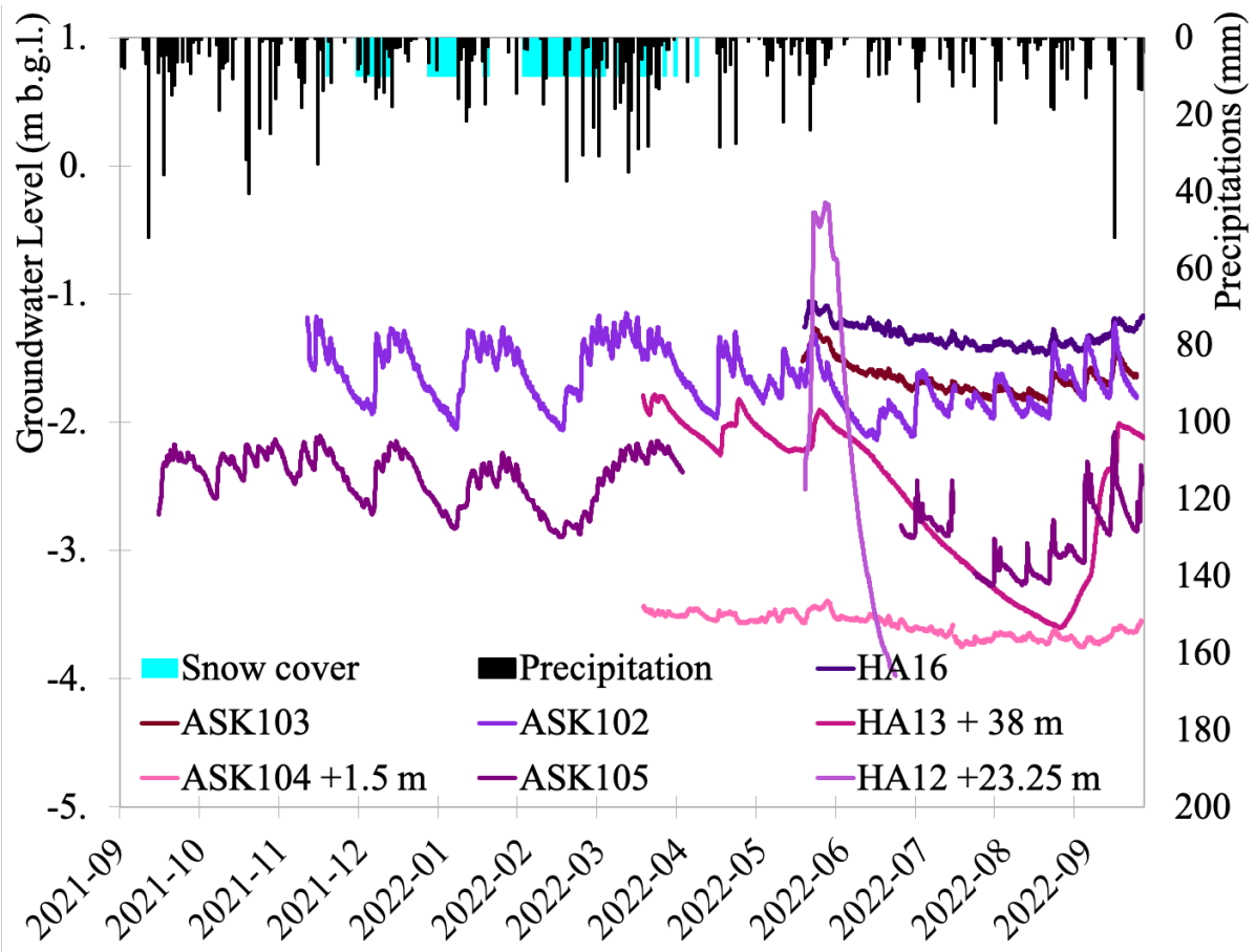
Figure 8: Hourly evolution of the groundwater level (in m b.g.l.) in the basalt aquifer, from September 2021 to September 2022 (5 boreholes: ASK102, ASK103, ASK104, ASK105, HA16), daily precipitation (in mm) from Höfn weather station 705, and days with snow cover.
