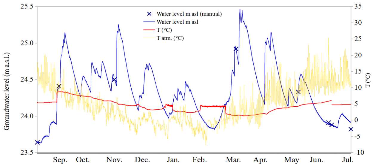
485 Figure 12: Hourly groundwater level (in blue, m a.s.l.) and temperature (in red) in the borehole FLA4, and atmospheric temperature (in yellow, from the Baro Diver probe in borehole FLA4). The temperature chronicle exhibits plateaus around 5 °C at the end of August 2021, in January, February, and July 2022, each time the groundwater level is lower than 24.1 m a.s.l.
