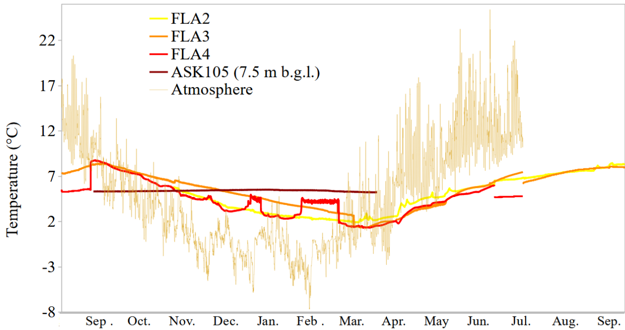
Figure 9: Hourly temperature records from August 2021 to September 2022: in the till and glacio-fluvial deposits aquifer in 3 boreholes (FLA2, FLA3, FLA4), in the basalt aquifer in 1 borehole (ASK105 at -7.5 m b.g.l.), and in the atmosphere (recorded by a Baro Diver at the top of FLA4).
