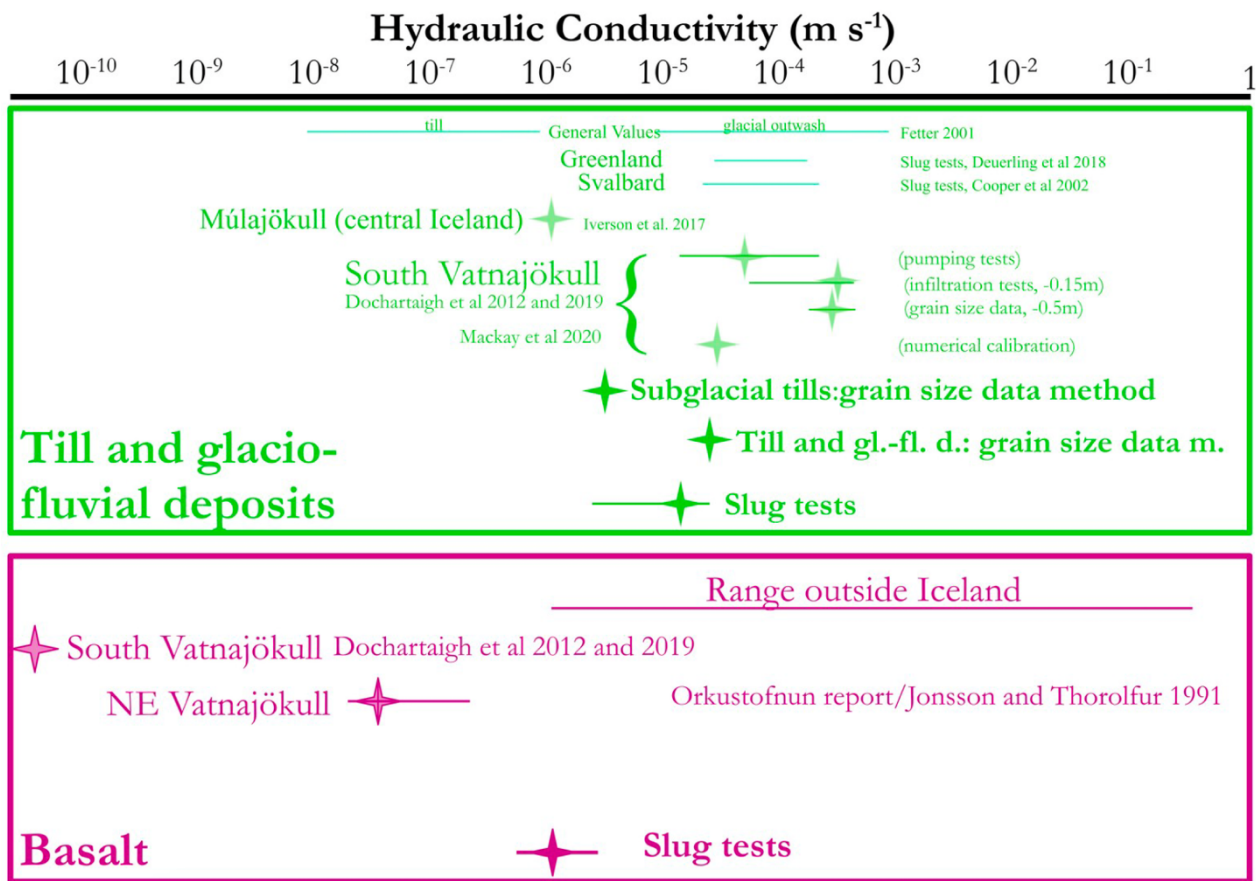
435 Figure 11: Hydraulic conductivity values for the till and glacio-fluvial deposits and the basalt from data analysis and the literature; stars indicate single or average value and horizontal lines the range of values. The range for hydraulic conductivities of basalt outside Iceland is based on several bibliographical references, details and references in the text.
