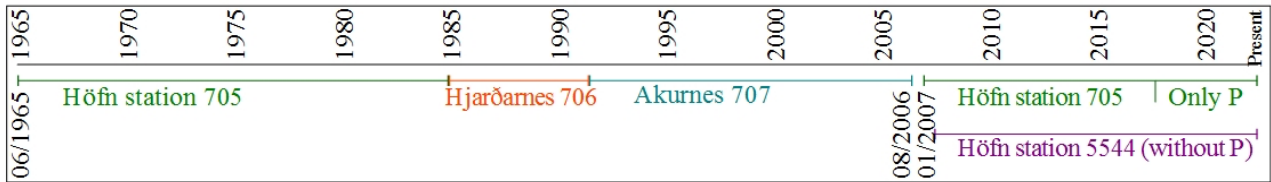
Figure 2: Time periods of the T and P records of the 4 Höfn weather stations: Höfn 705 (+4 m a.s.l.), Höfn 5544 (+5 m a.s.l.), Hjarðarnes 706 (+9 m a.s.l.) and Akurnes 707 (+17 m a.s.l.). The location of the four stations is shown with red plus symbols in fig. 3.
