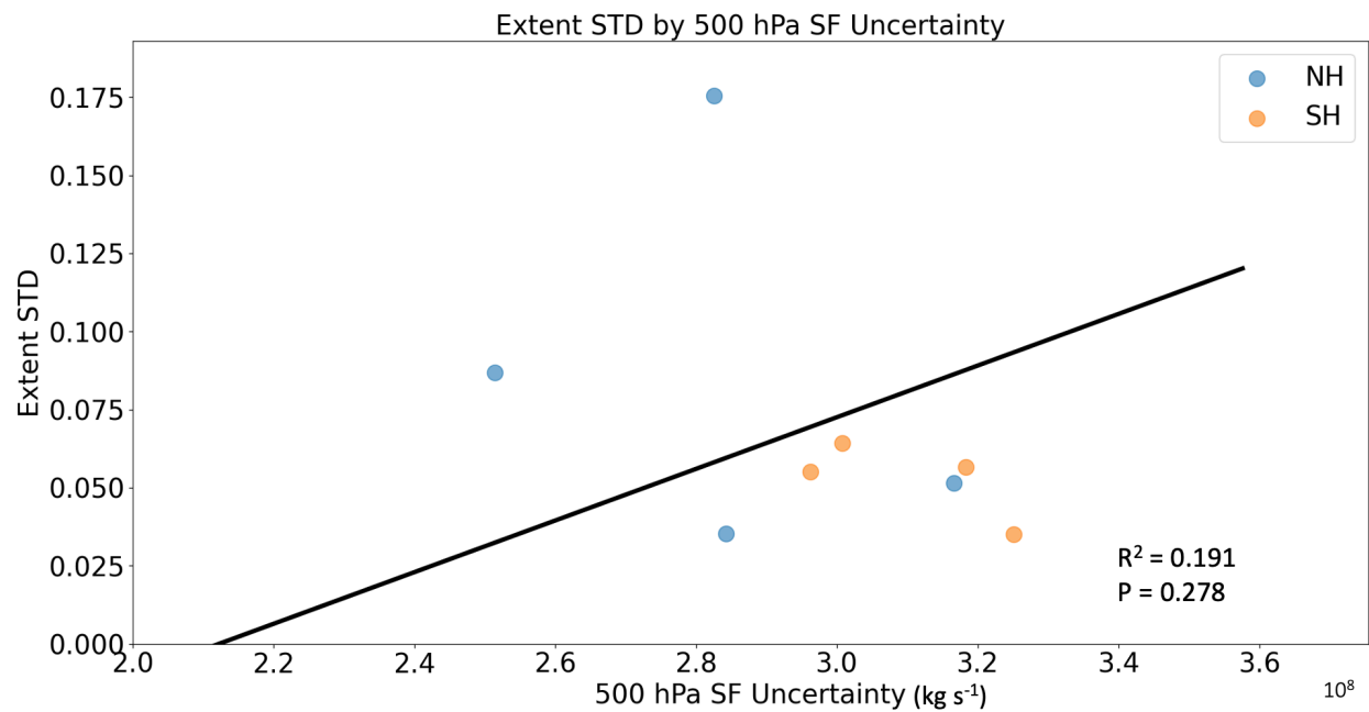
65 Fig S3: Climatological mean SF extent STD (degrees latitude) by 500 hPa SF uncertainty ( \text{kg s}^{-1} ) near the tropical edge, showing no significant relationship.
