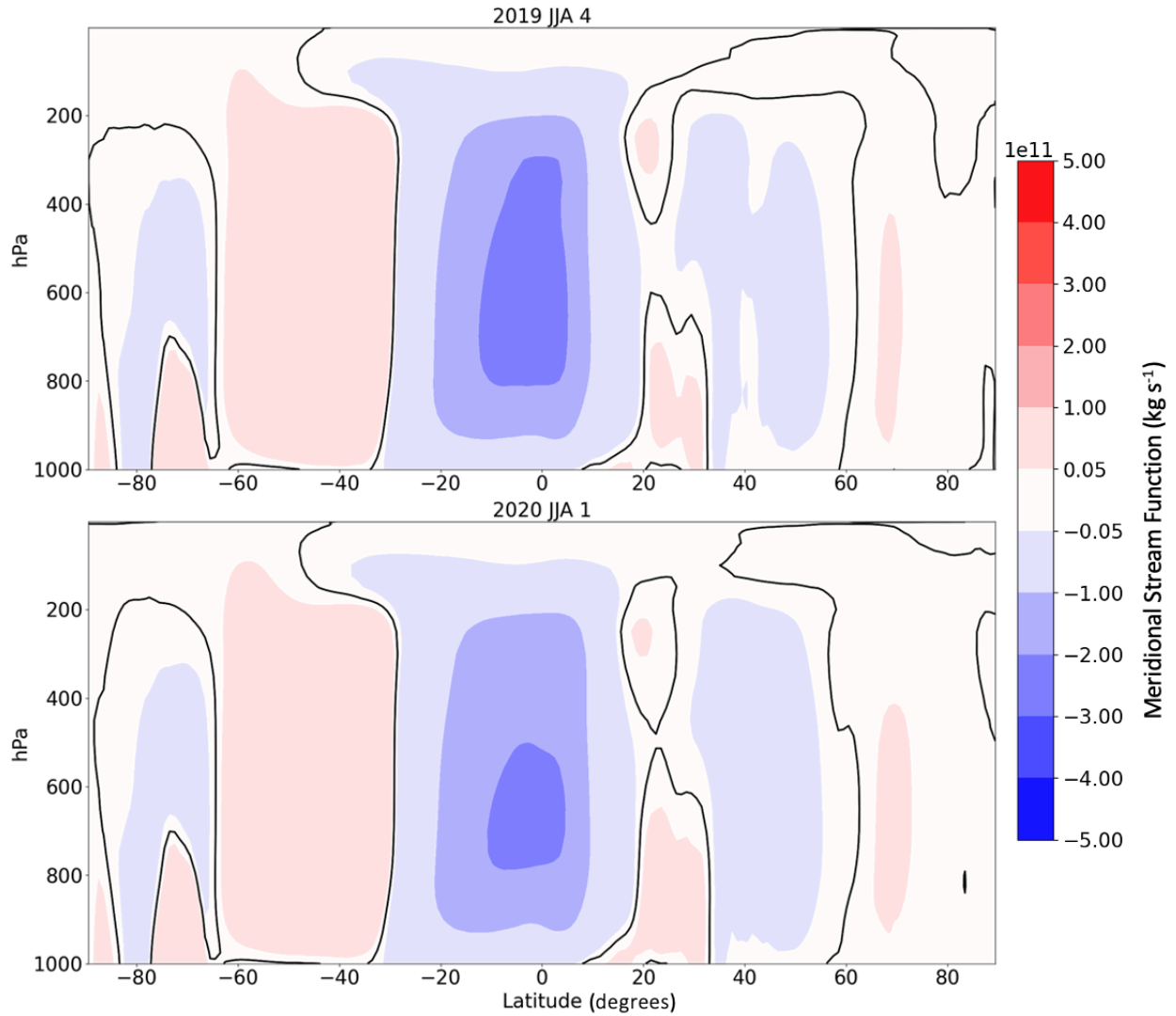
Figure S2: SF values ( \text{kg s}^{-1} ) for ensemble member 4 in JJA 2019, and ensemble member 1 in JJA 2020, showing an unenclosed NH HC. The black contours indicate the zero-crossing, while shading signifies SF intensity. Note the region near 500 hPa and 20 degrees in both years where there is no positive circulation.
