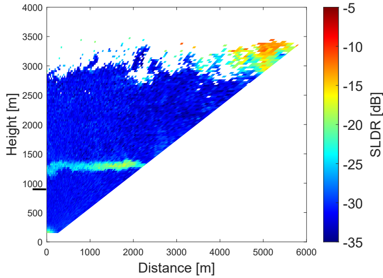
Figure 8. RHI scan of SLDR observed on 13 February 2017, at 13:31 UTC in Limassol from 90^\circ to 150^\circ elevation angle. The black horizontal line on the y axis mark the height of the layer analysed in Figure 9.
