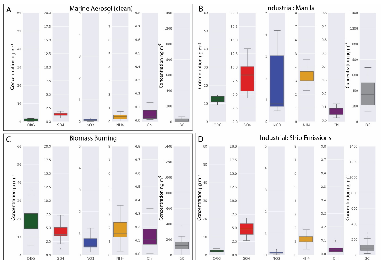
300 Figure 5: Chemical mass signatures of aerosol from boundary layer passes through (A) clean marine environment over the West Pacific Ocean east of the Philippines (01:25:28 - 01:35:28 UTC October 2019), (B) Manila industrial region (00:31:21 - 00:41:21 UTC 04 October 2019), (C) a biomass burning plume over the Sulu Sea (00:47:10 - 00:57:10 UTC 16 October 2019), (D) a pass through the R/V Sally Ride ship plume northeast of Luzon (04:03:42 - 04:13:42 UTC 2 October 2019).
