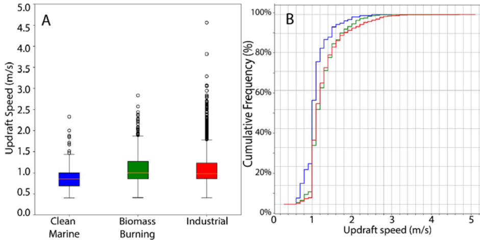
Figure 10: (A) The distribution of the updraft speeds measured at cloud base using data from the Turbulent Air Motion Measurement System (TAMMS) for the three aerosol types discussed in section 4. The median (orange line), the 25 th and 75 th percentile (colored boxes) the 5 th and 95 th percentile (black whiskers), and outliers (circles) are shown. (B) Cumulative frequency diagram of updrafts for the three aerosol types.
