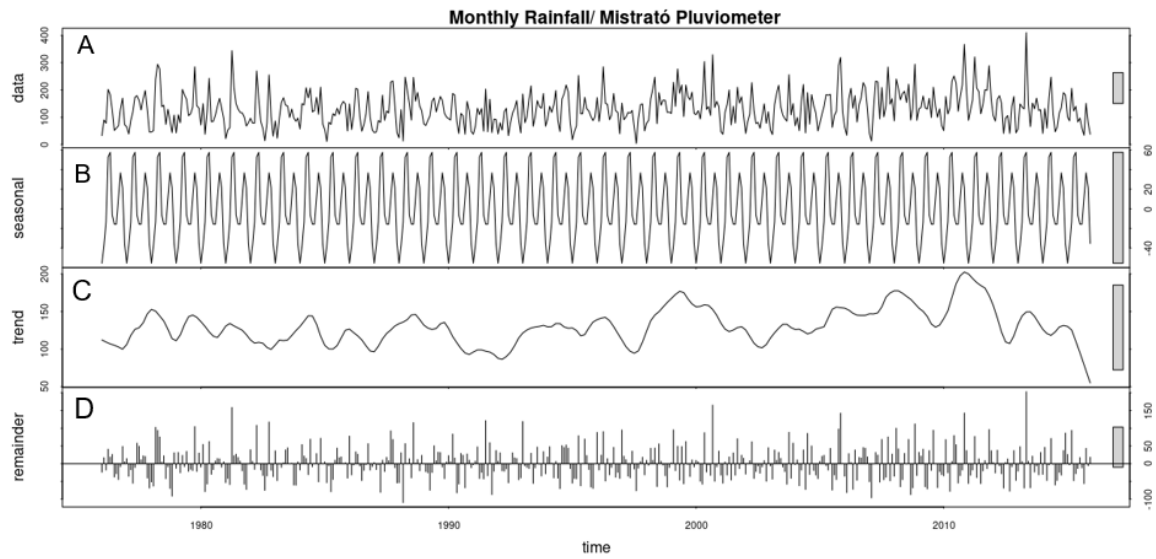
Figure S1. STL decomposition of monthly rainfall (1976-2015) for Mistrató station. (A) Monthly series (mm/month), (B) Seasonal component, (C) Trend component, (D) Remainder component (stochastic) (E-H).
