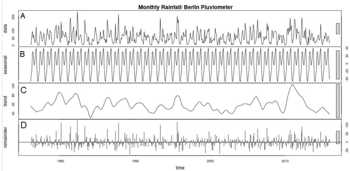
Figure S2. STL decomposition of monthly rainfall (1976-2015) for Berlin station: (A) Monthly series (mm/month), and (B-D) seasonal, trend component, and remainder components (stochastic), respectively.
