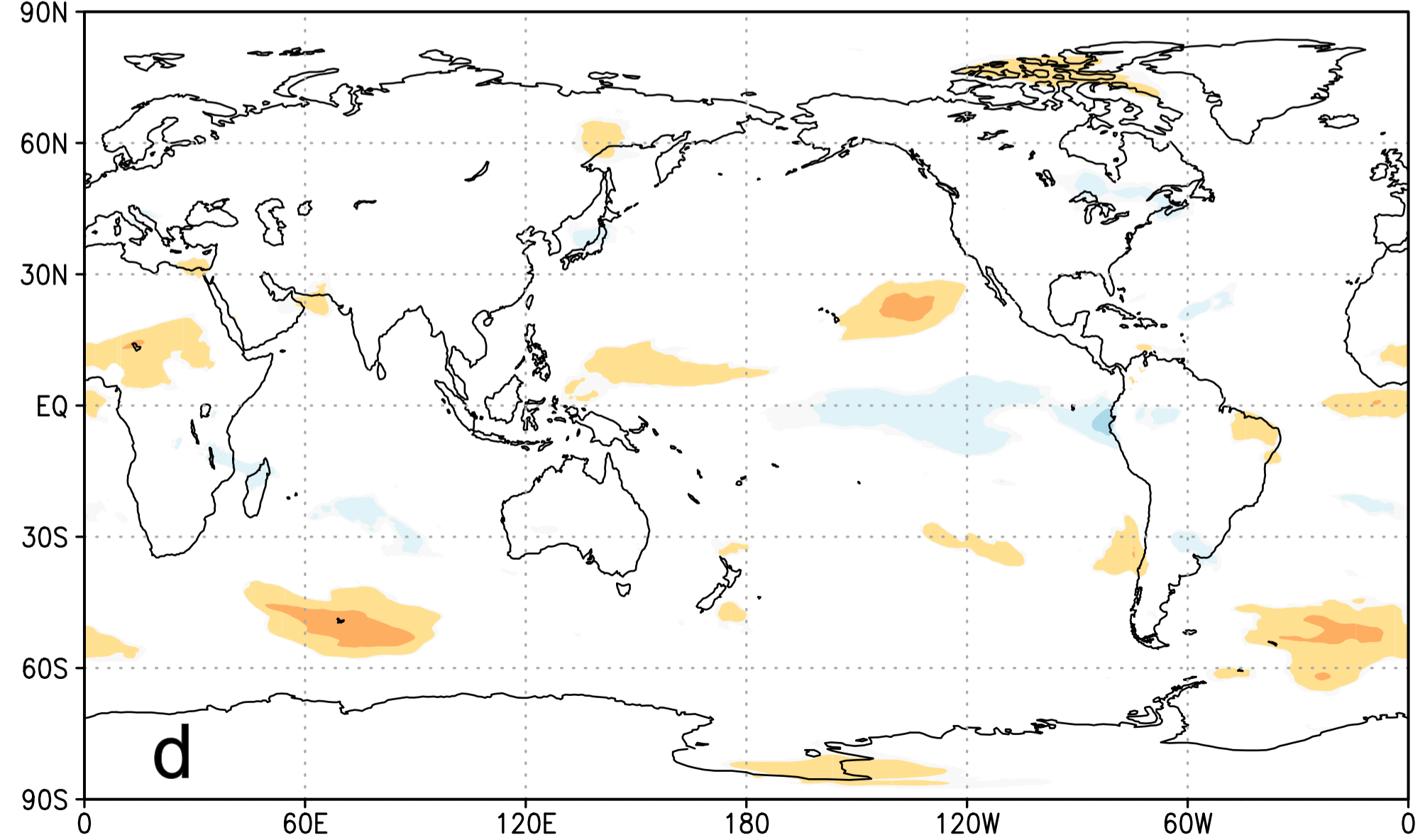
corr Dec–Feb monthly Berlin precipitation anomalies with Dec–Feb monthly ERA5 column vapour anomalies 1976:2015 p < 5\%
