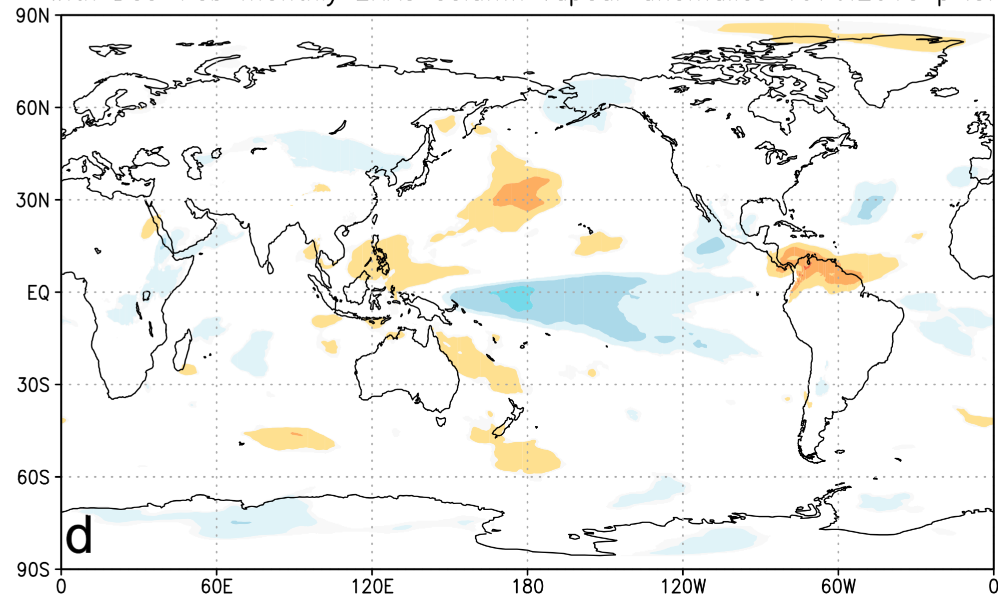
corr Dec–Feb monthly Mistrato precipitation anomalies with Dec–Feb monthly ERA5 column vapour anomalies 1976:2015 p < 5\%
