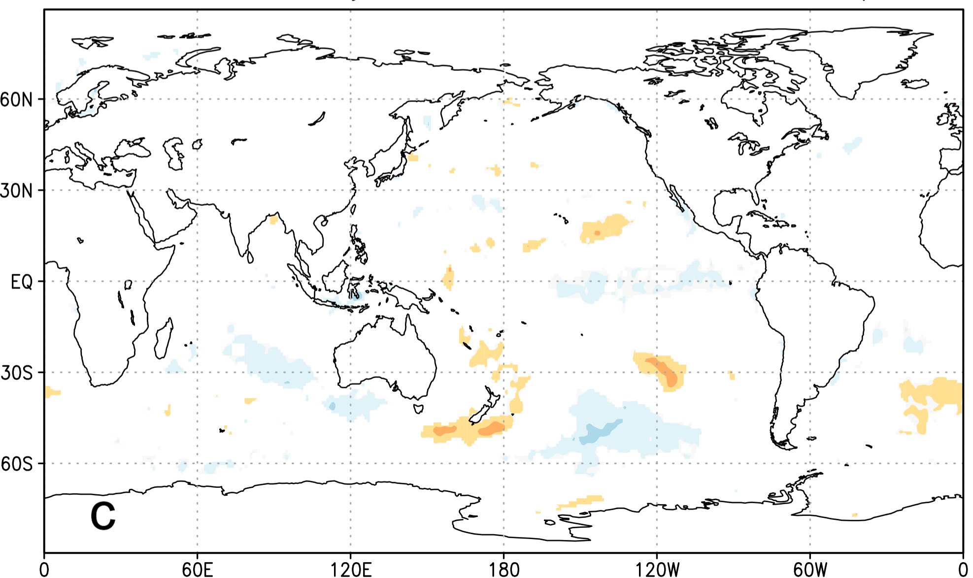
corr Dec–Feb monthly Berlin precipitation anomalies with Dec–Feb monthly HadISST1 SST anomalies 1976:2015 p < 5\%
