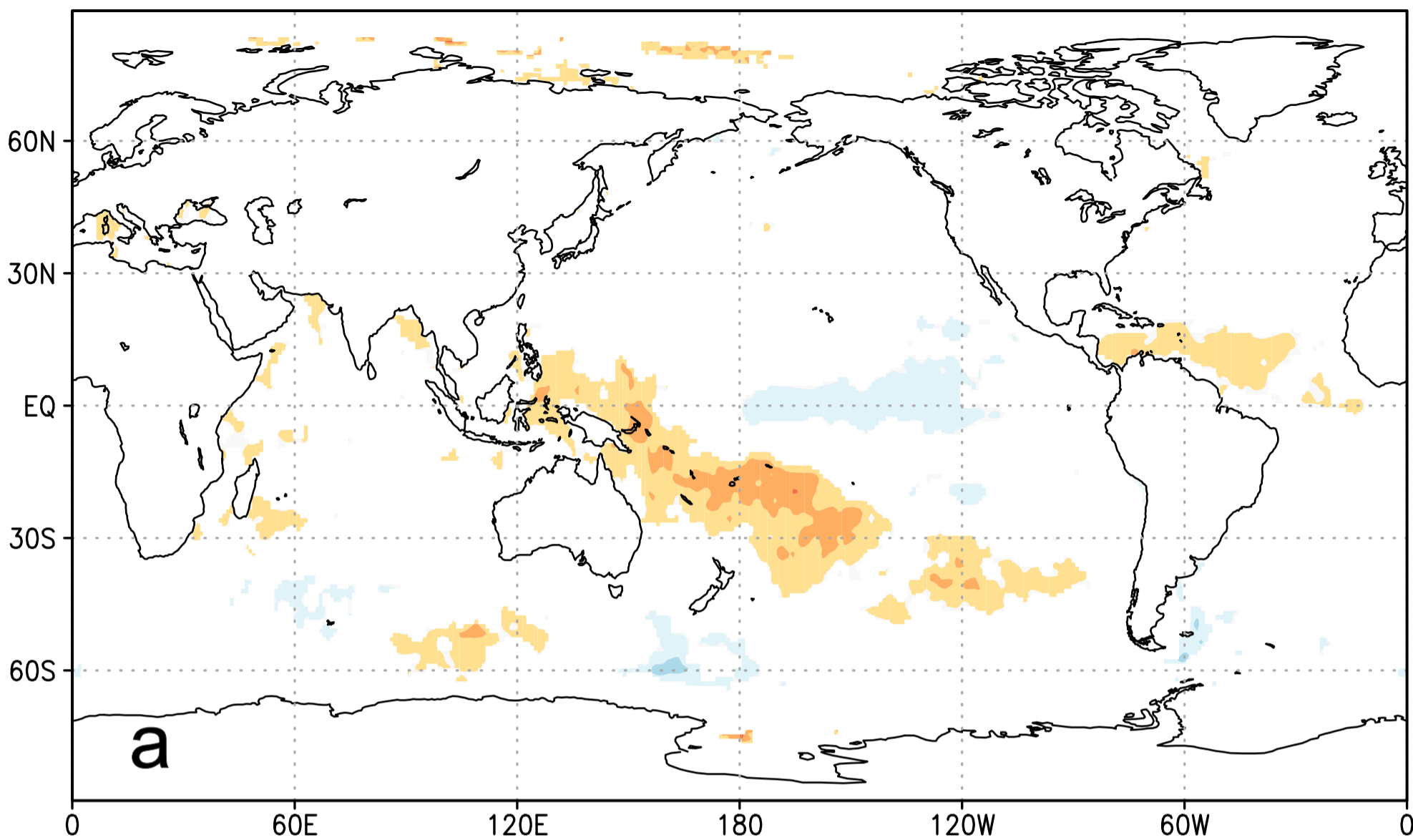
corr Jun–Aug monthly Berlin precipitation anomalies with Jun–Aug monthly HadISST1 SST anomalies 1976:2015 p < 5\%
