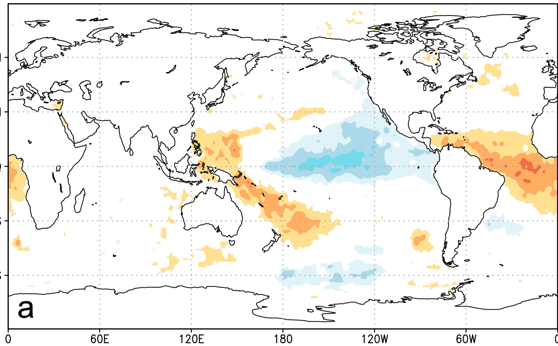
corr Jun–Aug monthly Mistrato precipitation anomalies with Jun–Aug monthly HadISST1 SST anomalies 1976:2015 p < 5\%
