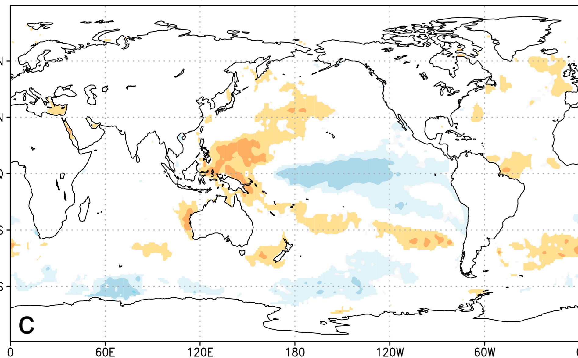
corr Dec–Feb monthly Mistrato precipitation anomalies with Dec–Feb monthly HadISST1 SST anomalies 1976:2015 p < 5\%
