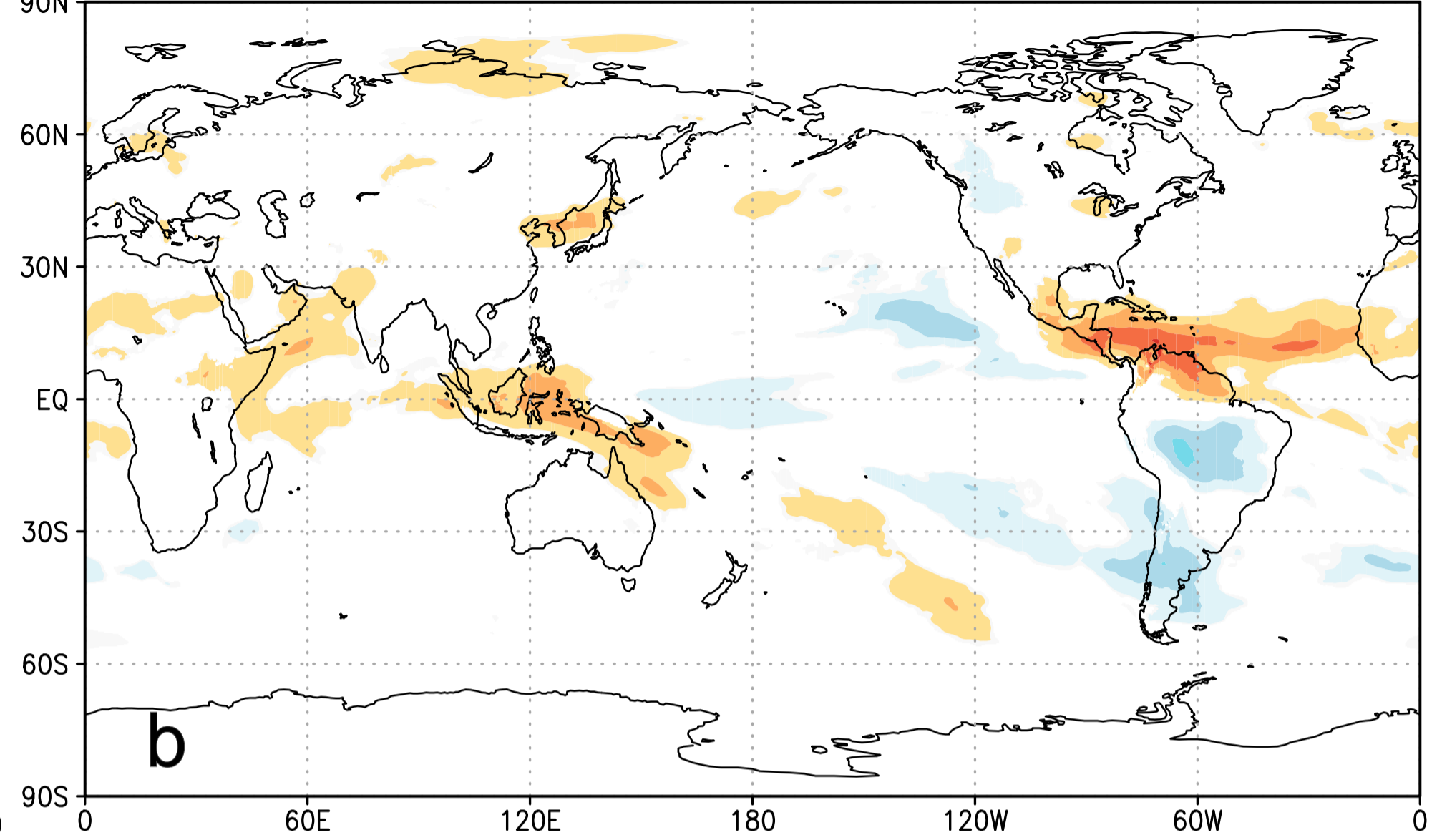
corr Jun–Aug monthly Berlin precipitation anomalies with Jun–Aug monthly ERA5 column vapour anomalies 1976:2015 p < 5\%
