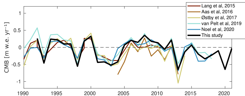
Figure 12. Time series of yearly emb CMB from different model studies from 1990-2021.
