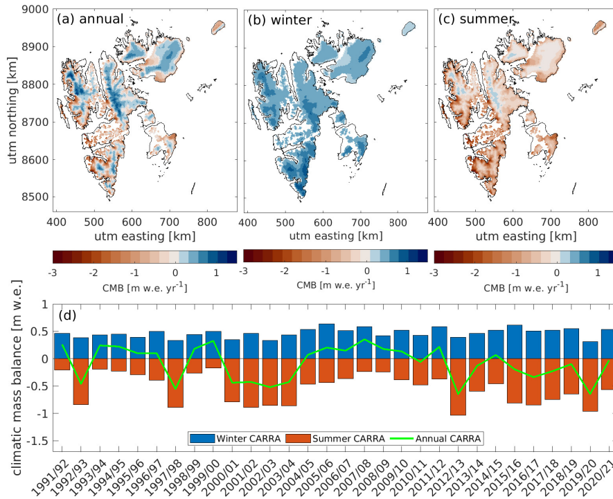
Figure 6. Climatic mass balance of Svalbard from 1991/92 to 2020/21. The top row contains maps of the average (a) annual, (b) winter, and (c) summer \text{emb-CMB} , while (d) shows the temporal evolution of the summer, winter and annual \text{emb-CMB} for each mass balance year (September - August). Dark-red and blue show the results using CARRA forcing, while lighter-colored bars show the results using AROME-ARCTIC (denoted AA).
