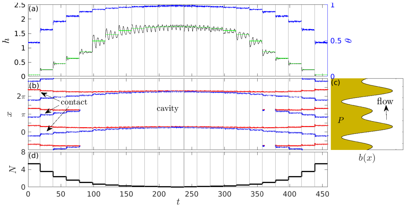
Figure 5. Using the same plotting scheme as in figure 3, dynamic cavity evolution under step changes in N with a fully permeable bed, P = (0, a) .
