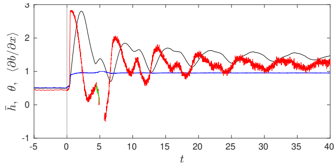
Figure 9. Cavity height \bar{h} (black), cavitation ratio \theta (blue) and mean contact angle \langle \partial b / \partial x \rangle (red and green) corresponding to a step change from N = 1.02 to N = 0.47 at t = 0 (for \bar{h} and \theta , these are the blue curves in figure 7, plotted for a longer time interval). For each contact area (c_j, b_{j+1}) , I compute the mean contact angle as \langle \partial b / \partial x \rangle = (b_{j+1} - c_j)^{-1} \int_{c_j}^{b_{j+1}} \partial b / \partial x dx = (b(b_{j+1}) - b(c_j)) / (b_{j+1} - c_j) . Note that there is an interval from t = 4.94 to t = 5.69 during which the code detects no contact area (a sufficiently deep water layer is present everywhere) and there are two contact areas between t = 4.43 and t = 4.88 .
