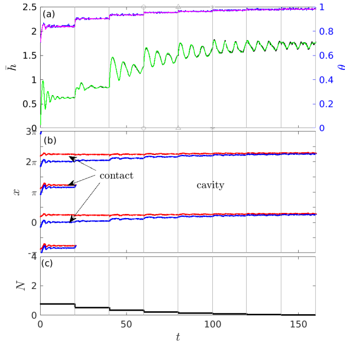
Figure 6. Using the same plotting scheme as in figure 3, dynamic cavity evolution under step changes in N with a fully permeable bed, P = (0, a) , using a smaller initial value of N than in figure 5. In each panel the solution for the same mesh as used in figure 5 and all remaining figures is shown in black/blue in panel a and blue/red in panel b. The solution for a mesh with twice the resolution at the bed is shown in magenta/green in panel a and black in panel b.
