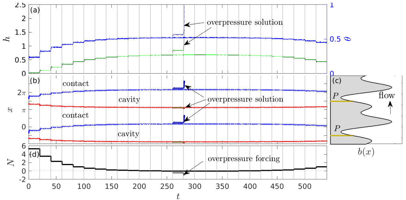
Figure 10. Using the same plotting scheme as in figure 3, dynamic cavity evolution under step changes in N with a permeable bed on the downstream side of the smaller bed protrusion, with P = \{4.64\} . The solution indicated by arrows corresponds to negative forcing effective pressure N , and departs at t = 260 from the solution not indicated by arrows.
