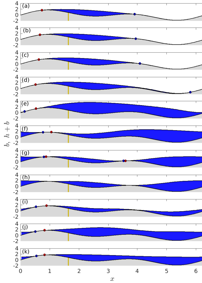
Figure 8. Cavity shapes for a step change from N = 1.02 to N = 0.47 (the blue curves in figure 7) at (a) t = 0 , (b) t = 10^{-3} , (c) t = .32 , (d) t = .49 , (e) t = 1.35 , (f) t = 3.39 , (g) t = 4.62 , (h) t = 5.16 , (i) t = 6.61 , (j) t = 8.70 and (k) t = 120 . Red dots correspond to upstream cavity endpoints, blue dots to downstream endpoints.
