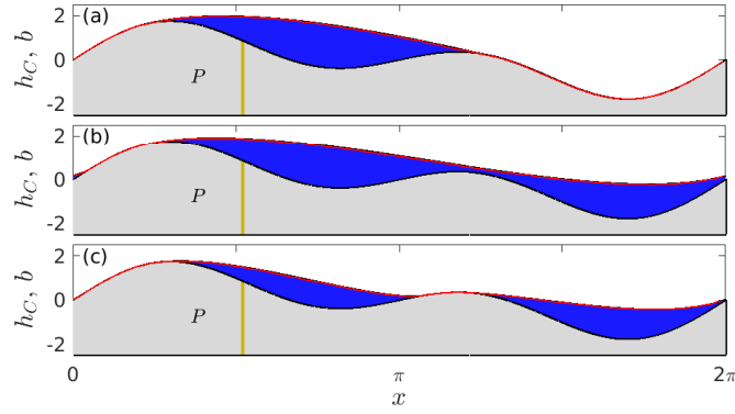
Figure 2. Comparison of steady cavity roof geometry (denoted by b + h for the dynamic model, h_C for the steady viscous model of part 1) for x_P = 1.64 . The bed is shown in grey, with the permeable bed portion P in beige. The result for the dynamic model is shown as a blue shaded cavity, the result of the steady state model of part 1 as a red curve. a) N = 1.053 before cavity expansion, b) N = 1.053 after cavity expansion and c) N = 2.37 , with an isolated cavity volume of V_2 = 1.87 imposed in the model of part 1, the volume having been computed from the dynamic solution. Note that this cavity volume is different from the value of V_2 = 1.062 for the isolated cavities that form under quasi-steady conditions for the same bed in part 1. The two cavity roof shapes are practically indistinguishable in each case.
