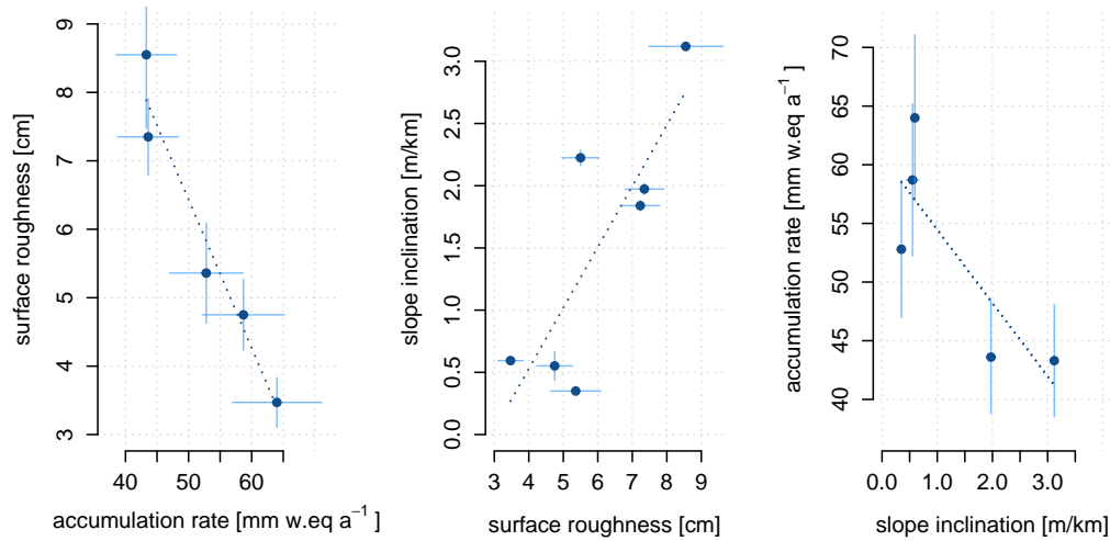
Figure D1. Comparisons between accumulation rate A [mm w.e. \text{a}^{-1} ], surface roughness SD_{SH} [cm], and slope inclination [ \text{m km}^{-1} ]. Linear regression lines (dashed) suggest possible relationships. Vertical and horizontal lines represent 2 \times \text{SDs} of the according environmental property as an indication for uncertainty. Uncertainty of 10 km slope inclinations are very small such that they are not visible for most sites.
