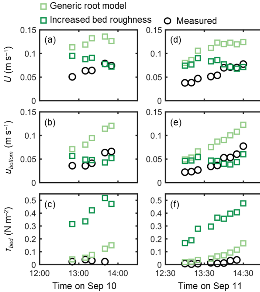
430 Figure 8. Time-series of measured and predicted (a, d) cross-sectional mean velocity ( U ), (b, e) (spatially averaged) velocity at z = 0.05 m, and (c, f) bed shear stress ( \tau_{bed} ) during the two-days measurement in Bakhawan Ecopark. The measured values are from Yoshikai et al. (2022a) and the predicted values are obtained through the COAWST employing the generic Xie root model and the increased bed roughness as an approximation of drag by mangroves, respectively.
