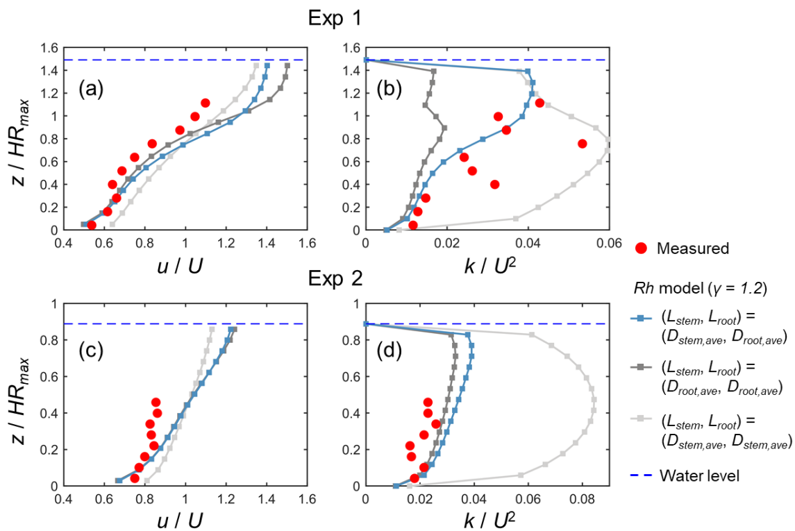
Figure R7. Comparison of the vertical profiles of (temporally and spatially averaged) velocity ( u ) and turbulent kinetic energy ( k ) normalized by the cross-sectional mean velocity ( U ) measured by Maza et al. (2017) and predicted by the COAWST using the Rh model with different length-scales of stem- and root-generated wakes ( L_{stem} and L_{root} , respectively) defined – blue markers: L_{stem} and L_{root} set to the stem diameter ( D_{stem,ave} ) and root diameter ( D_{root,ave} ), respectively; dark-gray markers: L_{stem} and L_{root} both set to D_{root,ave} ; light-gray markers: L_{stem} and L_{root} both set to D_{stem,ave} . The scale coefficient ( \gamma ) was set to 1.2 for all the cases.
