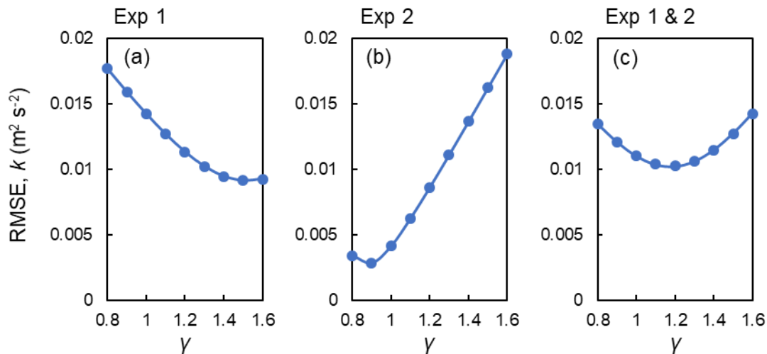
Figure R6. Root mean square error (RMSE) of modeled turbulent kinetic energy ( k ) against the measured data in (a) Exp 1, (b) Exp2, and (c) both Exp 1 and 2 of the flume experiment, by varying the value of scale coefficient ( \gamma ), for which the computation of the predicted value at the height of the measurement point was obtained by the interpolation of k computed at adjacent vertical layers.
